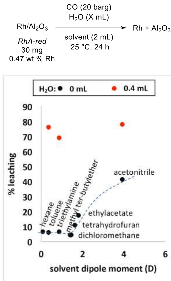
Fig. 1 | Leaching of RhA-red sample in different solvents.
