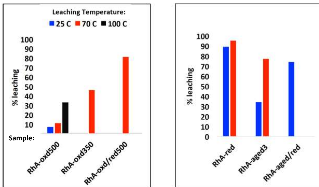
Fig. 4 | Effect of temperature on the leaching efficiency of samples pretreated under different conditions. Left: oxidized samples, right: reduced samples
