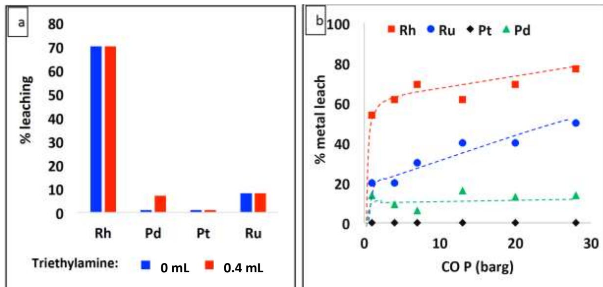
Fig. 7 | (a) Selective leaching of Rh in presence of Pd, Pt, and Ru with and without triethylamine at 20 barg CO and 25 °C. (b) Effect of CO pressure on leaching of Rh, Pd, Pt, and Ru from a mixture of the four metals in acetonitrile/water/triethylamine 5:1:1 v:v:v mixture at 70 °C.
