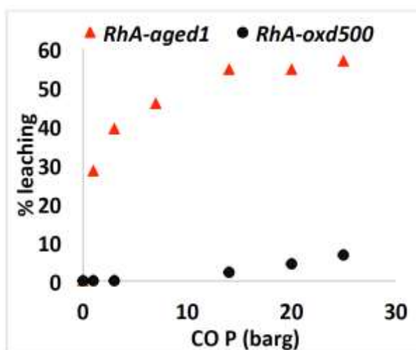
Fig. 3 | Effect of CO pressure on leaching of Rh from the pre-reduced and aged ( RhA-aged1 ) sample and the pre-oxidized ( RhA-oxd500 ) in acetonitrile/water/triethylamine solution after 24 h at 25 °C.
