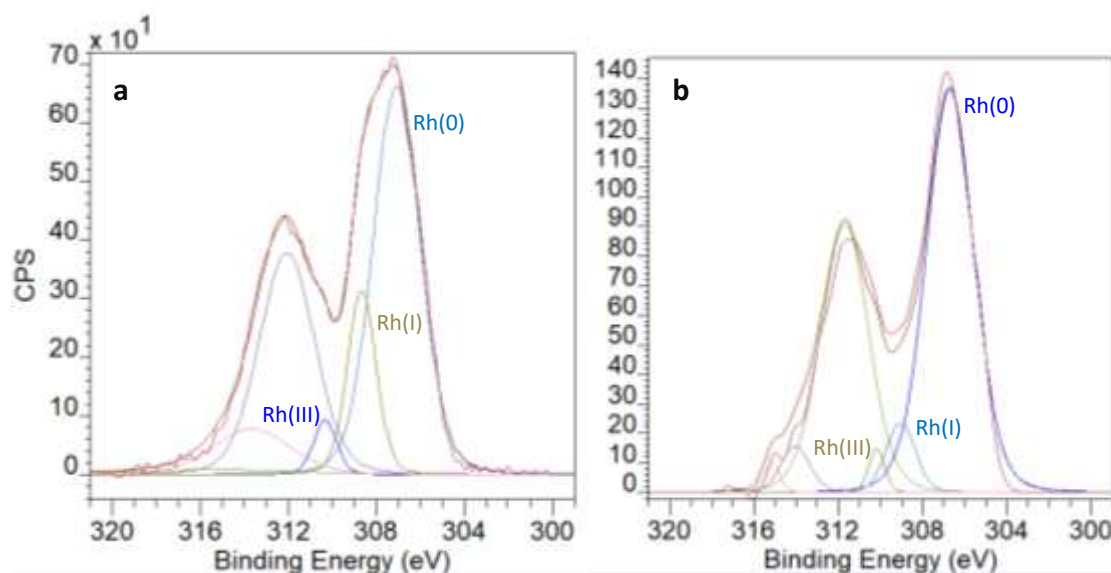
Fig. 6 | XPS Spectra of commercial Rh NP on alumina RhA-comm (oxidation state distribution from curve fitting) (a) before leaching: 74% Rh(0), 21% Rh(I), 5% Rh(III). (b) after leaching under standard conditions at 70 °C for 72 h followed by another 24 h at 25 °C: 88% Rh(0), 9% Rh(I), 3% Rh(III).
