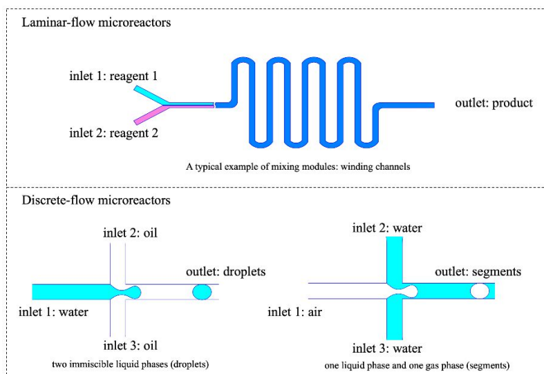
Figure 1. Pressure-driven microreactors categorized into two main groups: continuous laminar-flow and discrete segmented-flow microreactors.
