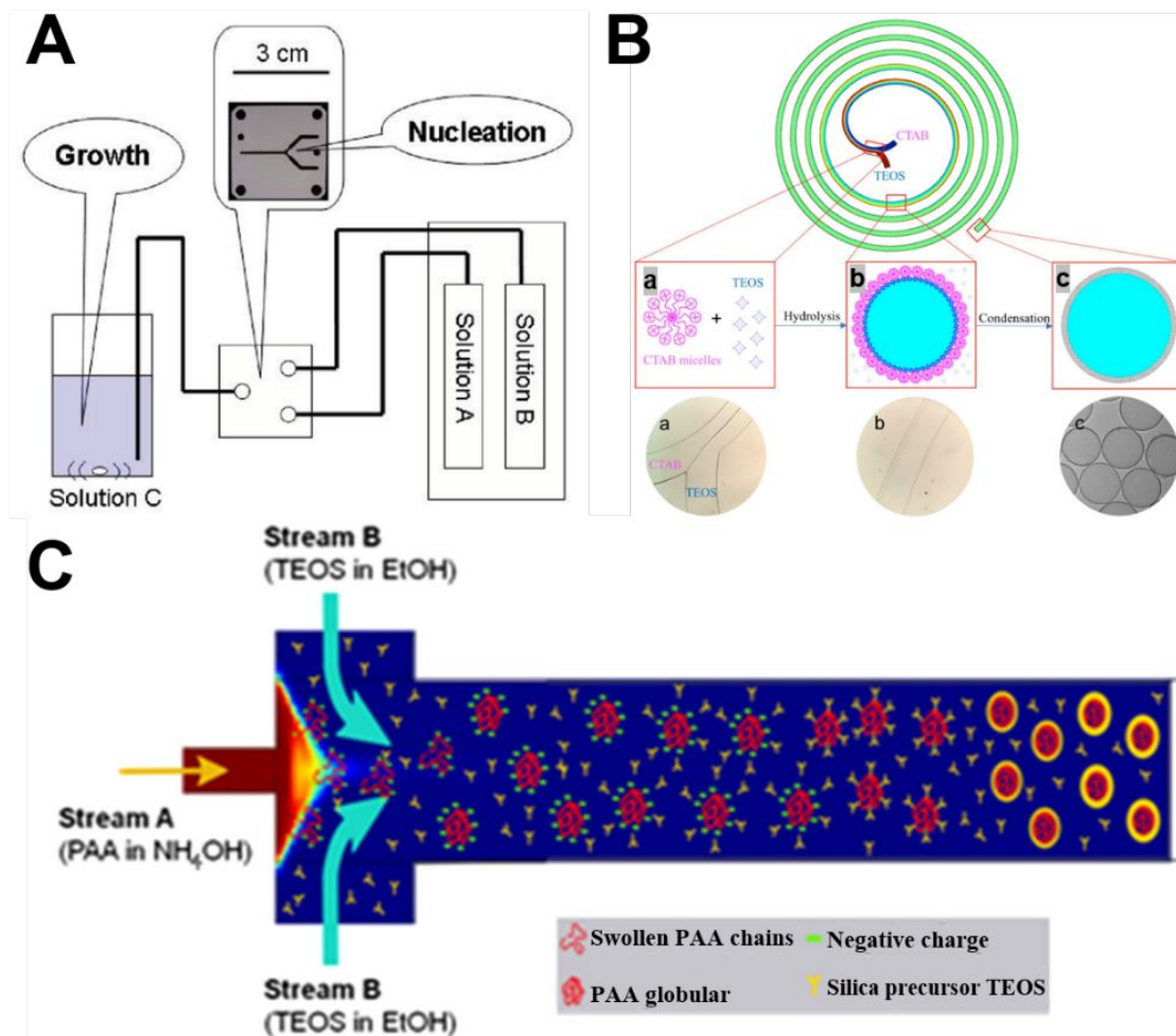
Figure 4. Examples of laminar flow microreactors for the synthesis of nanoporous silica sphere. (A) Schematic of the reaction setup for the synthesis of nanoporous silica sphere. Solutions A, B, and C are TEOS/MeOH, MeOH aqueous, and CTAC/MeOH aqueous, respectively. Reproduced with permission from ref. 43 . (B) Synthesis of submicrometer hollow silica sphere in spiral-shaped microreactor. (a) TEOS in pure ethanol and CTAB micelles in diluted ammonia were flowed into the spiral microchannel; (b) hydrolysis of TEOS occurred at the interface of the two laminar flows; (c) hollow silica spheres were collected at the outlet. Reproduced with permission from ref. 56 . (C) Formation mechanism of PAA spherical templates in the microreactor with hydrodynamic focusing micromixer for the synthesis of hollow silica nanoparticles. Mixing profile of the solutions was computed from a COMSOL model. Reproduced with permission from ref. 55 .
