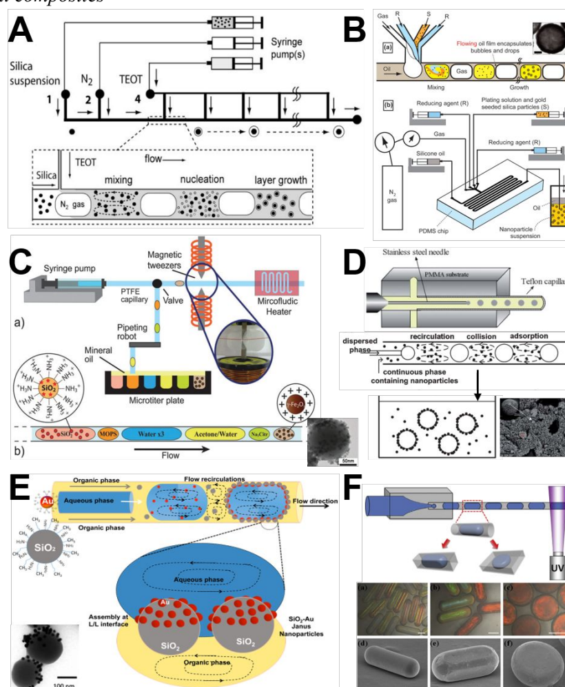
Figure 10. Examples of discrete segment and droplet microreactors for the synthesis of hierarchical composites. (A) Microfluidic synthesis of titania shells on colloidal silica ( \text{SiO}_2@\text{TiO}_2 ) at the gas-liquid interface. Reproduced with permission from ref. 81 . (B) Microfluidic foam generation of plasmonic nanoshell on silica surface. Reproduced with permission from ref. 93 . (C) Microfluidic droplet flow synthesis of silica nanoparticles coated with iron oxide nanoparticles. Reproduced with permission from ref. 112 . (D) Droplet flow synthesis of silica-chitosan hybrid
