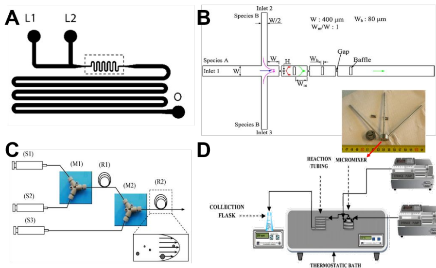
Figure 3. Examples of laminar flow microreactors for the synthesis of solid silica sphere. (A) Schematic of microchannel has two liquid inlets (L1 and L2) and one outlet (O). Reproduced with permission from ref. 39 . (B) Schematic diagram of the baffled micromixer with three mixing units. Reproduced with permission from ref. 45 . (C) Schematic diagram of microreactor system for silica synthesis. (S1), (S2), and (S3) are syringe for TMOS, HCl, and PEI polymer in Tris-HCl buffer solution, respectively. (M1) and (M2) are Y-shaped mixers. (R1) is the reaction tube for hydrolysis, (R2) is the reaction tube for silica precipitation. Reproduced with permission from ref. 46 . (D) Experimental setup using standard slit interdigital micromixer for the continuous silica particle synthesis. Reproduced with permission from ref. 44 .
