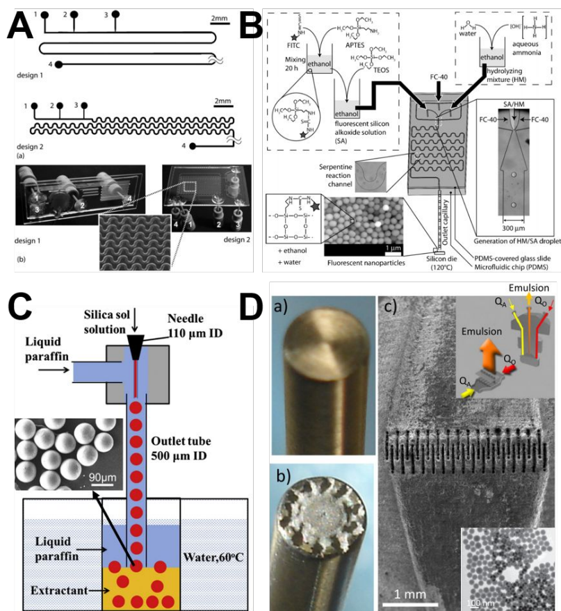
Figure 7. Examples of discrete segment and droplet microreactors for the synthesis of solid silica sphere. (A) Segmented gas-liquid flow microreactors with straight-walled channels (design 1) and meandering channels (design 2) for solid silica sphere synthesis. Number 2 is the gas inlet. Reproduced with permission from ref. 40 . (B) Procedure and setup for the droplet-based synthesis of silica sphere. Reproduced with permission from ref. 99 . (C) Droplet synthesis of silica microspheres. Reproduced with permission from ref. 108 . (D) Microfluidic interdigital mixer used to produce the silica nanosphere by microchannel emulsification. Reproduced with permission from ref. 117 .
