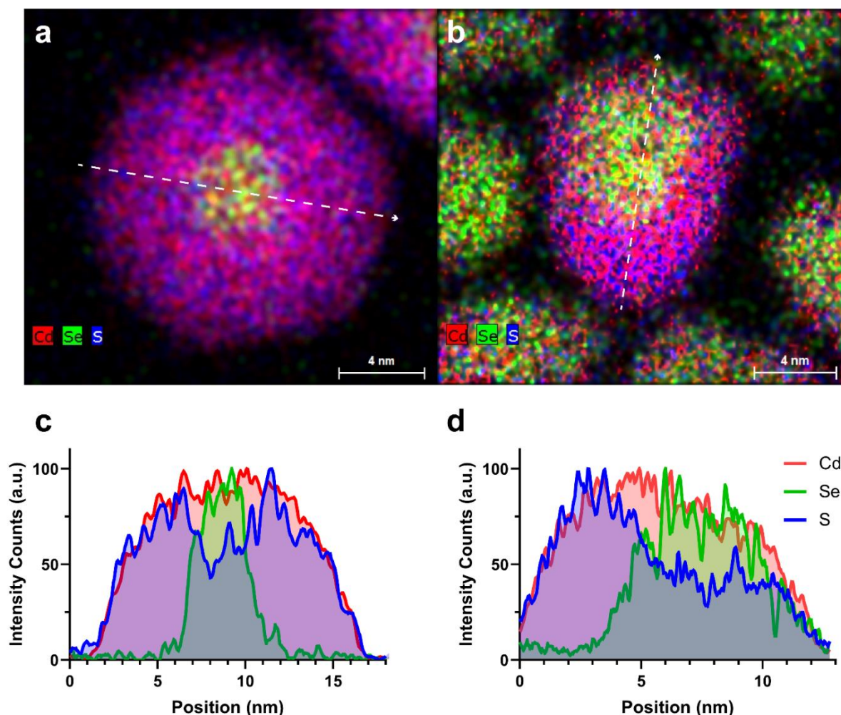
Fig. 1 Elemental characterization of CdSe/CdS QD architectures. Combined Cd (red), Se (green), and S (blue) elemental maps of a) Symmetrically shelled QDs and (b) QD655s show core/shell structures. Linescans of the elemental maps (white arrows) Se distribution relative to Cd and S in both (c) Symmetrically shelled QDs and (d) QD655s.
