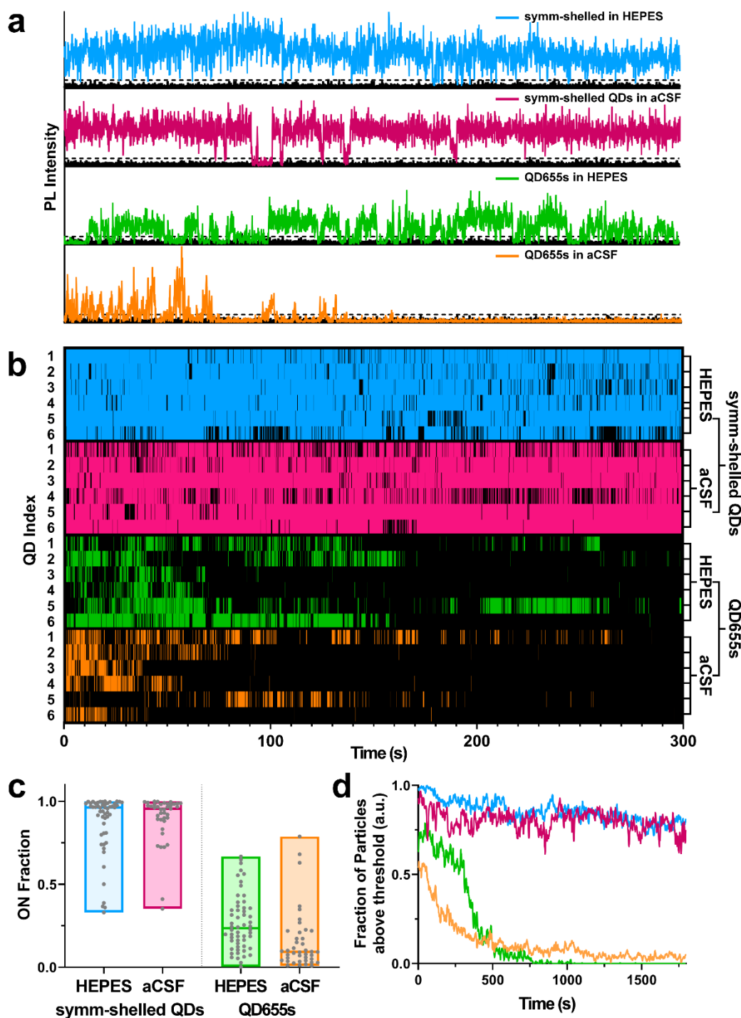
Fig. 3 Time series and blinking behaviour of single QDs. (a) Representative intensity trajectories for symmetrically shelled (symm-shelled) QDs and QD655s in both HEPES and oxygenated artificial cerebrospinal fluid (aCSF). (b) Subsets of blinking dynamics for symm-shelled QDs and QD655s in HEPES and aCSF. A total of 6 particles per condition were populated to display blinking behaviour. Colours represent times that the particle was in the ON state. (c) Comparison of ON fraction populations under each condition ( N \geq 40 QDs). (d) Comparison of photobleaching profiles for symm-shelled QDs vs QD655s under each condition ( N > 40 QDs).
