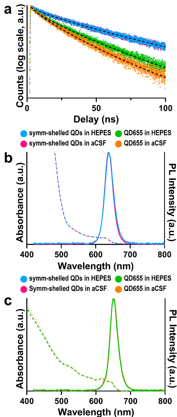
Fig. 2 Ensemble photophysical profiles of symmetrically shelled (symm-shelled) CdSe/CdS QDs and QD655s in HEPES buffer or oxygenated cerebrospinal fluid (aCSF). (a) Transient PL dynamics of symm-shelled QDs and QD655s in HEPES and oxygenated aCSF. (b) Absorbance (dotted) and emission (solid) spectra of (b) symm-shelled QDs and (c) QD655s in HEPES and oxygenated aCSF.
