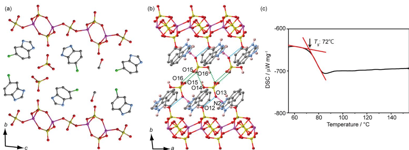
Fig. 1 (a) Crystal structure of [\{\text{Zn}_2(\text{HPO}_4)_2(\text{H}_2\text{PO}_4)\}(\text{ClbimH}^+)_2 \cdot (\text{H}_2\text{PO}_4^-)_n \cdot (\text{MeOH})_m] ( 1 ) viewed along the a axis at 223 K. (b) Hydrogen-bond (H-bond) network around guest \text{H}_2\text{PO}_4^- viewed from the c axis. H-bonds between guest \text{H}_2\text{PO}_4^- , guest \text{H}_2\text{PO}_4^- –ClbimH + , and guest \text{H}_2\text{PO}_4^- –coordinated \text{H}_2\text{PO}_4^- are drawn as green, blue, and pink dotted lines, respectively. (c) Differential scanning calorimetry curve of glass-form 1 ( 1g ). [Color coding: purple, Zn; yellow, P; red, O; blue, N; black, C; green, Cl; and light pink, H.]
