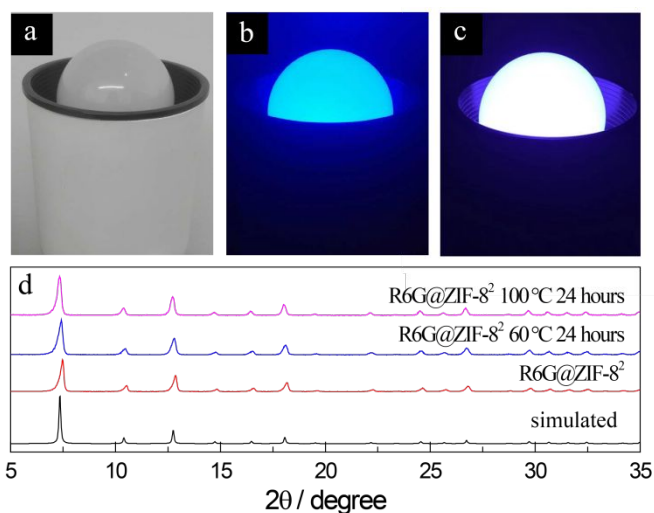
Fig. 3 Photographs of 450 nm blue light LED lamp when power is turned off (a) and on (b); and photograph of the LED lamp coated with R6G@ZIF-8 2 when the LED is turned on (c); (d) PXRD patterns changes before and after the treatments (heated at different temperature for 24 hours).
