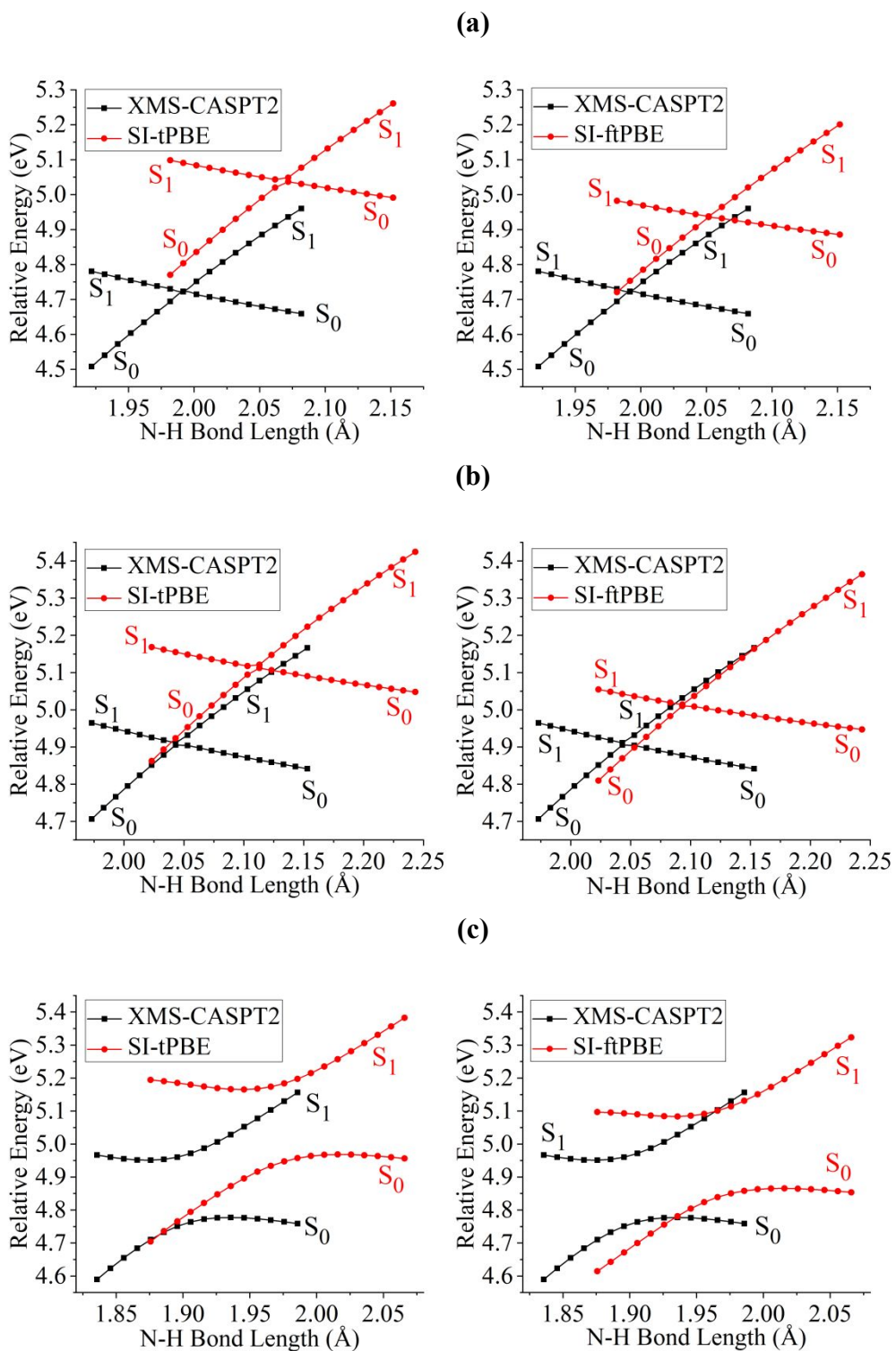
Figure 6. PESs for N-H bond fission of (a) eclipsed-H3, (b) eclipsed-H2 and (c) staggered methylamine near the LAC region with various methods. The relative energies are compared with those of equilibrium geometry for each method.
