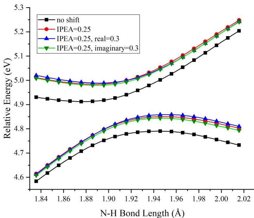
Figure 2. PESs for N-H bond fission of staggered methylamine near the LAC with various choices of IPEA and real or imaginary level shifts in MS-CASPT2 calculations. The energies are relative to those of the equilibrium geometry for each combination of options.
