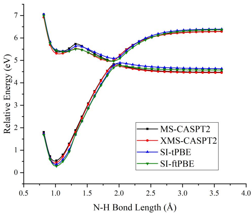
Figure 5. PESs for N-H bond fission of staggered methylamine with various methods. The relative energies are compared with those of equilibrium geometry for each method.
