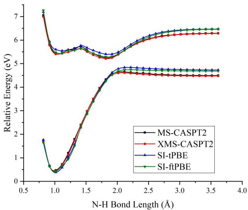
Figure 8. PESs for N-H bond fission of methylamine with H6-C4-N1-H3 dihedral angle equaling 100^\circ using various methods. The relative energies are compared with those of equilibrium geometry for each method.
