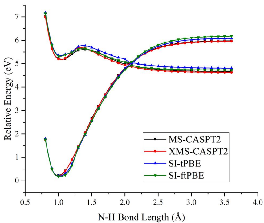
Figure 4. PESs for N-H bond fission of eclipsed-H 2 methylamine with various methods. The relative energies are compared with those of equilibrium geometry for each method.
