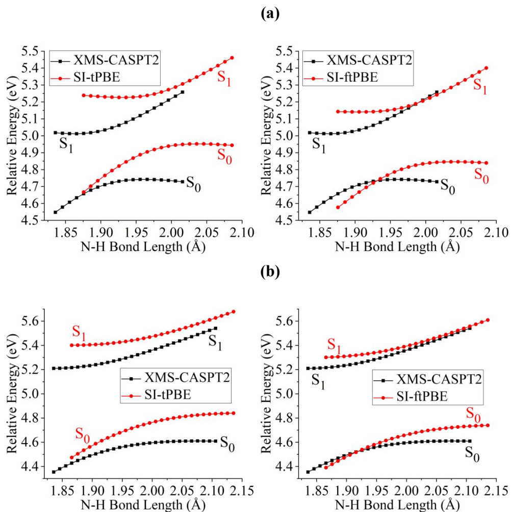
Figure 9. PESs for N-H bond fission of methylamine with H6-C4-N1-H3 dihedral angle equaling (a) 95^\circ and (b) 100^\circ near the LAC region with various methods. The relative energies are compared with those of equilibrium geometry for each method.
