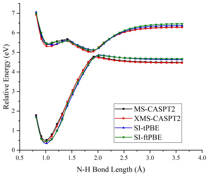
Figure 7. PESs for N-H bond fission of methylamine with H6-C4-N1-H3 dihedral angle equaling 95^\circ using various methods. The relative energies are compared with those of equilibrium geometry for each method.
