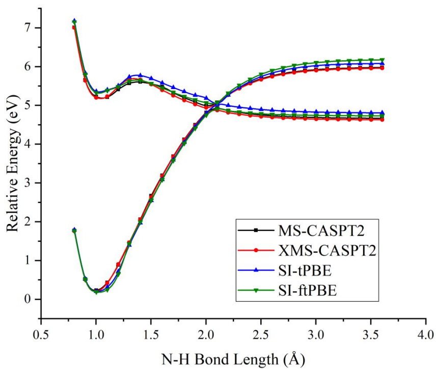
Figure 3. PESs for N-H bond fission of eclipsed-H3 methylamine with various methods. The relative energies are compared with those of equilibrium geometry for each method.
