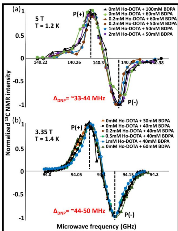
Figure 1. Normalized ^{13}\text{C} DNP microwave sweeps of 1:1 (v/v) sulfolane/[ ^{13}\text{C} ]pyruvic acid in the presence of variable concentrations of BDPA radical and Ho-DOTA a) At 5 T, (50 or 60 or 100 mM) BDPA doped with 0, 0.2, 1, 2 mM of Ho-DOTA b) At 3.35 T with 30 or 40 or 60 mM BDPA doped with 0, 0.2, 0.5, and 1 mM Ho-DOTA. Note the slight shift in the locations of P(+) and P(-) towards each other with increasing concentrations of Ho-DOTA for both systems.
