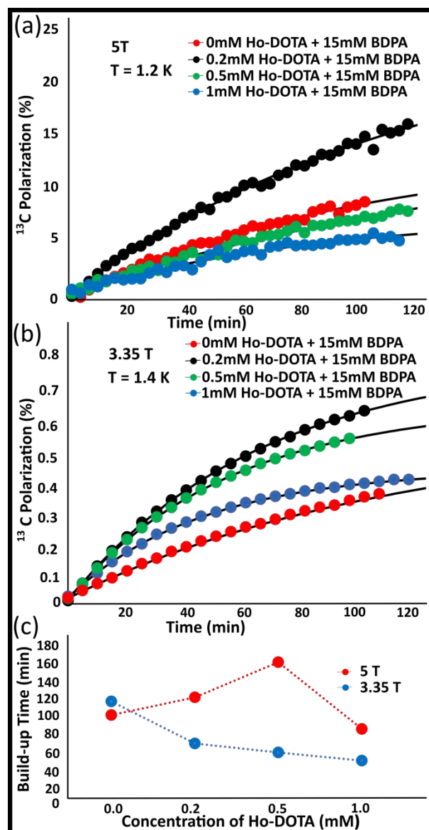
Figure 3. 13 C DNP polarization of 25 \mu l of 1:1 (v/v) sulfolane/[1- 13 C]pyruvic acid in the presence of 15 mM BDPA radical doped with various concentrations of Ho-DOTA (0, 0.2, 0.5, 1 mM) a) at 5 T b) at 3.35 T c) Buildup times for various concentrations of Ho-DOTA with 15 mM BDPA radical. The samples were polarized at the positive polarization peak with a 100 mW microwave source. At 3.35 T, the buildup time decreases with increase in concentration of Ho-DOTA. At 5 T, after an initial increase in buildup time, there is a sharp decrease at 1.0 mM Ho-DOTA.
