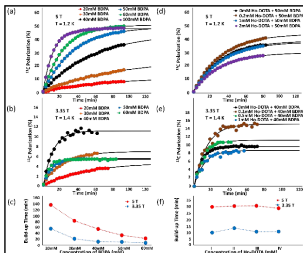
Figure 2. Time dependent ^{13}\text{C} DNP polarization of 25 \mu\text{L} of 1:1 (v/v) sulfolane/[ ^{13}\text{C} ]pyruvic acid (solid state) in the presence of variable concentrations of BDPA radical (20, 30, 40, 50, 60 mM) at a) 5 T and b) 3.35 T. c) DNP buildup times as extracted from fitting with a single exponential for various concentrations of BDPA. Buildup times decrease with increasing concentration of BDPA at both field strengths. Similarly, figure 2d, e, and 2f are ^{13}\text{C} DNP polarization buildups for 1:1 (v/v) sulfolane/[ ^{13}\text{C} ]pyruvic acid with BDPA and various concentrations of Ho-DOTA (0, 0.2, 0.5, 1 mM) d) 50 mM BDPA for 5 T system. Note the 50 mM BDPA curve with no Ho-DOTA does not match the observed polarization in a) as the samples were prepared in different batches. With such high concentrations of radical in limited volumes, excursions in absolute polarizations were nearly unavoidable. e) 40 mM BDPA for 3.35 T system f) Buildup times as a function of Ho-DOTA concentration with 40 (at 3.35 T) or 50 mM (at 5 T) BDPA radical. The samples were polarized at the positive polarization peak with a 100 mW microwave power source.
