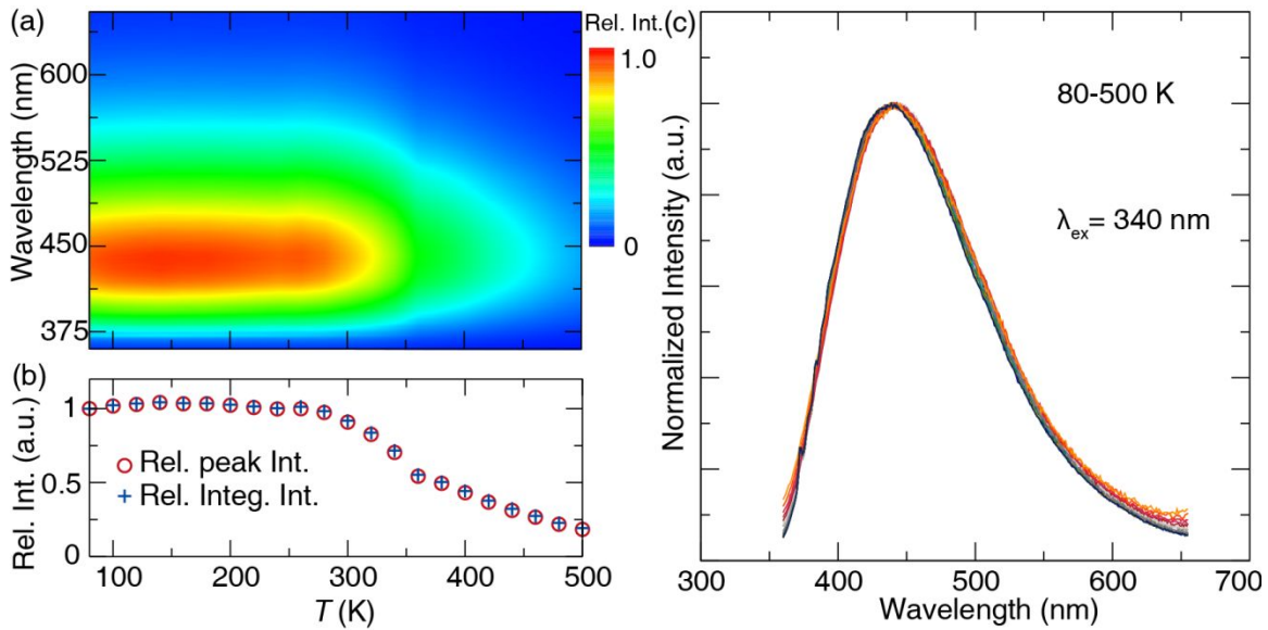
Figure 8 Contour plot of the normalized emission spectra of (\text{Ba}_{0.95}\text{Ce}_{0.05})_5\text{Si}_8\text{O}_{21} excited at 340 nm as a function of temperature; (b) relative integrated intensity of the emission spectra (rel. integ. int.) and the relative intensity of the emission peak (rel. peak int.) as a function of temperature; and (c) all normalized emission spectra of (\text{Ba}_{0.95}\text{Ce}_{0.05})_5\text{Si}_8\text{O}_{21} measured between 80 and 500 K.
