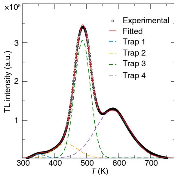
Figure 10 Thermoluminescence curve of (\text{Ba}_{0.95}\text{Ce}_{0.05})_5\text{Si}_8\text{O}_{21} collected from 320 K to 750 K with a heating rate of 1 K/s after being excited ( \lambda_{\text{ex}} = 254 nm) for 10 min.
