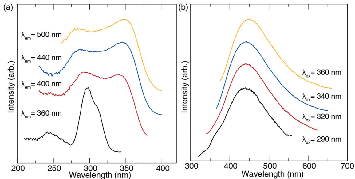
Figure 6 a) The excitation spectra of (\text{Ba}_{0.95}\text{Ce}_{0.05})_5\text{Si}_8\text{O}_{21} monitored at different emission wavelengths; b) The emission spectra excited by different excitation wavelengths.
