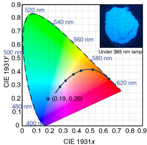
Figure 9 CIE coordinates of (\text{Ba}_{0.95}\text{Ce}_{0.05})_5\text{Si}_8\text{O}_{21} when excited at 340 nm; the inset presents a photograph of this phosphor under a 365 nm lamp.
