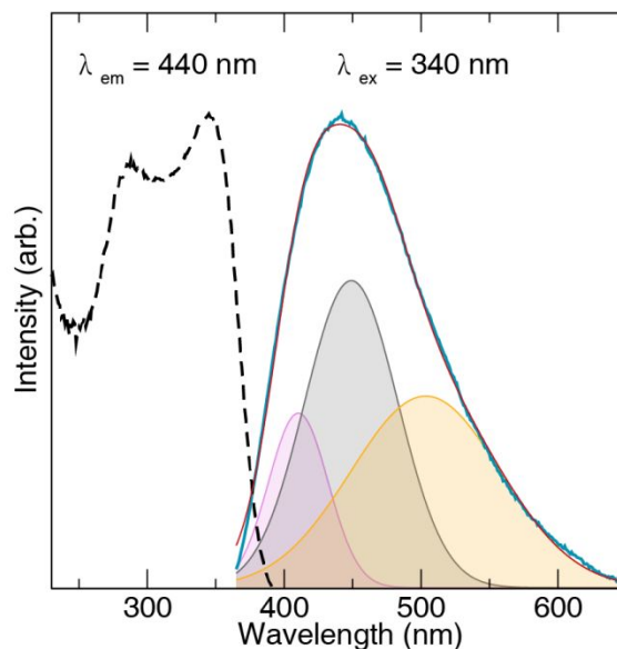
Figure 5 Photoluminescent excitation and emission spectra of (\text{Ba}_{0.95}\text{Ce}_{0.05})_5\text{Si}_8\text{O}_{21} at room temperature. The emission spectra is well fitted (by red curve) to present three Gaussian bands (violet, gray and orange) characteristic of \text{Ce}^{3+} .
