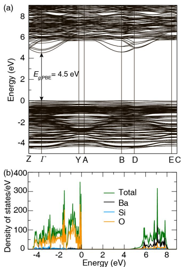
Figure 4 a) Band structure and b) density of states of Ba_5Si_8O_{21} calculated using the PBE functional.
