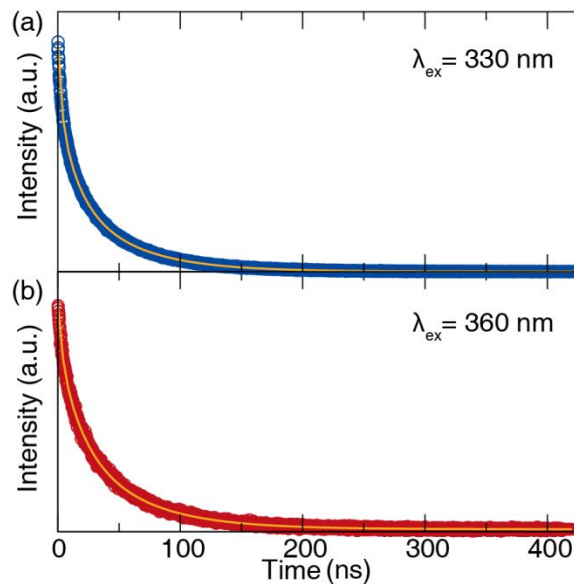
Figure 7 Time-gated photoluminescence decay curves of (\text{Ba}_{0.95}\text{Ce}_{0.05})_5\text{Si}_8\text{O}_{21} collected under a) 330 nm, and b) 360 nm excitation, respectively. The blue and red dots represent the collected data and the yellow line is the fit.
