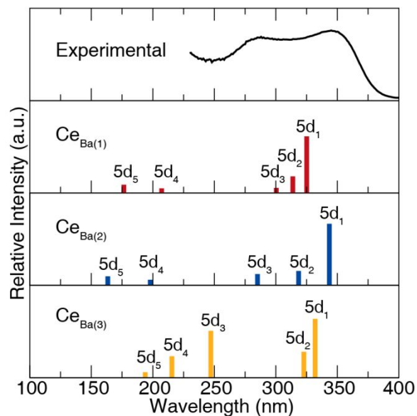
Figure 11 Schematic of the calculated energy and relative oscillator strengths of 4f \rightarrow 5d transitions of \text{Ce}^{3+} substituted on the different \text{Ba}^{2+} sites present in \text{Ba}_5\text{Si}_8\text{O}_{21} , compared with the experimental excitation spectra.
