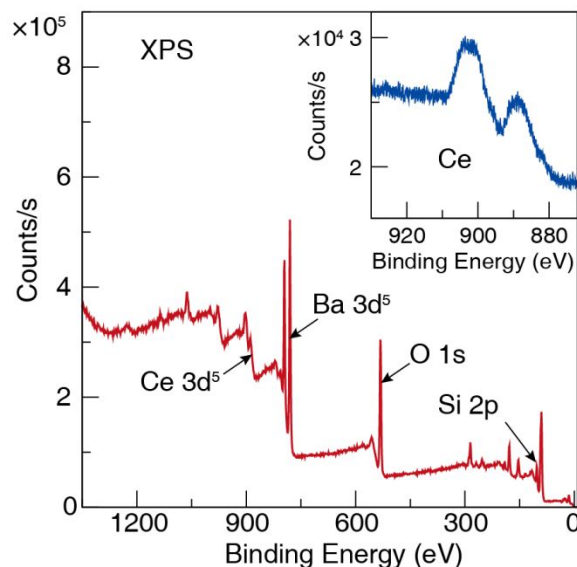
Figure 3 X-ray photoelectron spectroscopy (XPS) survey of (\text{Ba}_{0.95}\text{Ce}_{0.05})_5\text{Si}_8\text{O}_{21} with the inset highlighting Ce 3d in this sample.
