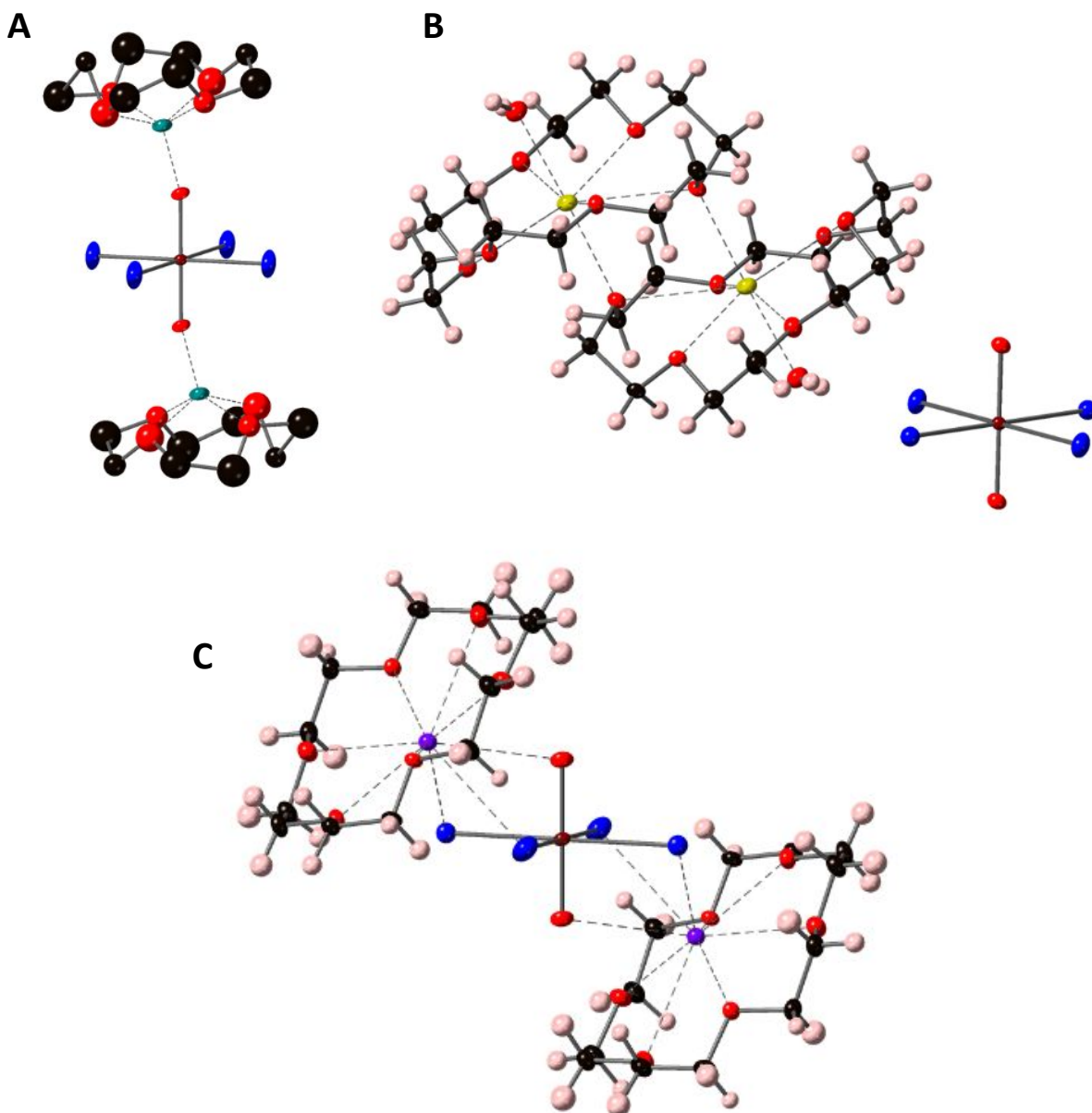
Figure 3. Second sphere coordination between the alkali metal encapsulated within the crown ether molecule and the [(\text{NpO}_2)\text{Cl}_4]^{2-} complexes for (a) LiNp , (b) NaNp , and (c) KNp . The Np, Cl, O, C, Li, Na, and K atoms are represented by dark red, blue, red, black, teal, yellow and purple ellipsoids, respectively.
