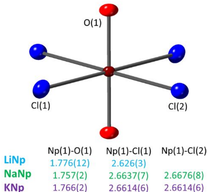
Figure 2. [(\text{NpO}_2)\text{Cl}_4]^{2-} coordination complex observed in the LiNp , NaNp , and KNp compounds with Np=O and Np-Cl bond distances determined from analysis by single-crystal X-ray diffraction.
