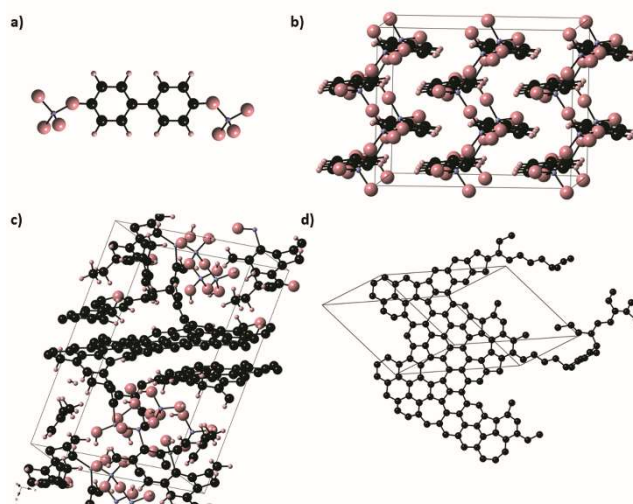
Fig. 9. Polymer fragment (a) used to build periodic models. Optimized structures obtained from ab-initio molecular dynamic simulations of heating a model of the DA-polymer at 1200 K (b) and 3000 K (c). The extended carbon arrangement found in the 3000 K model (d). The simulation was performed for about 150 ps under constant pressure allowing the cell to change its shape, though the density remained almost constant ( \rho=1.6 \text{ g/cm}^3 ) throughout the simulation. The composition is \text{Si}_8\text{O}_{24}\text{C}_{96}\text{H}_{64} , no gaseous species were removed during the simulation.
