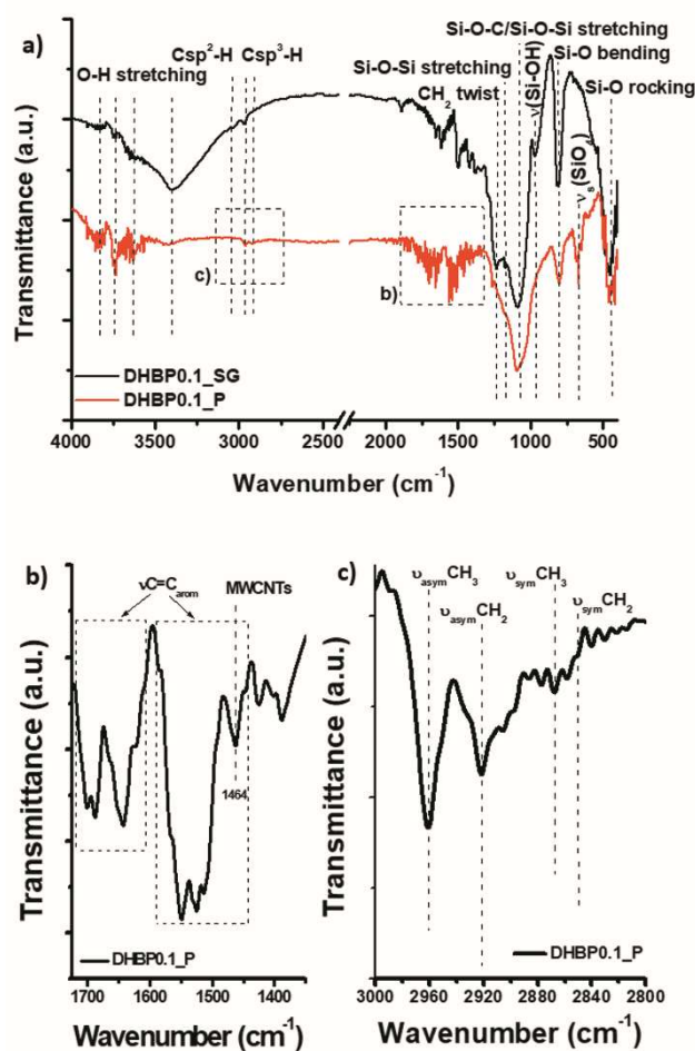
Fig. 6. a) FTIR spectrum of single source precursor DHBPO.1_SG as compared to DHBPO.1_P prepared via pyrolysis at 900 °C. b) The region corresponding to conjugated C=C vibration bands of free carbon phase in DHBPO.1_P; c) The presence of -CH 2 - and -CH 3 vibration modes in DHBPO.1_P. Please note the absence of any Csp 2 -H bonds in ceramic.
