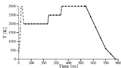
Fig. 14. Time vs. temperature scheme of annealing the polymer (Fig.2) model of composition \text{SiC}_{12}\text{O}_3\text{H}_8 model comprising 12288 atoms. Dashed line – NVT ensemble, time step 0.1 fs; solid line – NPT ensemble, time step 0.2 fs. At the moments of time marked with points we removed gaseous molecules \text{H}_2 , \text{CO} , \text{CO}_2 , \text{H}_2\text{O} , \text{O}_2 , \text{CH}_2\text{O} , \text{C}_2\text{H}_2 , \text{C}_2\text{H}_4 .
