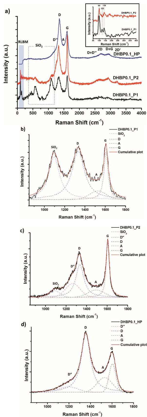
Fig. 7. Micro-Raman analysis of the ceramic sample as prepared at 900 (2 distinctive profiles, DHBPO.1_P1 and DHBPO.1_P2) and 1600 °C (DHBPO.1_HP). Fitting of the region 850-1800 cm^{-1} for b) DHBPO.1_P1, c) DHBPO.1_P2 and d) DHBPO.1_HP.
