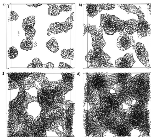
Fig. 11. Carbon structures in SiOC obtained at high annealing temperature in empirical potential simulations. The amount of “free” carbon increases in the sequence, C:Si = 0.5, 1, 2, 3. Only C atoms are shown, while Si and O have been omitted. All models exhibit a density of 2.2 g/cm 3 , the size of the (periodic) simulation box increases from 7.4 to 8.4 nm with increasing carbon content.
