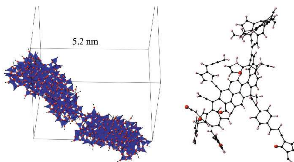
Fig. 13. SiOC structure obtained through reactive force field simulations after annealing DHBPO.1_SG. (left) two segregated silica beans; (right) a typical fragment of carbon with curvature.
