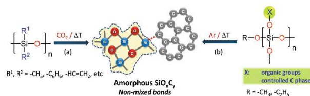
Fig. 1. Synthesis approach toward non-mixed bonded \text{SiO}_x\text{C}_y ceramics (i.e., C/ \text{SiO}_2 nanocomposites) via pyrolysis of polysiloxanes in \text{CO}_2 atmosphere 1 (a) or via thermal decomposition of orthosilicate-based sol-gel systems containing large, aromatic organic substituents (b). The difference of the novel approach (b) consists in using precursors containing no Si-C bonding in the structure, silicon being bonded only to oxygen.
