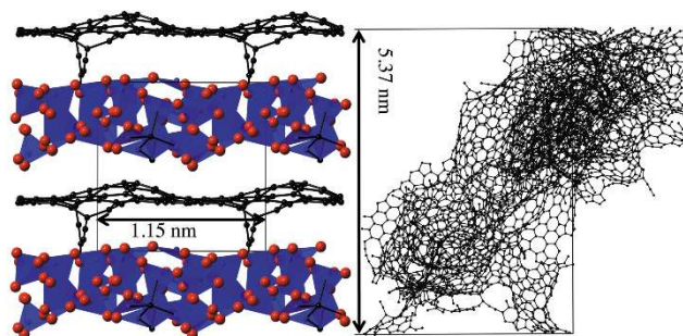
Fig. 12. Amorphous silicon oxycarbide models (composition Si 5 CO 8 +10C; density 2.2 g/m 3 ) generated via melt-quench simulations using the reactive force field. On the left a small 120-atom model showing graphene sheet segregated between “glassy” SiOC. Box sizes of this model are ~1.2 nm. On the right the “free” carbon structure in a 12288-atom model (box sizes ~5.4 nm). Si and O are not shown in this model for clarity.
