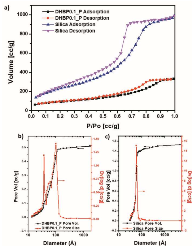
Fig. 8. a) BET isotherm analysis of DHBP0.1_P as compared with silica. Pores size distribution and pore volume for b) DHBP0.1_P and b) Silica. Please note that both samples were produced by pyrolysis at 900 °C in Argon atmosphere.
