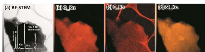
Fig. 5. a) Bright field scanning electron microscopy (BF-STEM) of DHBPO.1_P. Inset of EDX measured under BF-STEM. Element mapping of O_K \alpha (b), C_K \alpha (c) and Si_K \alpha (d) under STEM.
