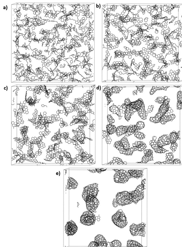
Fig. 10. Carbon structures in SiOC for the composition \text{SiO}_2:\text{C}_{0.5} , \text{C}:\text{Si} = 1:2 obtained in empirical potential simulations. Only C atoms are shown, Si and O have been omitted. The sequence of pictures corresponds to annealing at increasingly higher temperature (parameter T_{\text{MC}} in MC-simulations). The size of the (periodic) simulation box is 7.4 nm, the density of all SiOC models is 2.2 \text{ g/cm}^3 .
