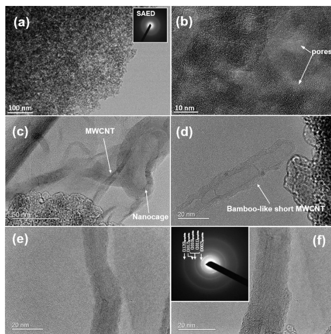
Fig. 4. Transmission electron microscopy of DHBP0.1_P revealing a) and b) the microporous structure, c) the presence of long defective MWCNTs as well as bean-like carbon nanocages; d) short bamboo-like carbon nanotubes; e) and f) defective long bamboo-like MWCNTs where scrolls coexist within a tube.
