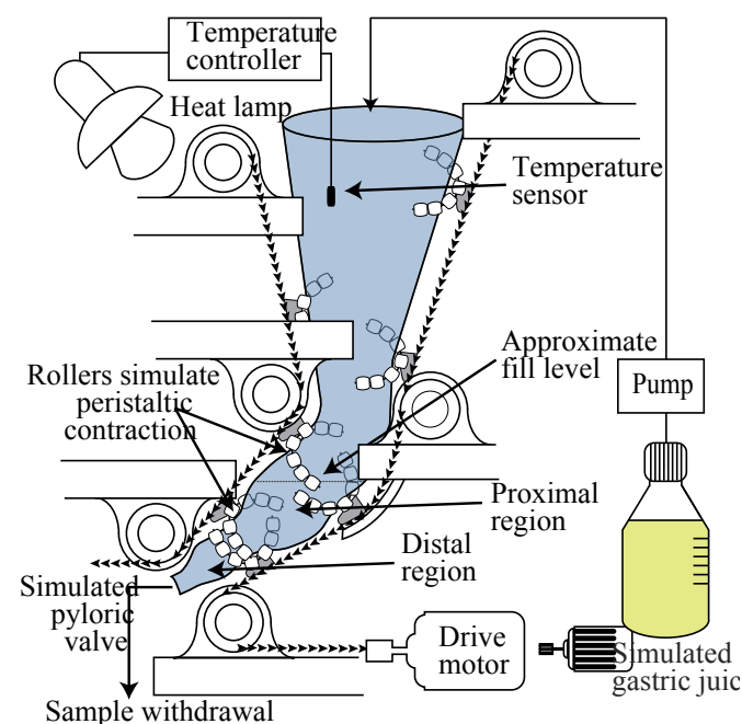
Figure 1. Diagram of the Human Gastric Simulator (HGS).
