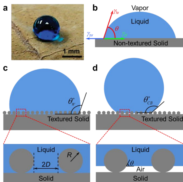
Figure 4. a) A droplet of water (dyed blue) beading up on a lotus leaf. Reproduced with permission. 130 © 2014 Nature Publishing Group. Schematic of a liquid droplet b) on a non-textured solid surface, c) in the Wenzel state on a textured solid surface, and d) in the Cassie-Baxter state on a textured solid surface. Note: \theta^* , apparent contact angle; \theta , Young's contact angle; R , radius of the feature; D , half the inter-feature spacing.
