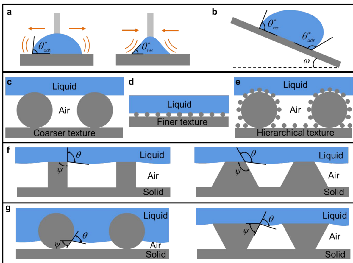
Figure 5. Schematic illustrating the a) advancing (the maximum) and receding (minimum) contact angles on a solid surface, b) a liquid droplet sliding on a tilted surface with the roll off angle of \omega . Schematics of a liquid droplet in the Cassie-Baxter state on c) a coarser textured surface, d) a finer textured surface, and e) a hierarchically structured surface, respectively. Schematics of a liquid droplet on f) concave textures with \psi \geq 90^\circ showing a liquid with \theta > 90^\circ in the Cassie-Baxter state, g) convex (re-entrant) textures with \psi < 90^\circ showing a liquid with \theta < 90^\circ in the Cassie-Baxter state. Note: \psi , local texture angle.
