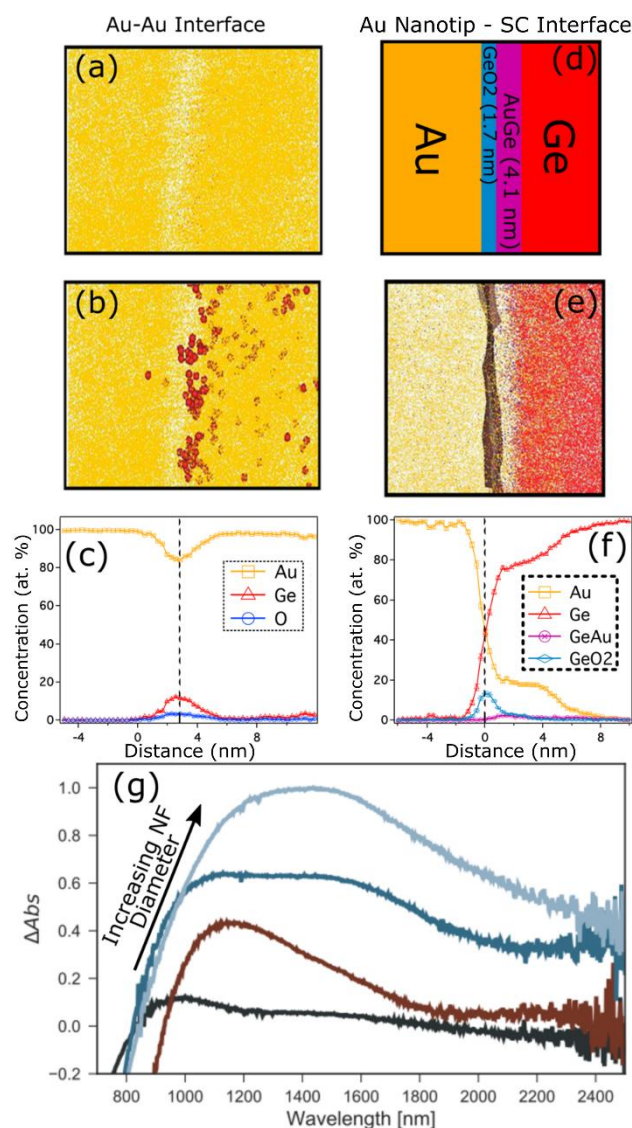
Figure 3 Atom-probe tomographic (APT) results from a Au-NF tip region. (a-b) Atom-probe tomography reconstruction of the Au-Au interface. Colours correspond to the legend presented in figure 3c. (c) Proximity histogram of the Au-Au interfaces shows gold clusters separated by an oxide layer. (d) Schematic of the Au-Ge interface. Colours correspond to the legend presented in figure 3f (e) Atom-probe tomography reconstruction of the Au-Ge interface (brown), indicated by an Ge 50 atomic % isoconcentration surface. (f) Proximity histogram of the Au tip-NW interface show a dielectric layer ( GeO_2 ) and AuGe layer formed between the tip and SC NW. Figures (a) through (f) were constructed using the proximity histogram methodology, which we have developed and used extensively as an aid to interpreting 3-D atom-probe tomographic
