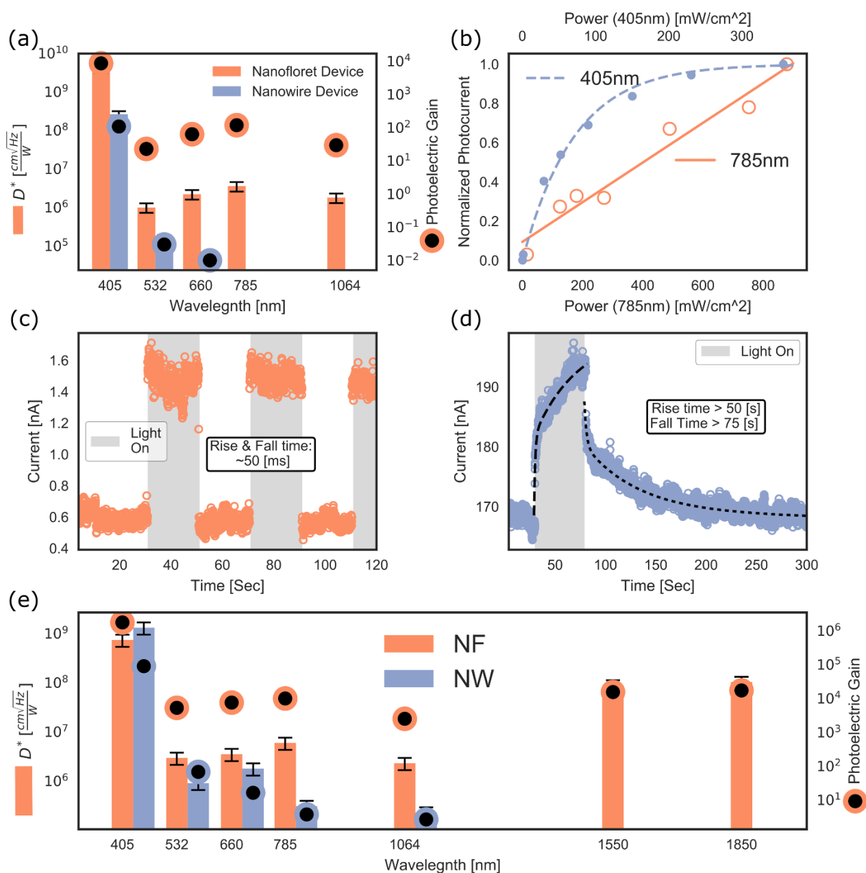
Figure 2 (a) Specific detectivity, D^* , and photoelectric gain, g , as a function of wavelength for the NF and NW devices. At all wavelengths the NF device is superior to the NW device. A difference exists between the UV (405 nm) regime and the 532 nm to 1064 nm regime, suggesting for different photo-response mechanisms. (b) Photocurrent optical power dependence for illumination with 405 nm and 785 nm wavelengths; at 785 nm the dependence is linear while at 405 nm the response saturates in the power range we utilized. (c-d) comparison between the photo-responses of (c) NF and (d) NW devices for illumination with a wavelength of 660 nm, where the rise and fall times of the NF device are shorter. The gray areas represent the light on periods. (e) The NF's device photo-response as a function of wavelength, for a device with pronounced surface states.
