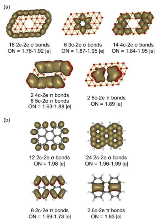
Fig. 5 Comparison of the AdNDP patterns for closed-shell C_2 B_{32} (a) and PAH C_{20}H_{12} (b). ON represents occupation number.
