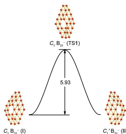
Fig. 6 Chiral conversion between two degenerate enantiomers of B_{31}^- ( C_1 I and C_1' II ) via buckling through transition state C_1 B_{31}^- ( TS1 ). The relative energy is given in kcal/mol at the CCSD(T)/6-311G(d)//PBE0/6-311+G(d) level.
