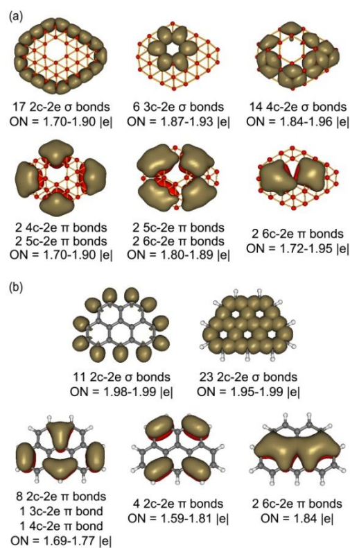
Fig. 4 Comparison of the AdNDP patterns of GM B_{31}^- (a) and PAH C_{19}H_{11}^- (b). ON represents occupation number.
