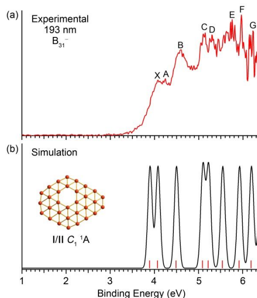
Fig. 1 Photoelectron spectrum of B_{31}^- at 193 nm, compared with simulated spectra of the lowest-lying isomers of B_{31}^- (I and II) at the TD-PBE0/6-311+G(d) level. The simulated spectra were obtained by fitting the calculated VDEs (vertical red bar) with unit-area Gaussian functions of 0.05 eV half-width.
