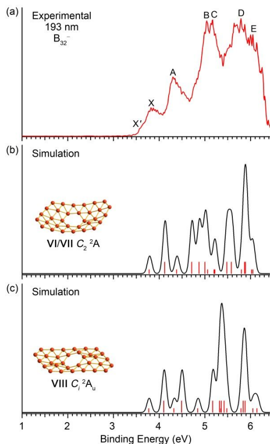
Fig. 2 Photoelectron spectrum of B_{32}^- at 193 nm compared with the simulated spectra of the lowest-lying isomers of B_{32}^- ( VI and VII ) and a low-lying isomer ( C_i , VIII ) at the TD-PBE0/6-311+G(d) level. The simulated spectra were obtained by fitting the calculated VDEs (vertical red bar) with unit-area Gaussian functions of 0.05 eV half-width.
