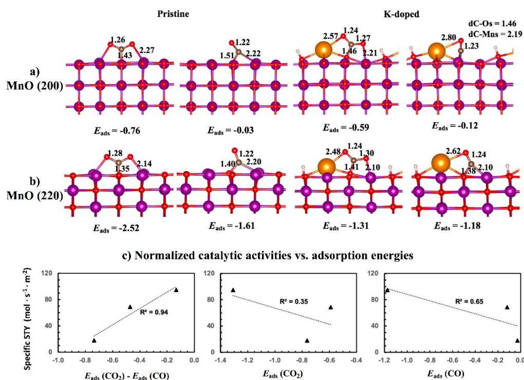
Fig. 6 Optimized structures and corresponding adsorption energies of CO 2 and CO on pristine and K + -doped (a) MnO (200) and (b) (220) surfaces. (c) Correlations between the measured specific STY at 800 °C and the calculated absorption energies of CO 2 and CO and their differences. Purple, brown, red, orange, and white balls represent Mn, C, O, K, and H atoms, respectively. Key bond lengths are shown in the unit of Å and the calculated adsorption energies are in the unit of eV.
