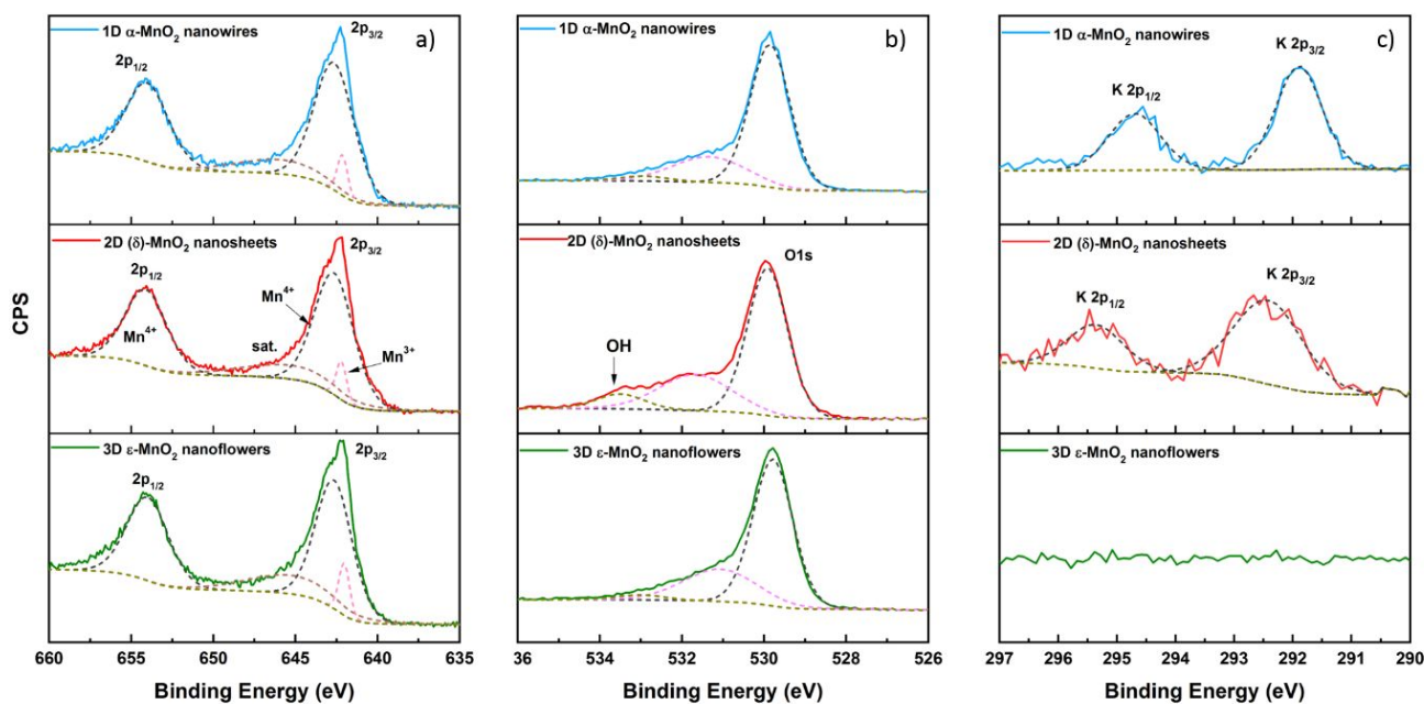
Fig. 2 XPS deconvolution spectra at (a) Mn 2p displaying \text{Mn}^{4+} 2p_{3/2} and 2p_{1/2} as well as the characteristic identifiable shape of \text{MnO}_2 ; (b) O1s, from which we find that \text{MnO}_2 nanosheets possess hydroxyl groups in the structures; (c) K 2p, \text{K}^+ was found both in \alpha\text{-MnO}_2 nanowires and ( \delta )- \text{MnO}_2 nanosheets but not in nanoflowers.
