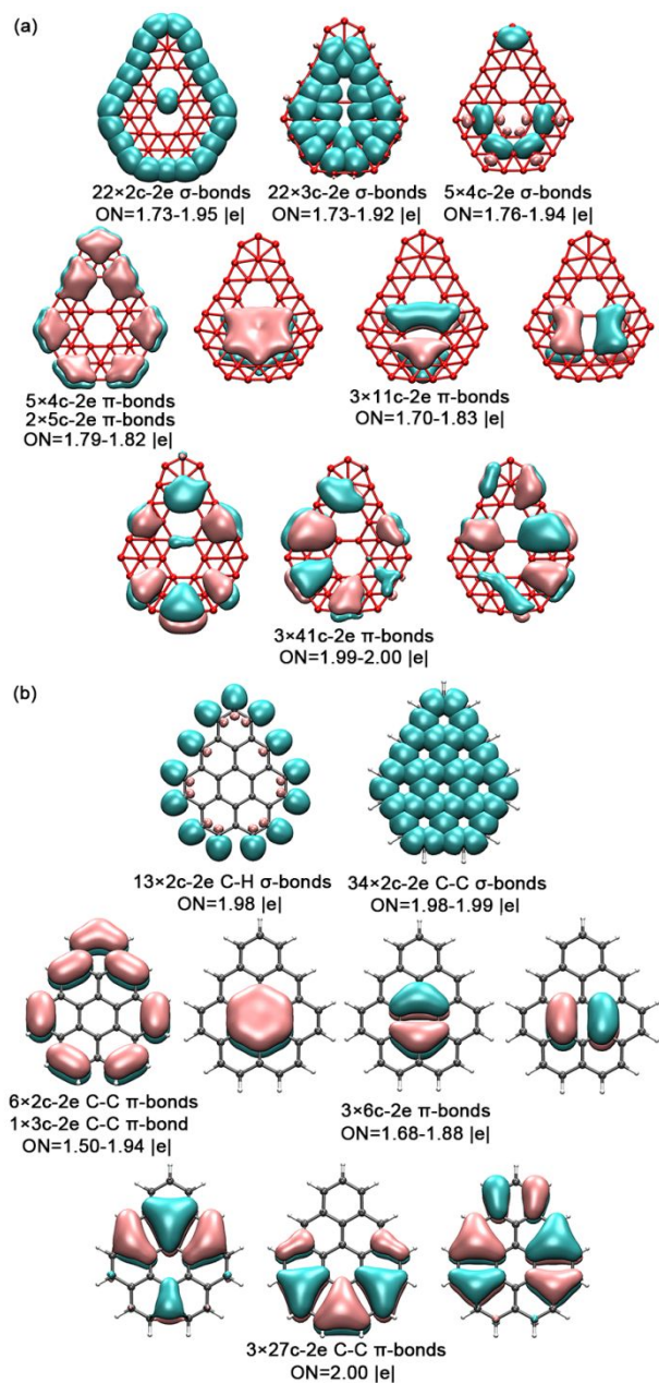
Fig. 5 The AdNDP bonding analysis for (a) C_5 B_{41}^- in comparison with that of (b) C_{2v} C_{27}H_{13}^+ . Occupation numbers (ONs) are shown.
