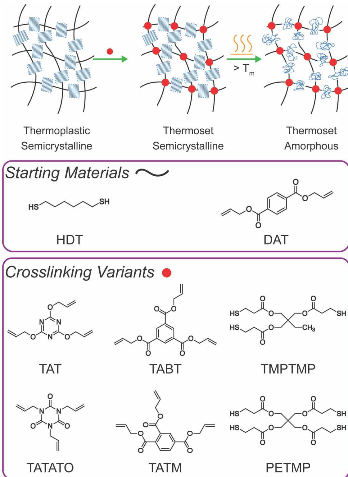
Fig. 1 Schematic of the photopolymerization approach used produce semicrystalline, crosslinked thiol-ene materials to improve the mechanical performance of printed components. A stoichiometric amount of crosslinker was included in the original HDT-DAT formulation at concentrations low enough to maintain crystallinity. Several prints were processed post-manufacture by heating above T_m and conditioning at that temperature until the crystallites melted to form an amorphous network.
