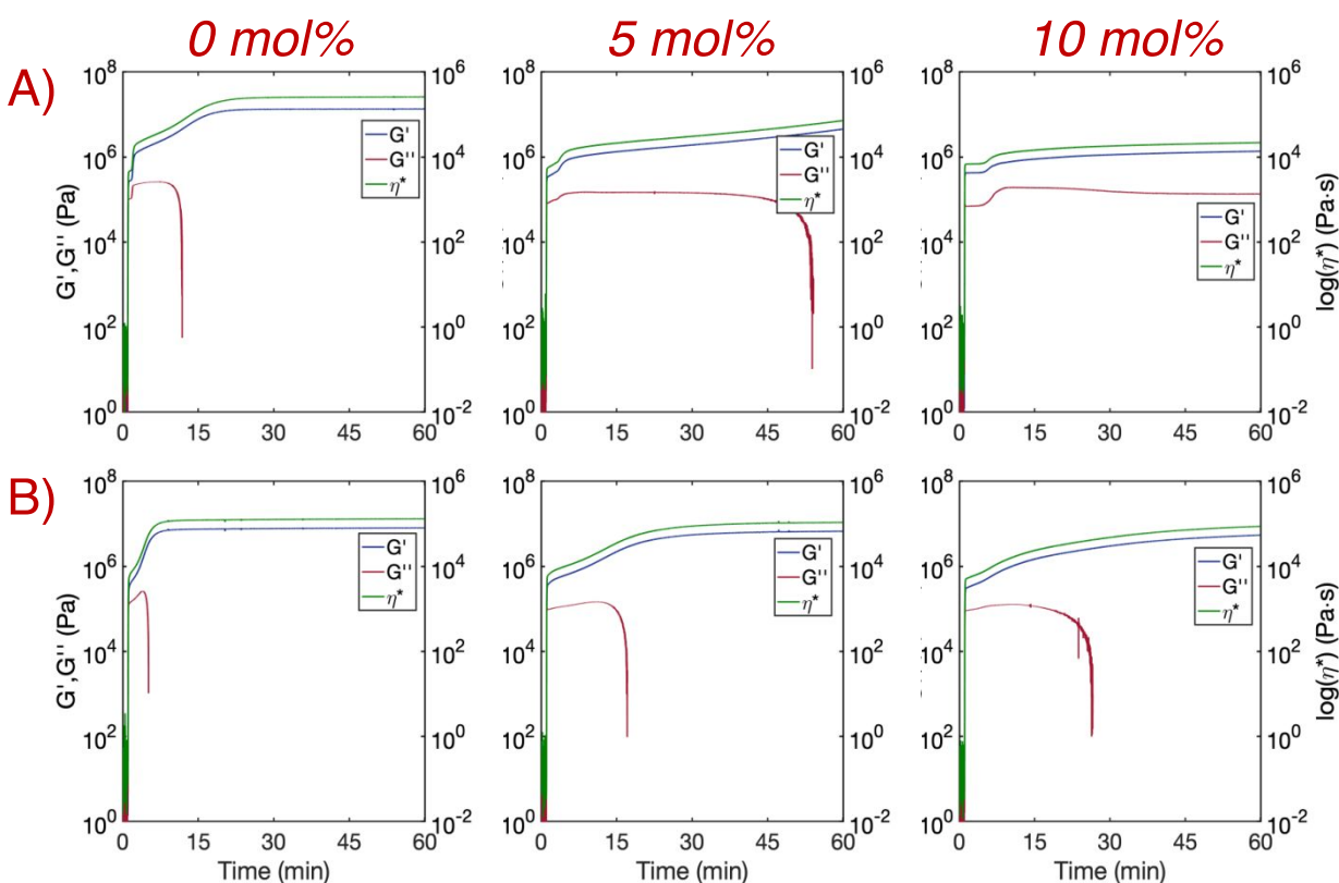
Fig. 3 Real-time photo-rheology of A) bulk and B) printing resin samples consisting of 0, 5, and 10 mol% TAT, and printing samples also contained 0.1 wt% CB. After 405 nm irradiation at 25 \text{ mW/cm}^2 for 10 s, a rapid increase in storage ( G' ) and loss ( G'' ) moduli occurs, and a successive secondary development of G' occurred during crystallization before plateauing. Similar behavior was concurrently observed for the complex viscosity ( \eta^* ). Subsequent G' and \eta^* growth post-polymerization slowed with increasing crosslinking density but significantly increased with the addition of CB.
