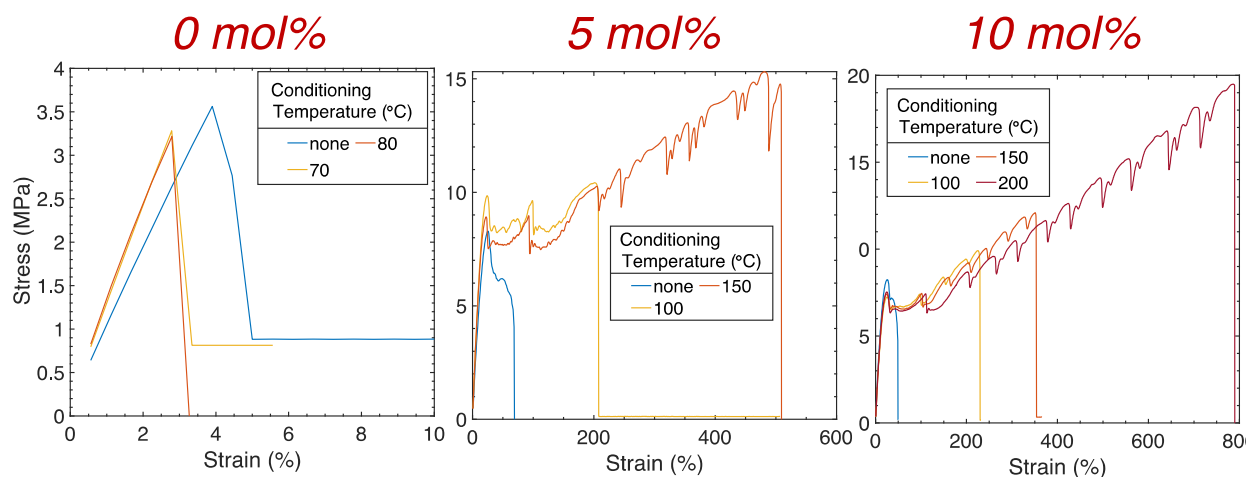
Fig. 4 Tensile stress-strain plots of samples printed with 0, 5, and 10 mol% TAT. Thermally conditioning samples without crosslinker showed no improvement in mechanical properties, whereas conditioning crosslinked samples yielded immense enhancement of print ductility. ASTM D638 Type V dogbones were printed and uniaxially strained at 5 mm min -1 .
