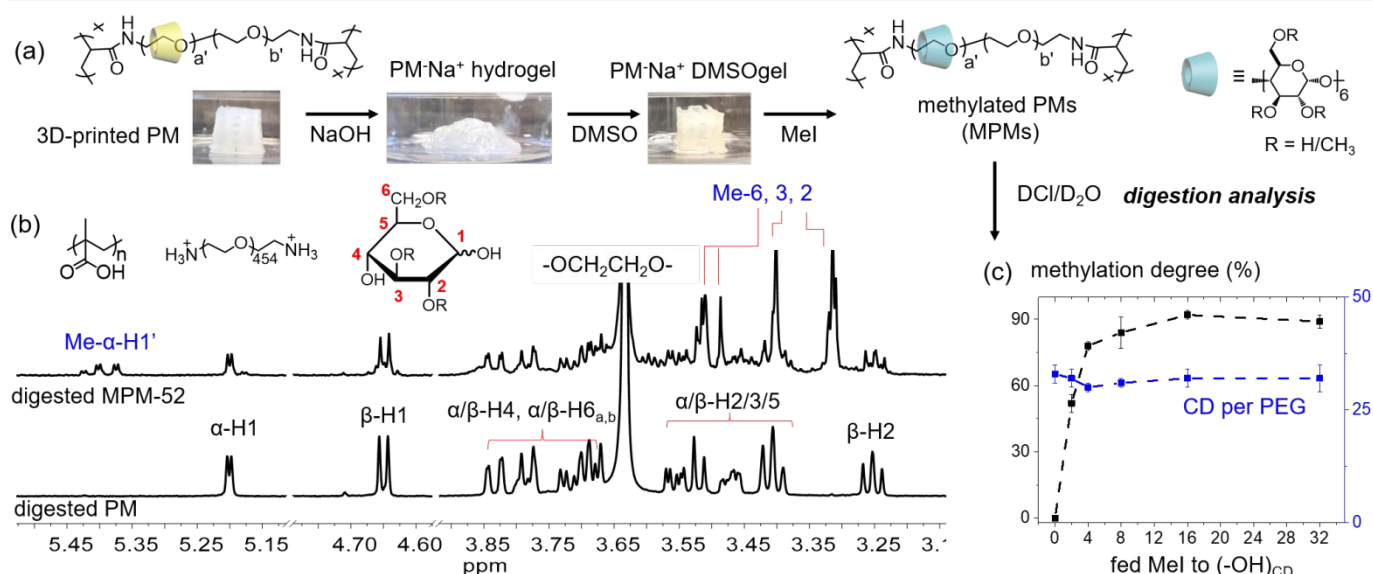
Fig. 2. (a) Post-printing synthesis of methylated polyrotaxane monoliths (MPMs) and their hydrolyzed products in DCI/D 2 O. (b) 1 H NMR spectra of the digested products of PM and MPM in DCI/D 2 O at 298 K. (c) Averaged methylation degrees (black square, calculated from three parallel experiments) of MPMs obtained through post-printing methylation with different feeding Mel ratios. The numbers of α-CDs per PEG in MPMs (blue square) were also calculated from the 1 H NMR spectra.
