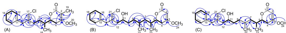
Fig. 2. Key connections determined from 2D NMR spectra for compound 1 (A), compounds 2 and 3 (B) and compound 4 (C). Bold bonds are used to show proton-proton connections determined through vicinal couplings, dashed bold bonds are used to show proton-proton connections determined through allylic and homoallylic couplings, and arrows are used to show HMBC correlations.
