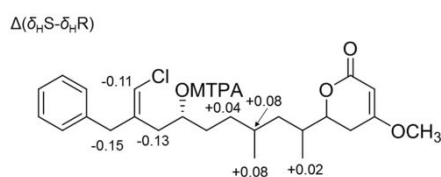
Fig. 4. \Delta(\delta_{\text{H}S}-\delta_{\text{H}R}) values determined for S - and R -MTPA esters of smenolactone C ( 3 ).
