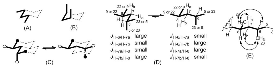
Fig. 3. (A) The most stable conformer of pentane. (B) A high-energy conformer of pentane showing the destabilizing syn -pentane interaction. (C) The two only low-energy conformers of 2,4-dimethylpentane. (D) The two only possible low-energy conformations of the C-5/C-9 segment of compound 3 . Coupling constants of H-7a and H-7b show that the conformation shown on the right is highly preferred, whatever configurations at C-6 and C-8 may be. (E) NOESY correlations of H 3 -23 with H-8 and H-7b (but not with H-7a) and of H 3 -22 with H-6 and H-7a (but not with H-7b) define relative configuration of C-6 and C-8.
