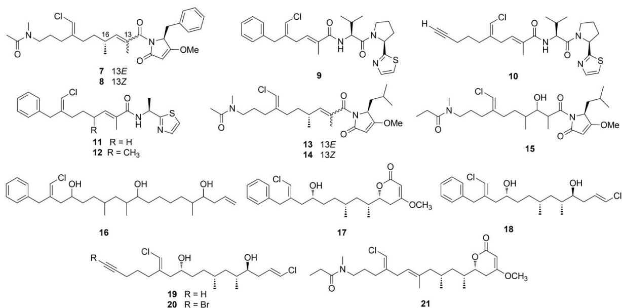
Chart 2. Structures of smenamides A ( 7 ) and B ( 8 ), smenothiazoles A ( 9 ) and B ( 10 ) and conulothiazoles A ( 11 ) and B ( 12 ) isolated from Smenospongia spp, and of smenamides C ( 13 ), D ( 14 ), and E ( 15 ) and trichophycins A-F ( 16-21 ) isolated from Trichodesmium sp.
