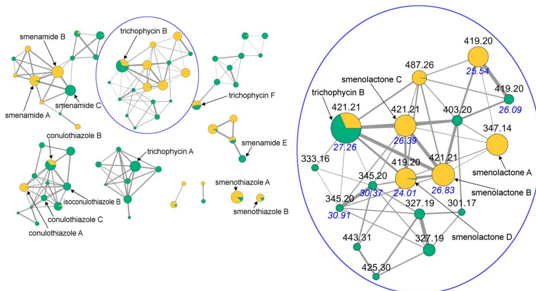
Fig. 1. The molecular network obtained combining the LC-MS/MS analyses of extracts from S. aurea and Trichodesmium sp. . Nodes are represented as a pie chart showing the source of the compound (yellow: S. aurea , green: Trichodesmium sp. ). Node size is relative to ion count, edge thickness is relative to cosine score. The networking cluster containing trichophycin B (17) and the new smenolactones A-D (1-4) is expanded, and nodes are labeled with parent m/z values and HPLC retention times. Retention times of isomeric compounds are shown in blue.
