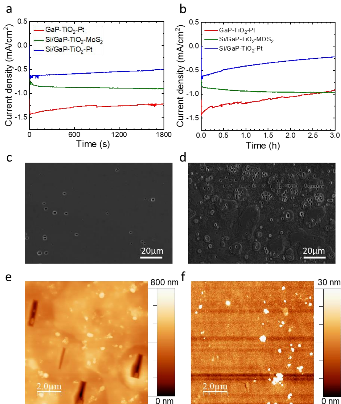
Figure 4 a. Photoelectrochemical stability measurements of a various GaP photocathodes for 30 min photocurrent density–time ( J-t ) plots held at 0 V versus RHE in in 1 M HClO 4 under one sun illumination. b. Photoelectrochemical long stability measurements of a various GaP photocathodes for 3h held at 0 V versus RHE in 1M HClO 4 under 1 sun illumination. SEM images of the photoelectrodes after reliability test (> 3h): c. Si/GaP-TiO 2 -MoS 2 and d. Si/GaP-TiO 2 -Pt (scale bar 20μm). AFM surface morphology the photoelectrodes after reliability test (> 3h): e. Si/GaP-TiO 2 -MoS 2 and f. Si/GaP-TiO 2 -Pt.
