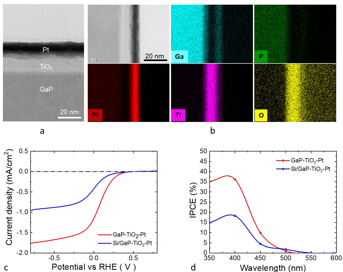
Figure 2. a. Structural, chemical profiling of the Si/GaP-TiO 2 -Pt photocathode, and PEC measurements. a. Cross-sectional STEM image Si/GaP-TiO 2 -Pt photocathode (scale bar 20 nm). b. Energy Dispersive X-ray Spectroscopy (EDS) mapping shows the individual layer thickness associated with the Ti, O, Ga, P, and Pt elements (scale bar 20 nm). c. Photocurrent density–potential ( J – V ) curves (scan rate is 50 mV s -1 ) of GaP-TiO 2 -Pt (red line) and Si/GaP-TiO 2 -Pt (blue line) photocathodes in 1 M HClO 4 under one sun illumination. d. Incident photon-to-current conversion efficiency (IPCE) of GaP-TiO 2 -Pt (red line) and Si/GaP-TiO 2 -Pt (blue line) photocathodes in 1 M HClO 4 at -0.8 V versus RHE.
