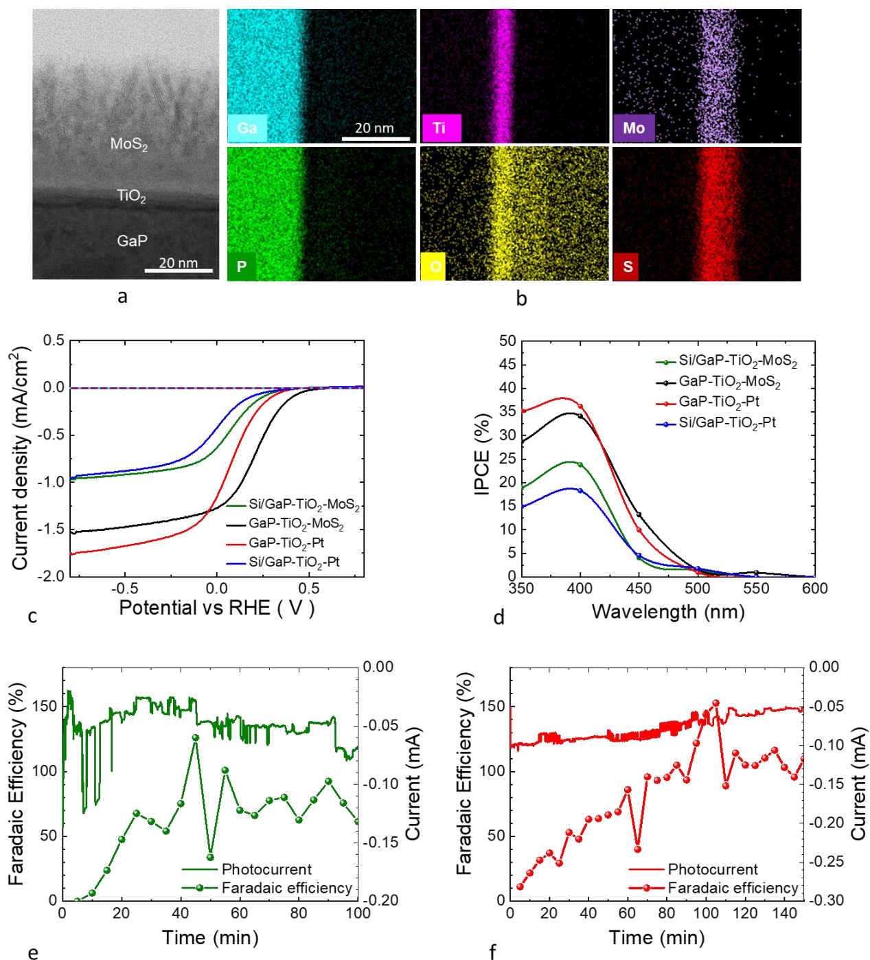
Figure 3. Structural, chemical profiling of the Si/GaP-TiO 2 -MoS 2 photocathode, and PEC measurements. a. Cross-sectional STEM image Si/GaP-TiO 2 -MoS 2 photocathode (scale bar 20 nm). b. EDS line profiling coupled with spectral component matching and the mapping shows the individual layer thickness associated with the Ti, O, Ga, P, Mo, and S elements (scale bar 20 nm). c. Photocurrent density-potential ( J - V ) curves (scan rate is 50 mV s -1 ) of GaP-TiO 2 -Pt (red line), Si/GaP-TiO 2 -Pt (blue line), Si/GaP-TiO 2 -MoS 2 (green line), and GaP-TiO 2 -MoS 2 (black line) photocathodes in 1 M HClO 4 under one sun illumination. d. Incident photon-to-current conversion efficiency (IPCE) of GaP-TiO 2 -Pt (red
