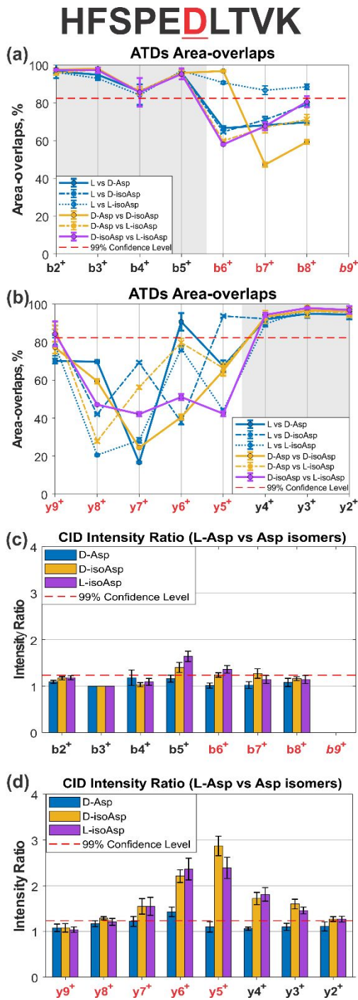
Figure 5 Result summary for Asp isomers of HFSPEDLTVK, L-Asp vs D-Asp (blue), D-isoAsp (yellow), or L-isoAsp (purple). ATD area overlaps in the isomeric (a) b-ions and (b) y-ions. CID intensity ratios of the isomeric (c) b-ions and (d) y-ions.
