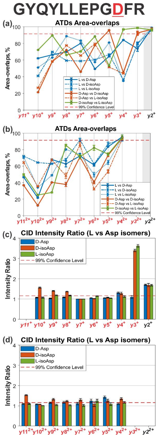
Figure 4 Results for Asp isomers of GYQYLLEPGDFR. ATD area-overlaps between L-Asp and D-Asp (blue), D-isoAsp (orange), or L-isoAsp (green) for (a) singly charged y-ions and (b) doubly charged y-ions. CID intensity ratios of the isomeric (c) singly charged y-ions and (d) doubly charged y-ions.
