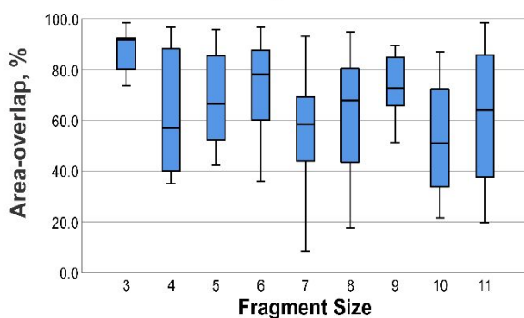
31 (b) ATDs Area-overlaps vs Fragment Sizes
