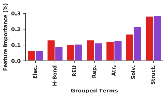
Fig. 3 Important features in GBT models derived from REF2015 (red) and BETA_Nov16 (purple). Feature importance (%) determined as described in ESI.
