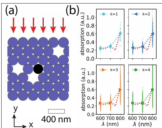
Figure 1 – (a) Schematic geometry of a 2D omission glass. A GaAs cylinder absorber (black) is surrounded by a lattice of n = 41 \text{SiO}_2 cylinders (blue). For this specific example, three cylinders have been omitted from the structure, or k = 3 . Illumination is incident from above (red arrows), with the polarization vector parallel to the cylindrical axis. For FDTD simulations, the geometry has periodic boundary conditions along the x -direction. (b) Integrated absorption spectra for k = 1-4 computed from the complete set of ensemble configurations. The dots represent the integrated absorption for each configuration in the ensemble to show the intrinsic physical variance in the ensemble. The k = 0 absorption spectrum (dashed red line) is plotted for comparison in each panel.
