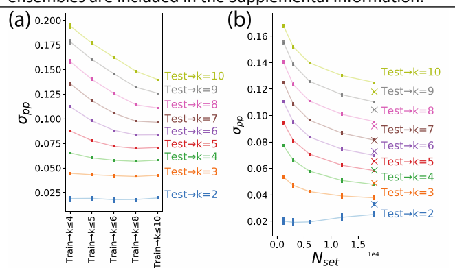
Figure 3 – (a) \sigma_{pp} measurements for MLP emulators trained on with a fixed number of samples ( N_{set} = 3000 ) with varying distribution (described in text) across the ensembles in a library of \lambda = 600 nm FDTD simulations. No simulations from the k = 7 or k = 9 ensembles were included in the training set but were included as a test set. Each line represents the \sigma_{pp} measurement averaged over eight unique models. The solid bars represent the standard deviation of measurements. (b) \sigma_{pp} measurements for MLP emulators (solid lines) trained on the ' k \leq 10 ' training set as a function of N_{set} . \sigma_{pp} was also calculated for varied contributions from each ensemble. The 'X' data represents \sigma_{pp} measurements for an emulator trained a training set of simulations skewed towards high k -values, consisting of the entire k = 0-2 ensembles, 500 simulations from k = 3 , 500 from k = 4 , 2500 from k = 5 , 2500 from k = 6 , 6000 from k = 8 , and 6000 from k = 10 .
