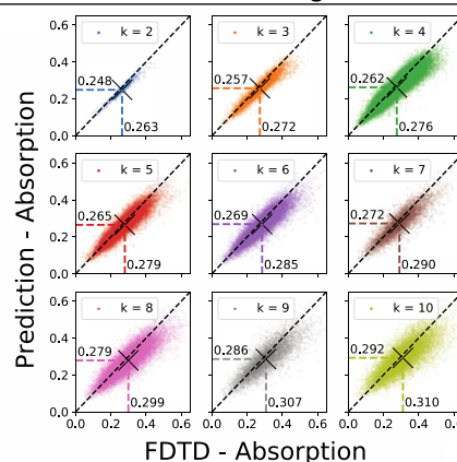
Figure 4 - Scatter plots showing the distribution of integrated absorption values ( \lambda = 600 nm) for each of the test data configurations, using an emulator trained on a training set consisting of the k = 0-2 ensembles, 500 simulations from k = 3 , 500 from k = 4 , 2500 from k = 5 , 2500 from k = 6 , 6000 from k = 8 , and 6000 from k = 10 . For each configuration in the ensemble, the x-coordinate of the point represents the FDTD-derived absorption for the configuration while the y-coordinate represents the MLP-predicted absorption. The black 'X' in each plot indicates the average of the predicted (y-coordinate) and the FDTD-determined true (x-coordinate) absorption for that ensemble.
