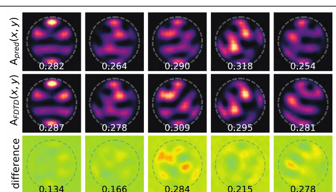
Figure 2 – Randomly chosen examples of the MLP-predicted profile A_{\text{pred}} , the corresponding true profile A_{\text{FDTD}} , and the difference between the two profiles (difference). The integrated absorption ( \lambda = 600 nm) for each profile is included at the bottom of each panel. The \sigma_{\text{pp}} metric for each pair is included at the bottom of the difference panel.
