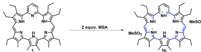
Figure 2. Addition of 2 equivalents of methanesulfonic acid (MSA) yields the diprotonated anti-aromatic species 1b .
