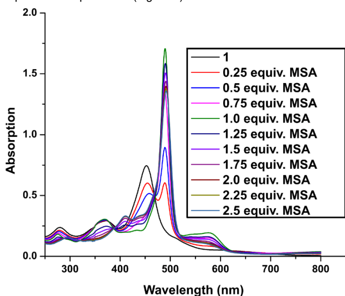
Figure 3. UV-Vis spectral titration of 1 with MSA in \text{CHCl}_3 . The red shift in the Soret-like band and the appearance of Q-type features was taken as initial evidence of extended \pi -conjugation.
