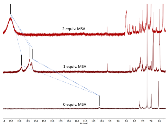
Figure 4. NMR spectral titration of 1 in \text{CDCl}_3 with \text{MSA-}d_4 . The downfield shift in the pyrrole NH resonance seen upon diprotonation is taken as evidence for conversion to an antiaromatic form.
