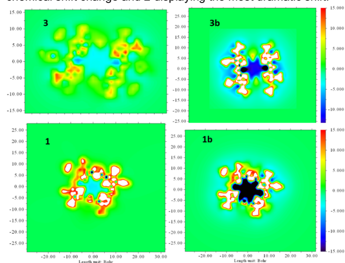
Figure 6. Iso-chemical surface shielding (ICSS) of pyriamethyrin 1 and 3 , dipyriamethyrin and their protonated forms. Green regions indicate non-aromatic, blue-black indicate antiaromaticity, and red indicates aromaticity.
