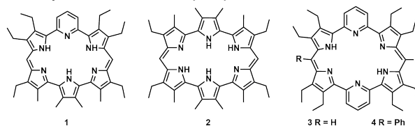
Figure 1. Chemical structures of pyriamethyrin ( 1 ), amethyrin ( 2 ), and the dipyriamethyrins ( 3 and 4 ) considered in the present study.
