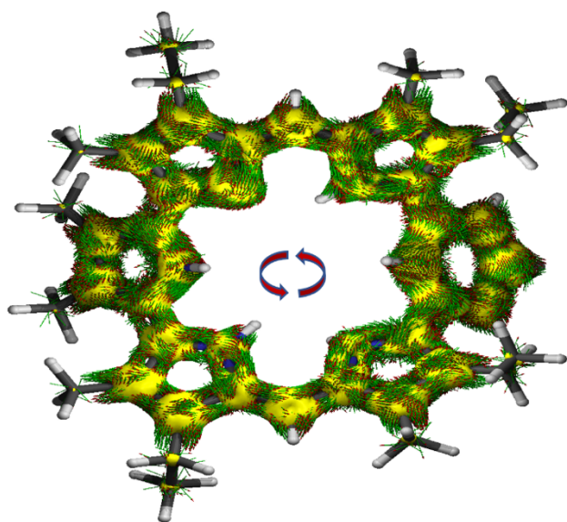
Figure 5. Calculated anisotropy induced current density (ACID) plot for diprotonated pyriamethyrin 1b . Current density vectors associated with a global counter-clockwise current are seen, as would be expected for an anti-aromatic compound.
