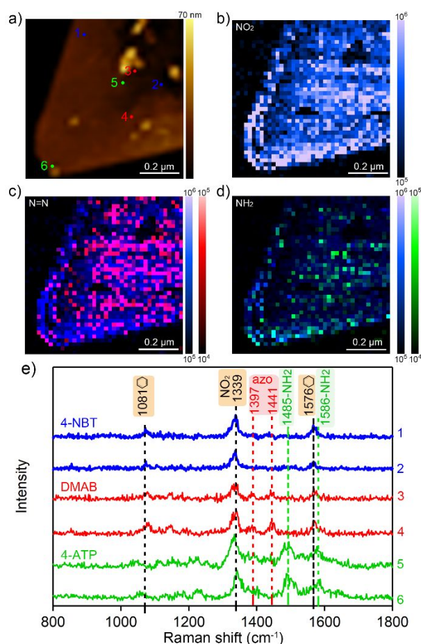
Fig. 1 (a) AFM image of WAu@PdMPs. (b) TERS image of NO 2 on WAu@PdMPs (20 nm per pixel). Overlapping TERS image of NO 2 vibration with (c) DMAB (d) 4-ATP vibration on WAu@PdMPs. Intensity of 1339 \text{cm}^{-1} band (NO 2 ) of 4-NBT is shown in blue, intensities of 1397 and 1441 \text{cm}^{-1} (azo) of DMAB is shown in red, intensities of 1485 \text{cm}^{-1} (NH 2 ) is shown in green. (e) Typical TERS spectra randomly picked up from chemical maps on (b-d) showing presence of 4-NBT (blue), DMAB (red) and NH 2 in green, which have been labeled in Fig. 1(a) and (e).
