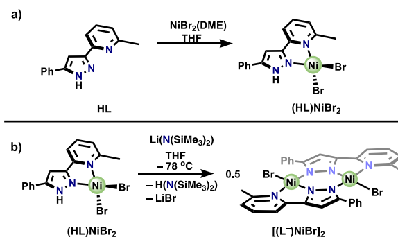
Scheme 3. a) Synthesis of (HL)NiBr_2 and b) dehydrohalogenation of (HL)NiBr_2 to form [(L^-)NiBr]_2
