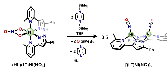
Scheme 2. Balanced reaction for formation of [(L)Ni(NO)]_2
