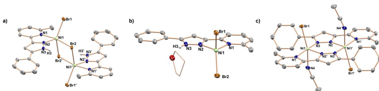
Figure 4. Molecular structure (50% probability ellipsoids) showing selected structural parameters of a) [(HL)NiBr_2]_2 : Br2-Ni1, 2.4849(3); Br2-Ni1', 2.5506(3); Br1-Ni1, 2.4235(3); Ni1-N1, 2.1005(15); Ni1-N2, 1.9834(15); Br1-Ni1-Br2, 140.284(11); N1-Ni1-Br2', 167.61(4), b) (HL)NiBr_2 : Br1-Ni1, 2.3527(4); Br2-Ni1, 2.3552(4); Ni1-N1, 2.019(2); Ni1-N2, 1.983(2); Br1-Ni1-Br2, 129.928(17); N1-Ni1-Br1, 111.51(6); N1-Ni1-Br2, 106.35(6); N2-Ni1-Br1, 108.79(7); N2-Ni1-Br2, 108.24(6), c) [(L^-)Ni(Br)(MeCN)]_2 : Br1-Ni1, 2.4888(3); Ni1-N2, 1.9851(17); Ni1-N3', 2.0067(18); Ni1-N1, 2.0800(18); Ni1-N4, 2.0997(19); N4-Ni1-Br1, 164.16(6); N3'-Ni1-N1, 173.71.
