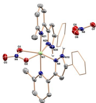
Figure 1. Molecular structure (50% probability ellipsoids) of [(HL)(L)Ni(NO_3)]NO_3 showing selected atom labelling; unlabelled atoms are carbon. All protons except pyrazole NH protons have been removed for clarity. Ni1-O2, 2.1364(16) Å; Ni1-O1, 2.1545(17); Ni1-N21, 2.1473(17); Ni1-N29, 2.0176(18); Ni1-N9, 2.0197(18); Ni1-N1, 2.1260(18).
