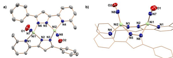
Figure 3. Molecular structure (50% probability ellipsoids) of [(L)Ni(NO)]_2 showing a) top view of the non-hydrogen atoms and b) side-on view with selected structural parameters: Ni1-N2, 1.9840(16); Ni1-N1, 2.0737(18); Ni1-N6, 2.0040(17); Ni1-N7, 1.6470(19); N7-O1, 1.164(3); O1-N7-Ni1, 165.72(19).
