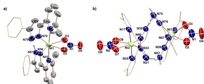
Figure 2. a) Molecular structure (50% probability ellipsoids) of one molecule of (HL)(L)Ni(NO_3) , showing selected atom labelling; only the NH proton is shown (on N57). Selected structural parameters: Ni1-O2, 2.115(6) Å; Ni1-O3, 2.211(6); Ni1-N53, 2.143(7); Ni1-N58, 2.060(7); Ni1-N67, 2.125(8); Ni1-N76, 2.000(8); O2-N1, 1.270(10); O3-N1, 1.296(10); O4-N1, 1.210(9); values for the second crystallographically independent Ni show no notable deviations from these and b) View of the [(HL)(L)Ni(NO_3)]_2 dimer. Hydrogen bonds are shown with dashed lines. Phenyl groups are shown as wireframe.
