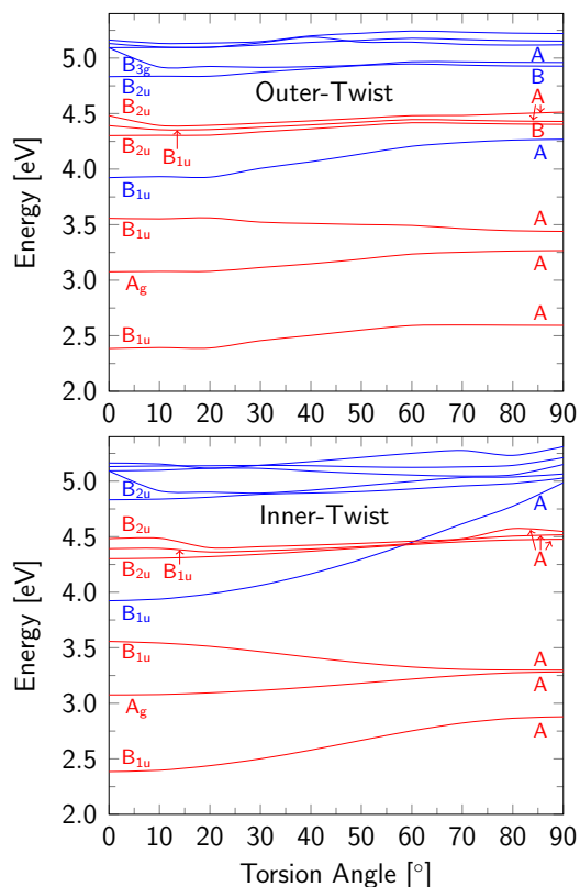
Fig. 6 Potential energy surfaces of excited singlet (blue) and triplet (red) states along the relaxed ground-state scan of side-twisted (top) and mid-twisted (bottom) BPEB-HH at the TDDFT/CAM-B3LYP/def2-TZVP level. The energy is given relative to the ground state in its planar equilibrium geometry, respectively. The states are labeled according to the D_{2h} point group on the left, and according to the C_2 point group on the right.
