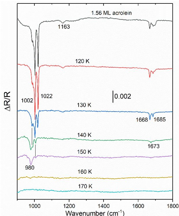
Fig. 3 RAIR spectra of 1.56 ML acrolein adsorbed on Ag(111) at 85 K (black). The surface was annealed to the indicated temperature for one minute and re-cooled to 85 K.
