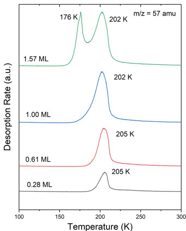
Fig. 8. TPD spectra of 2-propenol adsorbed on Ag(111) at 85 K with increasing coverage.
