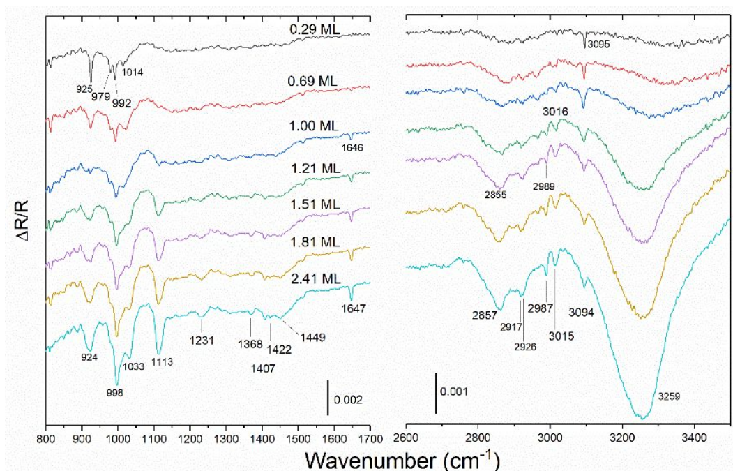
Fig. 7. RAIR spectra of 2-propenol adsorbed on Ag(111) at 85 K with increasing coverage.
