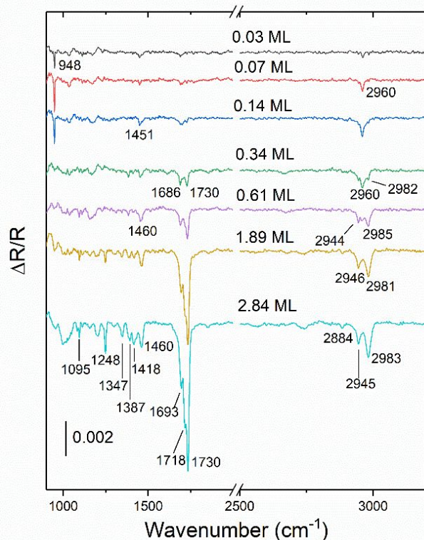
Fig. 4 RAIR spectra of propanal adsorbed on Ag(111) at 85 K with increasing coverage.
