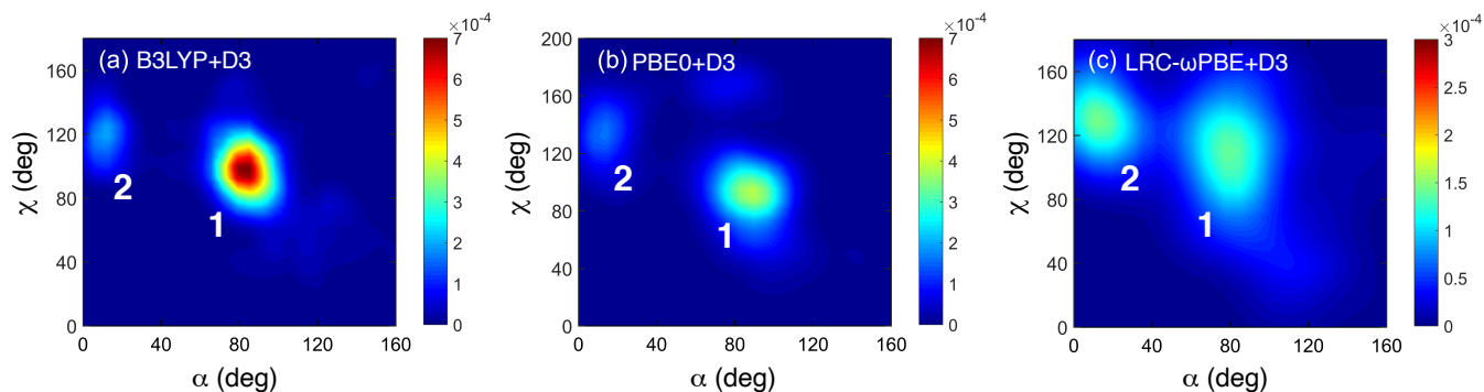
Fig. 6 Two-dimensional joint distributions of \alpha and \chi (as defined in Fig. 1), for simulations using (a) B3LYP+D3, (b) PBE0+D3, and (c) LRC- \omega PBE+D3. The two prominent features are labeled "1" and "2" for convenient reference in the text.
