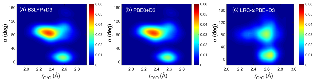
Fig. 5 Two-dimensional joint distributions of r_{\text{O}^*\text{O}} and \alpha , for simulations using (a) B3LYP+D3, (b) PBE0+D3, and (c) LRC- \omega PBE+D3. These geometrical parameters are defined in Fig. 1.
