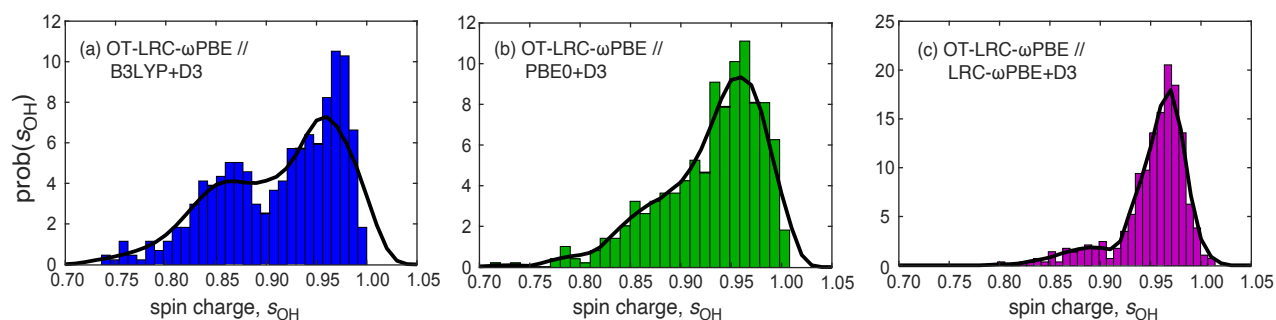
Fig. 7 Histograms for the total spin charge s_{\text{OH}} on the \cdot\text{OH} moiety, for simulations performed using (a) B3LYP+D3, (b) PBE0+D3, and (c) LRC- \omega PBE+D3. The spin charges are computed at the OT-LRC- \omega PBE+D3/6-31+G* level, with \omega tuned separately for each simulation. Black curves are fits to the distribution, which can be interpreted as probability distributions for s_{\text{OH}} .
