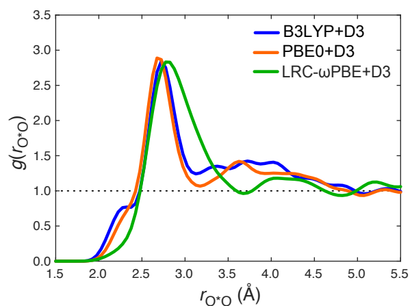
Fig. 2 Comparison of RDFs g(r_{O^*O}) for ^*OH(aq) , where O^* indicates the hydroxyl oxygen. Results were obtained from QM/MM simulations using three different density functionals.
