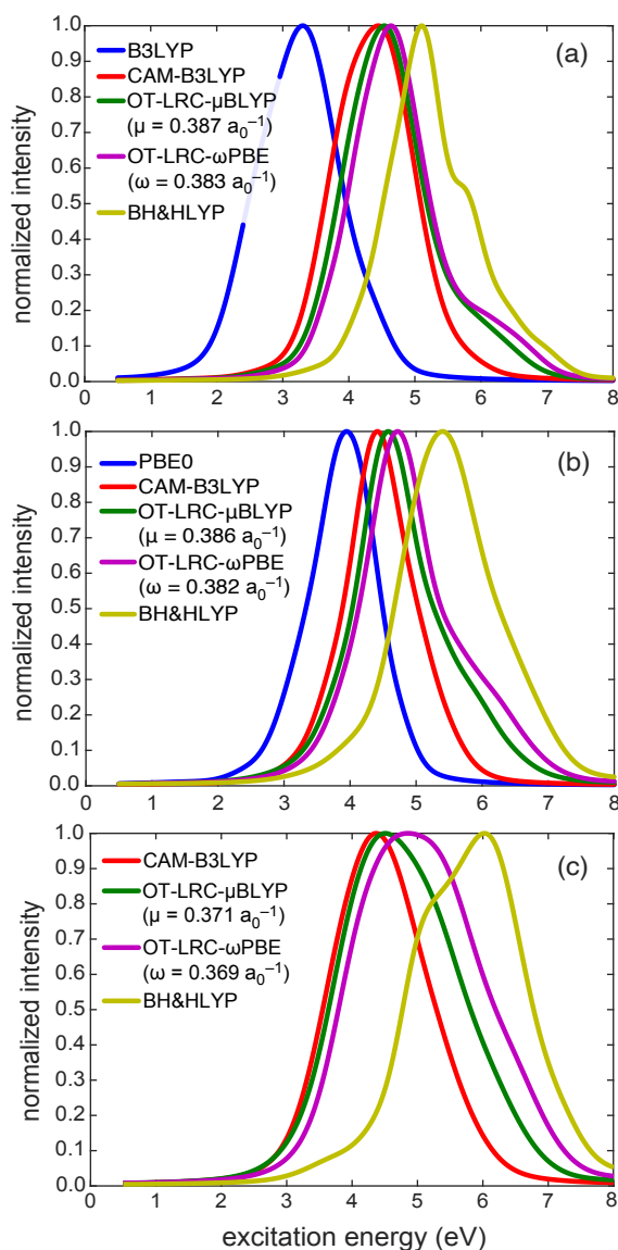
Fig. 8 Ensemble-averaged absorption spectra for \cdot\text{OH}(\text{aq}) computed using TD-DFT with various functionals as indicated, for QM/MM trajectory data obtained from (a) B3LYP+D3, (b) PBE0+D3, or (c) LRC- \omega PBE+D3 simulations.
