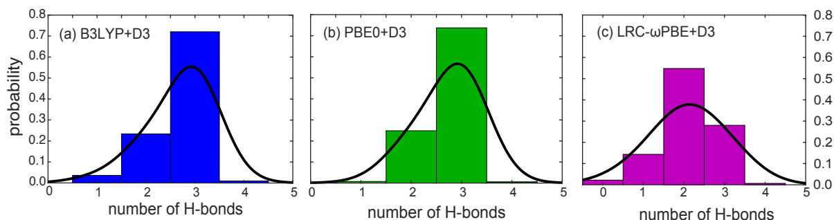
Fig. 4 Histograms for the number of hydrogen bonds to \cdot\text{OH} , considering the nearest five water molecules to the radical, for simulations performed using (a) B3LYP+D3, (b) PBE0+D3, and (c) LRC- \omega PBE+D3. Black curves are fits to the normalized probability distributions.
