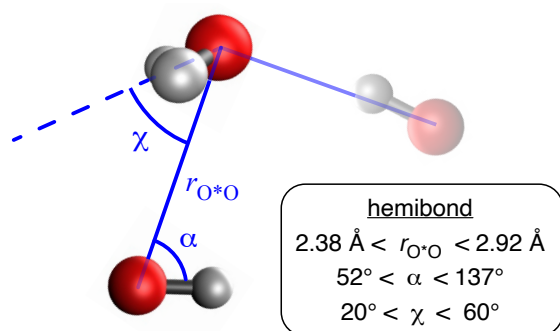
Fig. 1 Schematic view of the hemibonded \text{H}_2\text{O} \cdots \cdot\text{OH} complex (opaque models) along with a translucent hydroxyl radical in a hydrogen-bonded orientation. Quantitative suggestions for the geometrical parameters that define the hemibonded structure are taken from Ref. 30.
