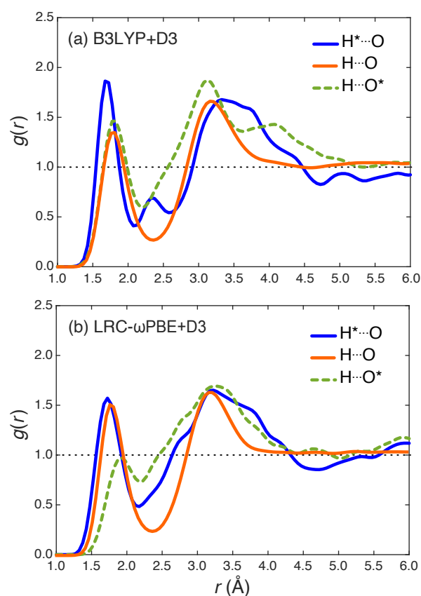
Fig. 3 Comparison of different oxygen–hydrogen RDFs obtained from (a) B3LYP+D3 versus (b) LRC- \omega PBE+D3 simulations. Covalent bonds have been excluded from the averaging so that g(r_{OH}) represents the RDF for hydrogen bonds only.
