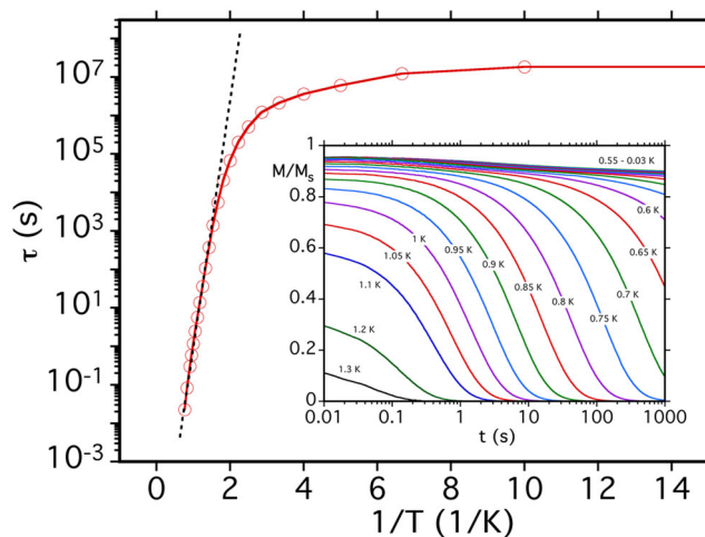
Figure 7. Relaxation time ( \tau ) vs. 1/T plot for a single crystal of 3\cdot 3\text{py}\cdot 12\text{CH}_2\text{Cl}_2 obtained from the dc magnetization decay vs. time data in zero applied field at the indicated temperatures shown in the inset. The dashed line is the fit of the thermally-activated region to the Arrhenius equation. See the text for the fit parameters.
