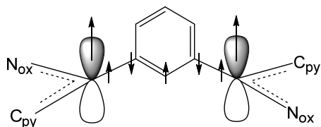
Figure 11. The proposed contribution to the inter-Mn 3 ferromagnetic coupling by spin polarization of \sigma -bonding electrons to the central 1,3-phenylene unit of the 1,3-ppmd 2 linker by the spin density in the orthogonal \pi -system. N ox = oximate N atom; C py = 2-C atom of the pyridine ring.
