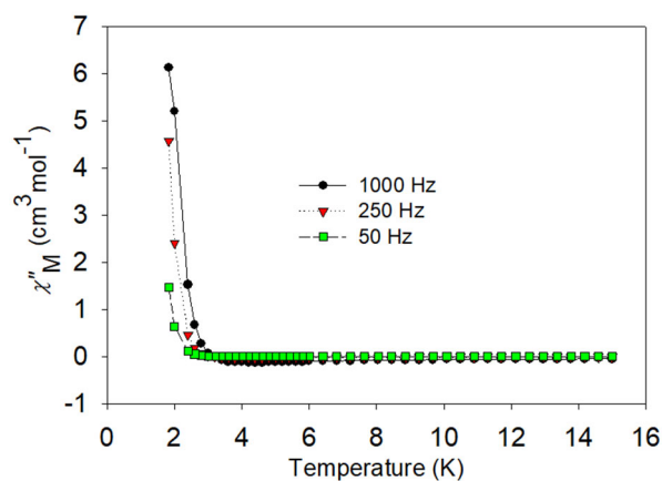
Figure 5. Plots of the (top) in-phase ( \chi'_M , as \chi'_MT ) and (bottom) out-of-phase ( \chi''_M ) ac susceptibility data vs. T for 3\cdot 6\text{H}_2\text{O} in a 3.5 G field at the indicated oscillation frequencies.
