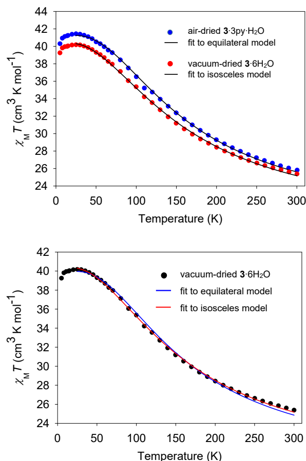
Figure 3. (top) \chi_M T per [\text{Mn}_3]_2 dimer vs. T for air-dried 3 ·3py·H 2 O and vacuum-dried 3 ·6H 2 O samples in a 0.1 T dc field. The solid lines are the fits of the 25–300 K data to equilateral (single J ) and isosceles (two J 's) models. See the text for the fit parameters. (bottom) Comparison of the fits of \chi_M T per [\text{Mn}_3]_2 dimer vs. T data for vacuum-dried 3 ·6H 2 O to an equilateral vs. an isosceles triangle model. See the text for the fit parameters.
