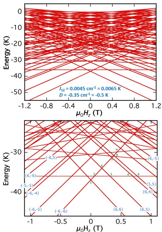
Figure 8. (Top) Spin state energies vs. applied dc field plot for 3-3py-12CH 2 Cl 2 constructed with J = +4.5 \times 10^{-3} \text{ cm}^{-1} ( \hat{H} = -2J_{12}\hat{S}_1 \cdot \hat{S}_2 convention) and D = -0.35 \text{ cm}^{-1} to simulate the positions of the avoided level crossings that lead to the experimentally observed QTM step positions in the hysteresis loops of Fig. 6. (Bottom) Expansion showing only the lower energy spin states populated at very low temperature, and the avoided level crossings relevant to the hysteresis loops in Fig. 6 when the field is swept from -1.2 T to +1.2 T. The green numbers 1 to 9 are the crossings listed in Table 3. Spin states are labelled in blue as (m_{S1}, m_{S2}) for the two \text{Mn}_3 units. See the text for the discussion of the avoided level crossings leading to the observed QTM steps in Fig. 6.
