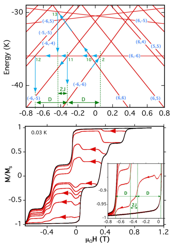
Figure 9. (Top) Portion of the spin state energy plot of Fig. 8, bottom, showing the minor loop strategy of scanning the dc field from -1 T to past crossing 2 and then reversing the scan (blue chevrons). Avoided level crossings 10 to 13 are those listed in Table 3 that should lead to QTM steps. Blue arrows show thermal relaxations after QTM from the generated excited states. Green arrows show the targeted field separations between QTM steps to obtain J ( = J_{12} ) and D . (Bottom) Experimental minor loop scans at 0.03 K and a 0.14 T/s dc field sweep rate showing the targeted QTM steps. The inset shows the clear observation of the QTM steps resulting from the avoided level crossings 2 and 11 to 13 , and the measurement of the \Delta H used to obtain J_{12} and D ; see the text for details.
