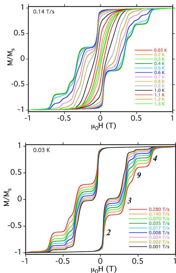
Figure 6. Magnetization ( M ) vs. dc field hysteresis loops for a single crystal of 3\cdot 3\text{py}\cdot 12\text{CH}_2\text{Cl}_2 ( top ) at the indicated temperatures at a 0.14 T/s field scan rate, and ( bottom ) at the indicated scan rates at 0.03 K. M is normalized to its saturation value, M_s . The step labels in the bottom figure refer to the QTM transitions in Table 3.
