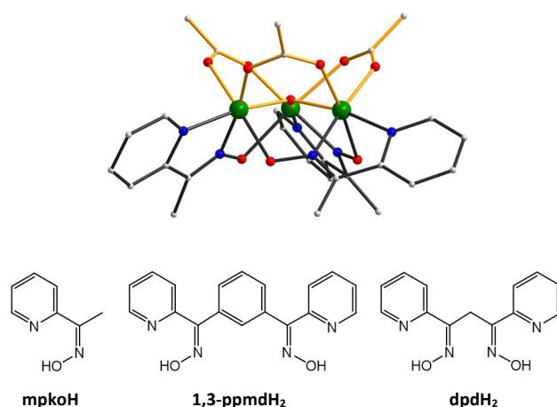
Figure 1. (top) Structure of the cation of monomer 2 viewed along the \text{Mn}_3 plane showing the tripodal arrangement of the three acetate and three mpko groups. Colour code: Mn, green; N, blue; O, red; C, gray. (bottom) Structures of mpkoH, 1,3-ppmdH 2 and dpdH 2 .
