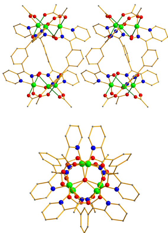
Figure 2. Complete cation of 3 viewed ( top ) as a stereopair almost along a C_2 symmetry axis, with the JT axes indicated as green bonds, and ( bottom ) along the C_3 axis. Colour code: Mn, green; N, blue; O, red; C, grey. Hydrogen atoms have been omitted for clarity.
