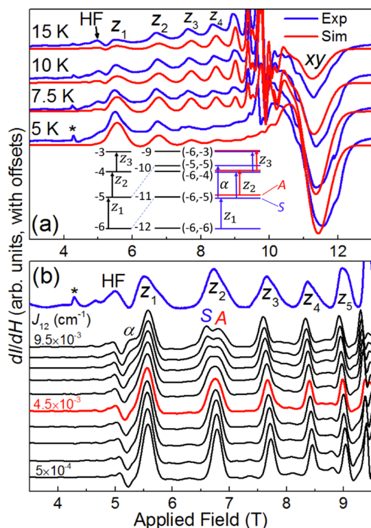
Figure 10. (a) Experimental (Exp) and simulated (Sim) powder HFEPR spectra of 3:3py·H 2 O at a frequency of 270 GHz, plotted as dI/dH ( I = transmitted intensity) for temperatures in the range from 5 to 15 K. The resonances labeled z_1 to z_4 correspond to the parallel ( z -) components of the powder pattern, xy correspond to the perpendicular components, and HF is a half field transition (see main text for explanation); the feature labeled with an asterisk (*) corresponds to a known O 2 impurity in the sample holder. The inset schematically depicts the lowest lying energy levels appropriate to the parallel resonances. On the left are the uncoupled states associated with each individual S = 6 Mn 3 SMM, labeled according to m_S value, with the \Delta m_S = +1 transitions corresponding to resonances z_1 to z_3 labeled. The middle panel shows the levels associated with the uncoupled dimer, labeled according to M = m_{S1} + m_{S2} ; as can be seen, the new states are generated simply by exciting one of the spins, thereby translating (dashed lines) the overall energy of the dimer accordingly. The right panel depicts the fully coupled energy levels, labeled according to (m_{S1}, m_{S2}) , where the blue and red states respectively correspond to the symmetric (S) and antisymmetric (A) combinations of |m_{S1}, m_{S2}\rangle and |m_{S2}, m_{S1}\rangle . (b) Simulations of the 10 K spectrum as a function of the exchange coupling parameter, J_{12} (in steps of 10^{-3} cm -1 , see legend). The linewidth is reduced from the best simulations in (a) so that it is possible to resolve additional resonances that emerge due to the exchange coupling, i.e., \alpha and the S and A z_2 resonances. The red simulated spectrum corresponds to the value of J_{12} deduced from magnetic hysteresis experiments and the value used for the simulations in (a).
