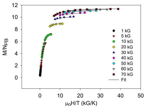
Figure 4. Magnetization ( M ) per \text{Mn}_3 unit of 3\cdot 6\text{H}_2\text{O} plotted as M/N\mu_B vs. \mu_0H/T . Solid lines are the fit of the data; see the text for the fit parameters.
