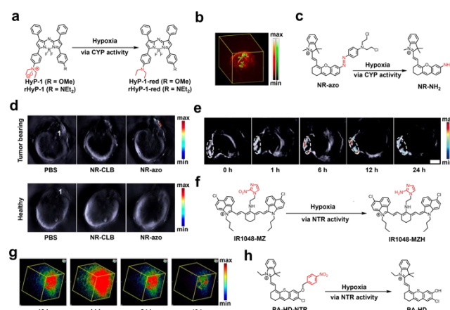
Figure 25. a) Reaction of HyP-1/rHyP-1 via CYP activity under hypoxic conditions. b) 3D PA imaging of 4T1 tumor using rHyP-1 to reveal hypoxic domains in green. c) Reaction of NR-azo via CYP activity under hypoxic conditions. d) PA images of tumor bearing mice and healthy mice at 0.5 hour after intratumoral injection of PBS, NR-CLB or NR-azo. e) PA images of tumor bearing mice before and at various time points after injection of Lipo-NR-azo. f) Reaction of IR1048-MZ via NTR activity under hypoxic conditions. g) PA images in A549 tumor-bearing BALB/c nude mice before and at various time points after injection of IR1048-MZ. h) Reaction of PA-HD-NTR via NTR activity under hypoxic conditions. b) is reproduced from ref. 311 with permission from American Chemical Society, Copyright 2018. d) and e) are reproduced from ref. 317, which is an open-access article distributed under the Creative Commons Attribution (CC BY-NC) License, 2019 Ivyspring International Publisher. g) is reproduced from ref. 329 with permission from John Wiley and Sons, Copyright 2021.
