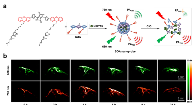
Figure 19. a) Schematic of the synthesis of SOA NPs. b) PA images of subcutaneous 4T1 xenograft tumors before and at various time points after the injection of SOA nanoprobe under 680 nm or 780 nm laser irradiation. a) and b) are reproduced from ref. 249 with permission from American Chemical Society, Copyright 2017.
