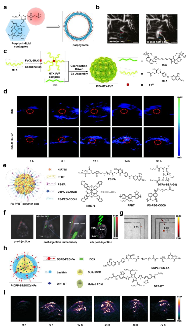
Figure 7. a) Schematic of porphysomes. b) PA images before and 15 mins after injection with porphysomes, showing secondary lymph vessels, lymph node, and inflowing lymph vessels. c) Schematic of synthesis of ICG-MTX-Fe III . d) PA images in HeLa tumor-bearing mice before and at various time points after injection of ICG or ICG-MTX-Fe III . e) Schematic of FA-PFBT polymer dots. f) PA images of the lymph vessel, T-SC, and T-PO in the NCI-H292 tumor-bearing mice before and immediately after injection of FA-PFBT polymer dots. g) Ex vivo fluorescence imaging of T-SC, T-IN and T-PO lymph nodes. h) Schematic of P(DPP-BT/DOX) NPs. i) PA images in HeLa tumor-bearing mice before and at various time points after injection of P(DPP-BT/DOX) NPs. a) and b) are reproduced from ref. 82 with permission from Springer Nature, Copyright 2011. c) and d) are reproduced from ref. 97 with permission from Royal Society of Chemistry, Copyright 2020. e), f) and g) are reproduced from ref. 91 with permission from John Wiley and Sons, Copyright 2018. h) and i) are reproduced from ref. 95 with permission from John Wiley and Sons, Copyright 2019.
