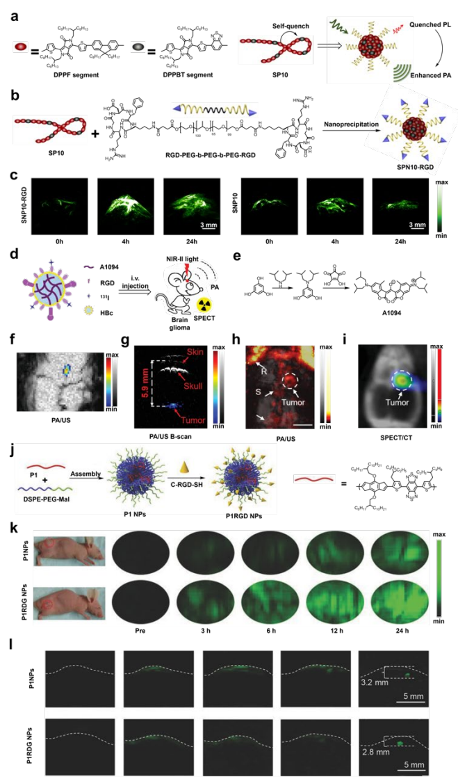
Figure 9. a) and b) Schematic of the synthesis of SNP10-RGD. c) PA images of murine 4T1 breast tumors before and at various time points after injection of SNP10-RGD or SNP10. d) Schematic of A1094@RGD-HBc. e) Synthesis of A1094 f) PA/US images of U87MG
