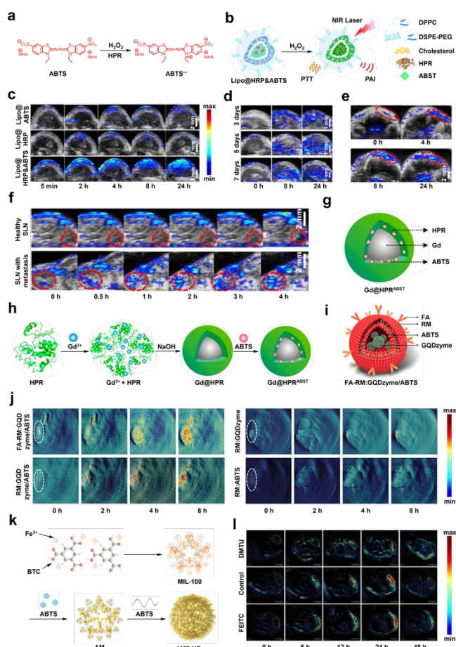
Figure 18. a) Reaction of ABTS under HPR-catalyzed H 2 O 2 oxidation. b) Schematic of the reaction of Lipo@HRP&ABTS with H 2 O 2 . c) PA images of the 4T1 tumors before and at various time
