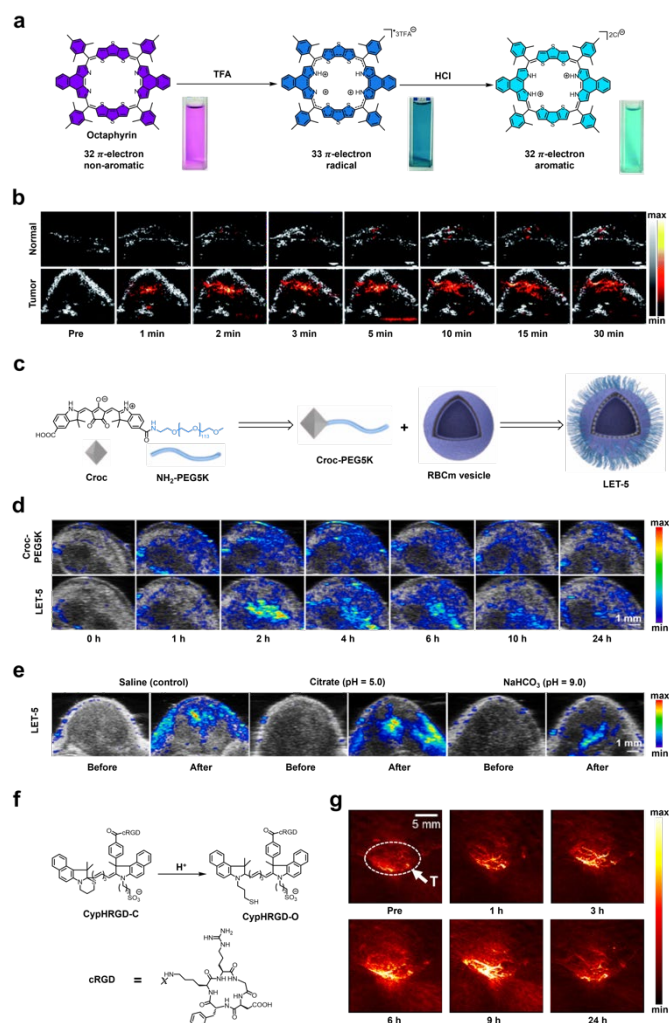
Figure 26. a) Reaction of octaphyrin under acidic conditions. b) PA/US B-scan image of BALB/c nude mice and HepG2-tumor bearing mice before and at various time points after injection of OctaNPs. c) Schematic of the synthesis of LET-5. d) PA images in 4T1 tumor-bearing mice before and at various time points after injection of Croc-PEG5K or LET-5. e) PA images of 4T1 tumor before and after injection of LET-5 with pre-treatment using saline, citrate buffer or a solution of NaHCO 3 . f) Reaction of CypHRGD-C under acidic conditions. g) PA images in A549 tumor-bearing mice before and at various time points after injection of CypHRGD-C. a) and b) are reproduced from ref. 366, which is an open-access article distributed under the Creative Commons Attribution (CC BY-NC) License, 2019 Ivyspring International Publisher. c), d) and e) are reproduced from ref.
