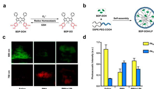
Figure 21. a) Reaction of BDP-DOH with O 2 •- and GSH. b) Schematic of the synthesis of BDP-DOH/LP. c) PA images of the EMT6 tumor (treated with saline, PMA, or PMA + LPA) after the injection of BDP-DOH/LP under 680 or 750 nm laser irradiation. d) PA intensities of the EMT6 tumor (treated with saline, PMA, or PMA + LPA) after the injection of BDP-DOH/LP under 680 or 750 nm laser irradiation. b) and c) are reproduced from ref. 264 with permission from American Chemical Society, Copyright 2019.
