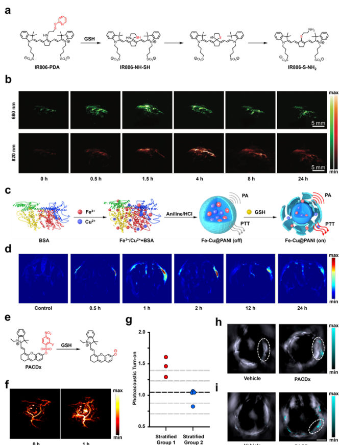
Figure 23. a) Reaction of IR806-PDA with GSH. b) PA images of xenograft HeLa tumors before and at various time points after the injection of IR806-PDA under 680 nm or 820 nm laser irradiation. c) Schematic of the synthesis of Fe-Cu@PANI. d) PA images of normal muscle (left) and xenograft 4T1 tumor (right) before and at various time points after the injection of Fe-Cu@PANI. e) Reaction of PACDx with GSH. f) PA images of the xenograft A549 tumor before and one hour after the injection of PACDx. g) Stratification based on PA fold turn-on after the injection of PACDx. h) PA images of the lung region after the injection of vehicle and PACDx in orthotopic lung cancer model. i) PA images of the liver after the injection of vehicle and PACDx in the liver metastasis model. a) and b) are reproduced from ref. 287 with permission from John Wiley and Sons, Copyright 2018. c) and d) are reproduced from ref. 288, which is an open-access article distributed under the CC BY-NC License, 2021 AAAS. e), f), g), h) and i) are reproduced from ref. 289 with permission from Springer Nature, Copyright 2021.
