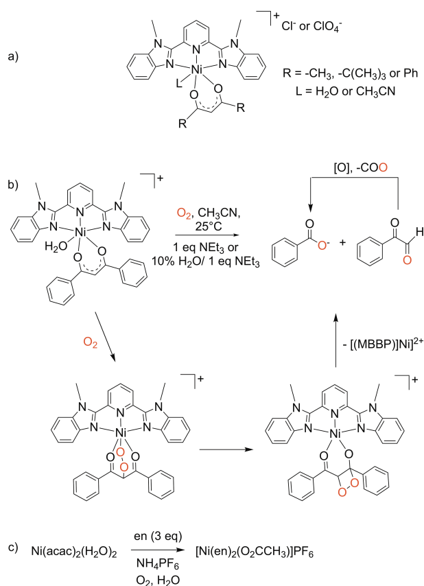
Scheme 3 a) MBBP-ligated \text{Ni}(\text{II}) diketonate complexes reported by Ramasubramanian, et al. 24 b) Proposed pathway of \text{O}_2 reaction of MBBP-ligated \text{Ni}(\text{II}) phenyl diketonate complex. c) Oxidative cleavage of an acetylacetonate ligand. 25
