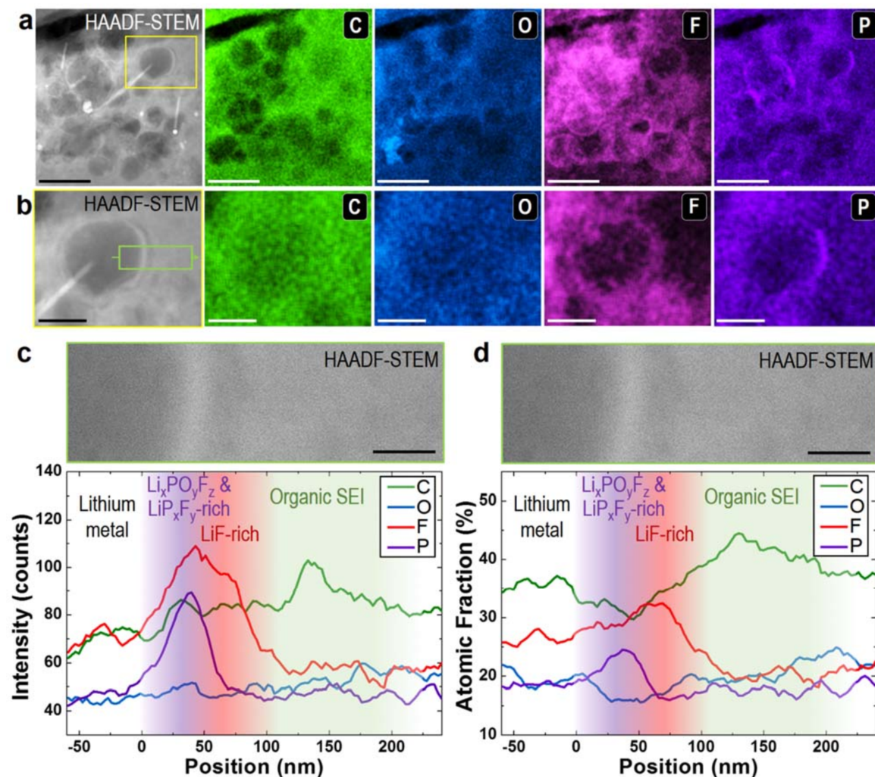
Fig. 4. Scanning TEM (STEM) energy-dispersive x-ray spectroscopy (EDS) analysis of SEI on lithium nanogranules in the presence of PDDA cationic polymer coating. (a) A high-angle annular dark-field (HAADF) STEM image and EDS elemental maps of lithium nanogranules and their SEI layers. Scale bars are 500 nm. (b) A magnified HAADF-STEM image and corresponding EDS elemental maps of a representative lithium nanogranule. The corresponding area is marked with a yellow box in the HAADF-STEM image in (a). Scale bars are 200 nm. (c, d) EDS line-scan profiles of the lithium nanogranule surface corresponding to the marked region in (b), where both intensity (c) and atomic fraction (d) are obtained. Each point was integrated with a window of 100 pixels \times 3 pixels (96.8 nm perpendicular and 2.9 nm parallel to the scanning line) to enhance EDS signals. The corresponding HAADF-STEM image is shown above each profile for better understanding. Scale bars are 50 nm.
