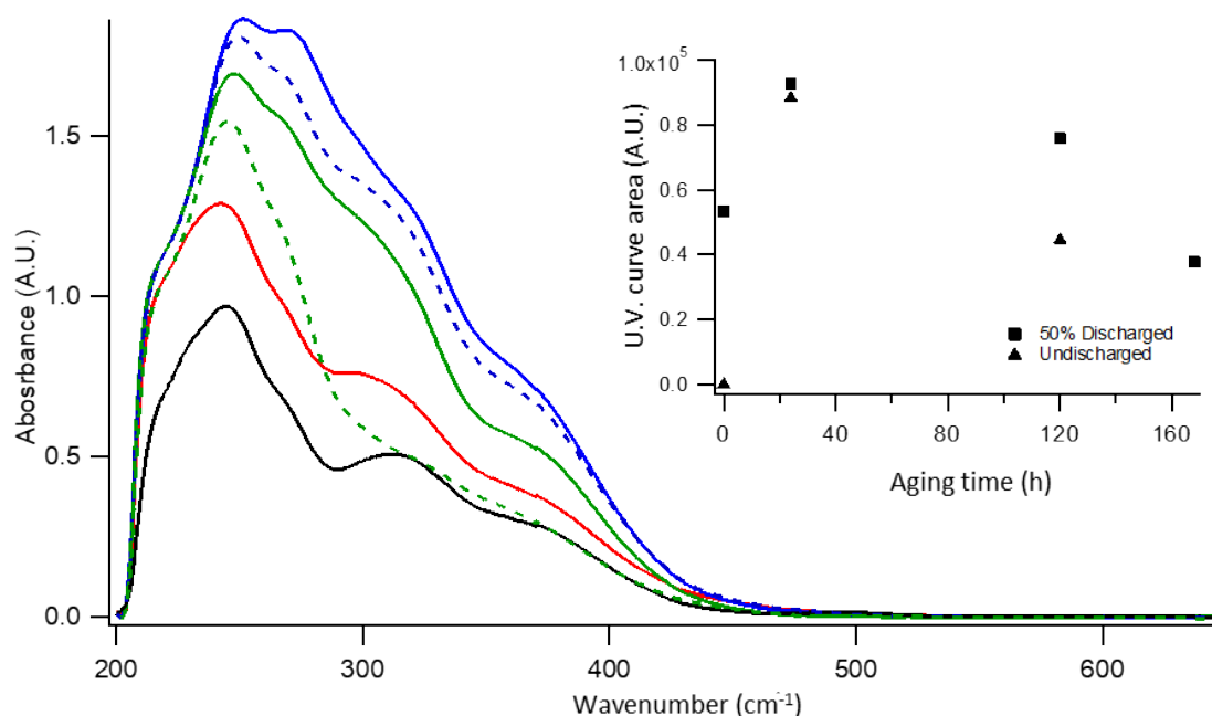
Fig. 1 Background subtracted UV/VIS absorbance spectra for extracted solutions from Mg-S cells using the 0.25 M MgTFSI 2 + 0.5 M MgCl 2 DME electrolyte. — 200 mAh/g discharged cell aged 0 h. — 200 mAh/g discharged cell aged 24 h. — 200 mAh/g discharged cell aged 120 h. — 200 mAh/g discharged cell aged 168 h. - - Undischarged cell aged 24 h. - - Undischarged cell aged 120 h. Inset shows total area under the spectra curves.
