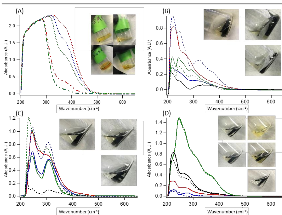
Fig. 4 UV/VIS spectra for (A) Synthesized magnesium polysulfides. ..... 0.2 M sulfur aged 0 h. ..... 0.2 M sulfur aged 24 h. ..... 0.2 M sulfur aged 72 h. - - - 0.05 M sulfur aged 0 h. - - - 0.05 M sulfur aged 24 h. - - - 0.05 M sulfur aged 72 h. (B) 1 M MgTFSI 2 + 2 M MgCl 2 in DME. —— 200 mAh/g discharged cell aged 0 h. —— 200 mAh/g discharged cell aged 24 h. —— 200 mAh/g discharged cell aged 72 h. —— 200 mAh/g discharged cell aged 168 h. - - - Undischarged cell aged 24 h. - - - Undischarged cell aged 72 h. - - - Undischarged cell aged 168 h. (C) 0.35 M Mg – 1:2 MgHMDS 2 :AlCl 3 . (D) 0.5 M Mg-FPB in DEG. Insets are photos of selected solutions analyzed by UV/VIS, black material in the photos are the extracted cathodes. Inset (A) Top left = 0.05 M solution as prepared. Top right = 0.05 M solution 72 h aged. Bottom left = 0.2 M solution as prepared. Bottom right = 0.05 M solution 72 h aged. Inset (B/C) Top left = 200 mAh/g discharged immediate analysis. Top right = undischarged 24 h aged. Bottom = reference solution for background subtraction. Inset (D) Top left = 200 mAh/g discharge 24 h aged. Top right = 200 mAh/g discharge 72 h aged. Middle left = undischarged 24 h aged. Middle right = undischarged 72 h aged. Bottom = reference solution for background subtraction.
