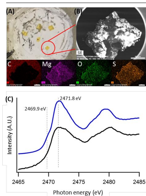
Fig. 2 (A) Photo of separator recovered from 200 mAh/g discharged cell, 168 h aged. (B) SEM image of highlighted deposit with accompanying EDX. All scale bars are 300 \mu m. (C) S K-edge XAS spectra for Mg_xS_y solid and for elemental sulfur.
