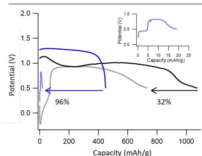
Fig. 5 1 st cycle discharge capacity for Mg-S cells at current rate of 0.1C. — 0 h aged 0.5 M Mg-FPB in DEG. — 168 h aged 0.5 M Mg-FPB in DEG. — 0 h aged 0.25 M MgTFSI_2 + 0.5 M MgCl_2 in DME. — 168 h aged 0.25 M MgTFSI_2 + 0.5 M MgCl_2 in DME. Inset shows the 168 h aged MgTFSI_2/MgCl_2 potential curve, enlarged for clarity.
