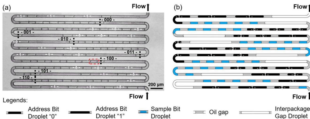
Figure 6. A proof-of-concept protocol for acoustofluidic droplet coding. (a) Micrograph and (b) schematic of the encoded droplet array. Herein, droplets are dispensed successively in end-to-end droplet packages. Each package consists of a large droplet, three droplets with regulated sizes, and five small droplets of monodispersed size, which work as an interpackage gap to denote the start of a droplet package, address bits to give the binary address code of the package by volume, and droplet samples, respectively. Thus, each droplet sample in this sequence is assigned to a unique identifier code with an address code of the package it belongs to and its sequence number in this package. For example, as shown by the dashed red box, the droplet is assigned to an identifier 011-5, which represents the 5 th droplet in the package with an address code 011. The capacity of this coding approach can be greatly expanded by using more droplets for the address bit or by increasing the number of sample droplets in one package.
