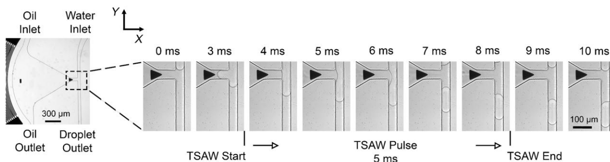
Figure 2. Micrographs of acoustofluidic droplet dispensing process. The oil flow was jetted from the chamber under the effect of TSAWs, which cuts the water flow off to form a droplet downstream of the T-junction. The flow rates of water and oil are 4.5 \mu\text{L min}^{-1} and 5 \mu\text{L min}^{-1} , respectively. The duration of the TSAW pulse is 5 ms. The gap period between adjacent pulses is 5 ms.
