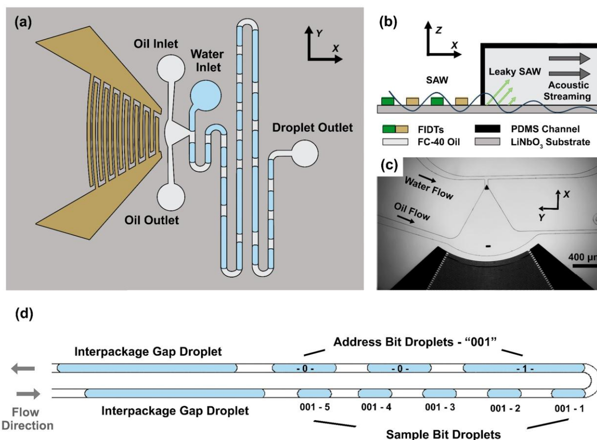
Figure 1. Schematic of the acoustofluidic droplet dispensing and coding platform. (a) Oil in the chamber of a circular sector shape is jetted via the orifice upon the acoustic attenuation of the focused surface acoustic waves (SAWs). The oil jet cuts the continuous water flow to form dispersed droplets which flow downstream the microchannel. The size of droplets can be regulated in real-time by tuning the gap period between adjacent SAW pulses. (b) The SAWs generated by the focused interdigital transducers (FIDTs) leak at the substrate-oil interface and induce acoustic streaming in the chamber. (c) Micrograph of the acoustofluidic droplet dispensing structure. The orifice locates at the focal point of the FIDTs (shown as the triangular alignment mark in this micrograph). (d) Schematic of a droplet package in (a). Droplets are dispensed successively in end-to-end droplet packages. As a protocol, each package consists of an “Interpackage Gap Droplet” (a large droplet) to indicate the beginning of a package, a 3-bit “Address Bit Droplets” of the package (three droplets with regulated sizes) to present the binary address of the package by volume, and five “Sample Bit Droplets” with consistent volume. Based on this setup, each droplet sample is assigned to a specific identification number consisting of a package address and a sequence number in this package. The five droplet samples here are represented by identification numbers “001-1”, “001-2”, ..., “001-5”, respectively.
