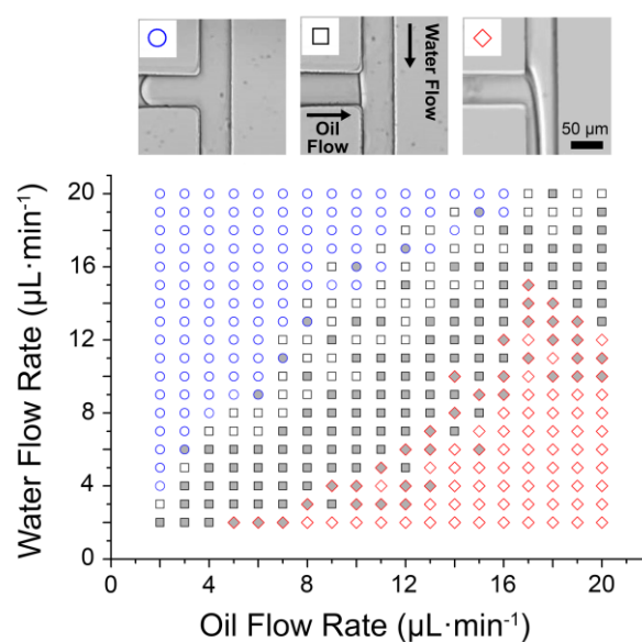
Figure 3. Influence of flow rates on the dispensing stability. When the flow rates of water and oil are balanced, the interface at the orifice is stable and two streams flow via corresponding paths (black square). If the flow rate of the oil stream becomes large enough, it will be pushed out through the orifice into the water channel (red diamond). When the water flow rate is too large to maintain the stable water-oil interface, the water flows into the oil chamber (blue circle). Combinations of flow rates suitable for the dispensing process actuated by 5 ms width TSAW at a frequency of 100 Hz is denoted by the grey fillings. The scale bar is
