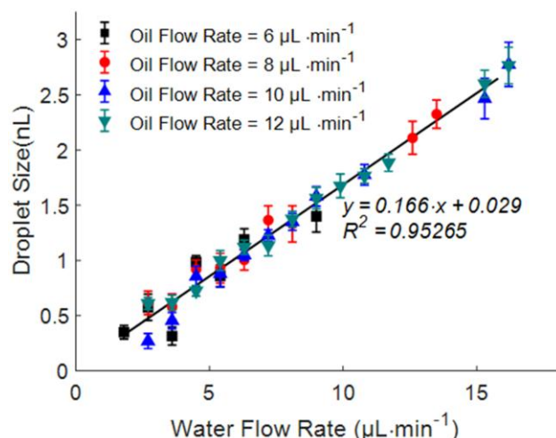
Figure 4. Effect of the flow rate on the acoustofluidic droplet dispensing process. In our design, the dispersed droplet size is proportional to the water flow rate but independent of the oil flow rate. Each period of the acoustic pulse consists of a 5 ms TSAW pulse and a 5 ms rest period. Each point in this figure is averaged over 5 tests,
