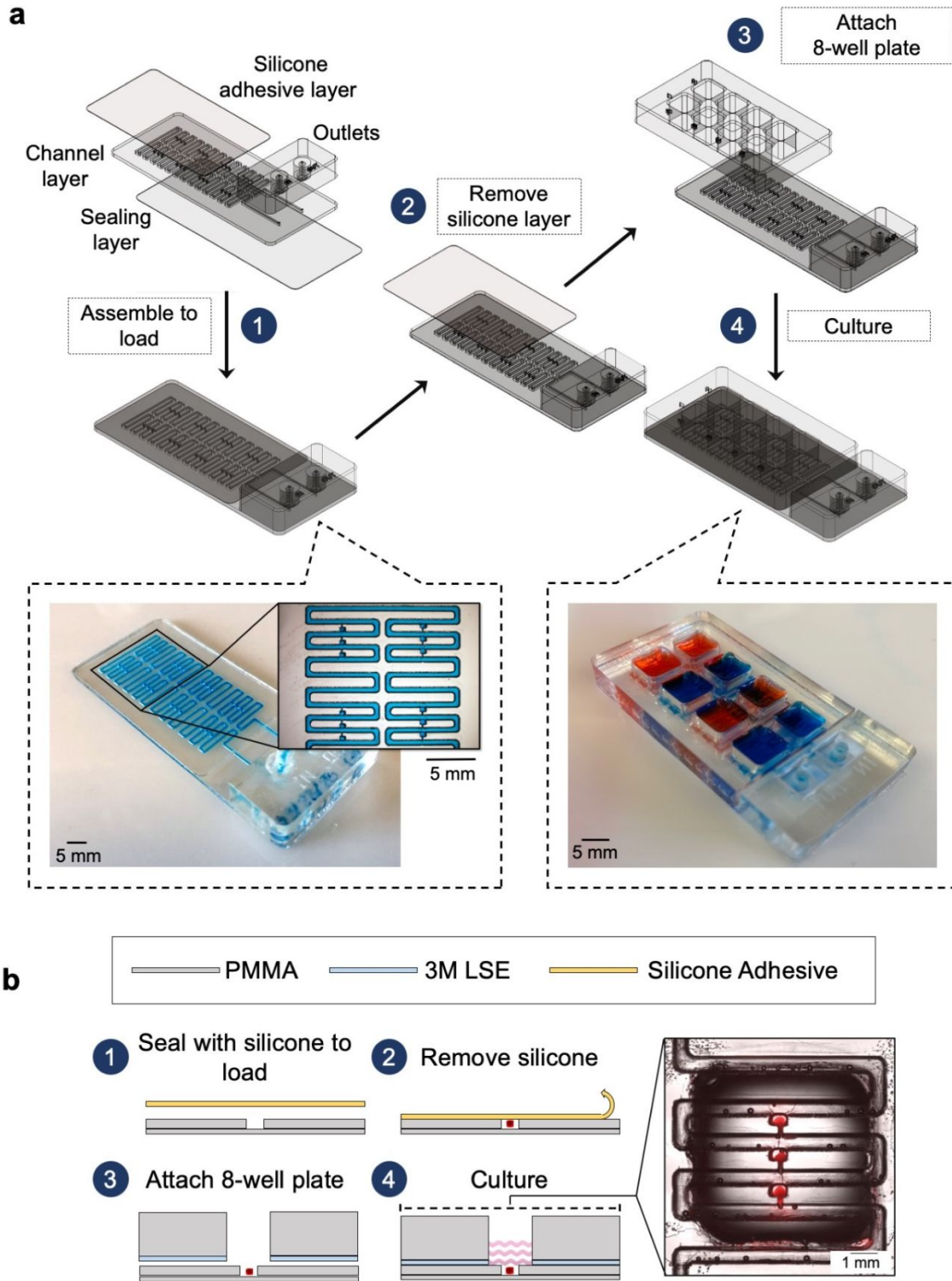
Fig. 5. Microfluidic device design and operation. a) Multistage design of the microfluidic device, with a loading stage (1-2) and a culture stage (3-4). 3D renderings of device components, as well as micrographs of a device ready for loading (filled with blue dye) and of a device ready for culture (wells filled with red and blue dyes). (b) Cross-sectional view of the same multi-step operational procedure
