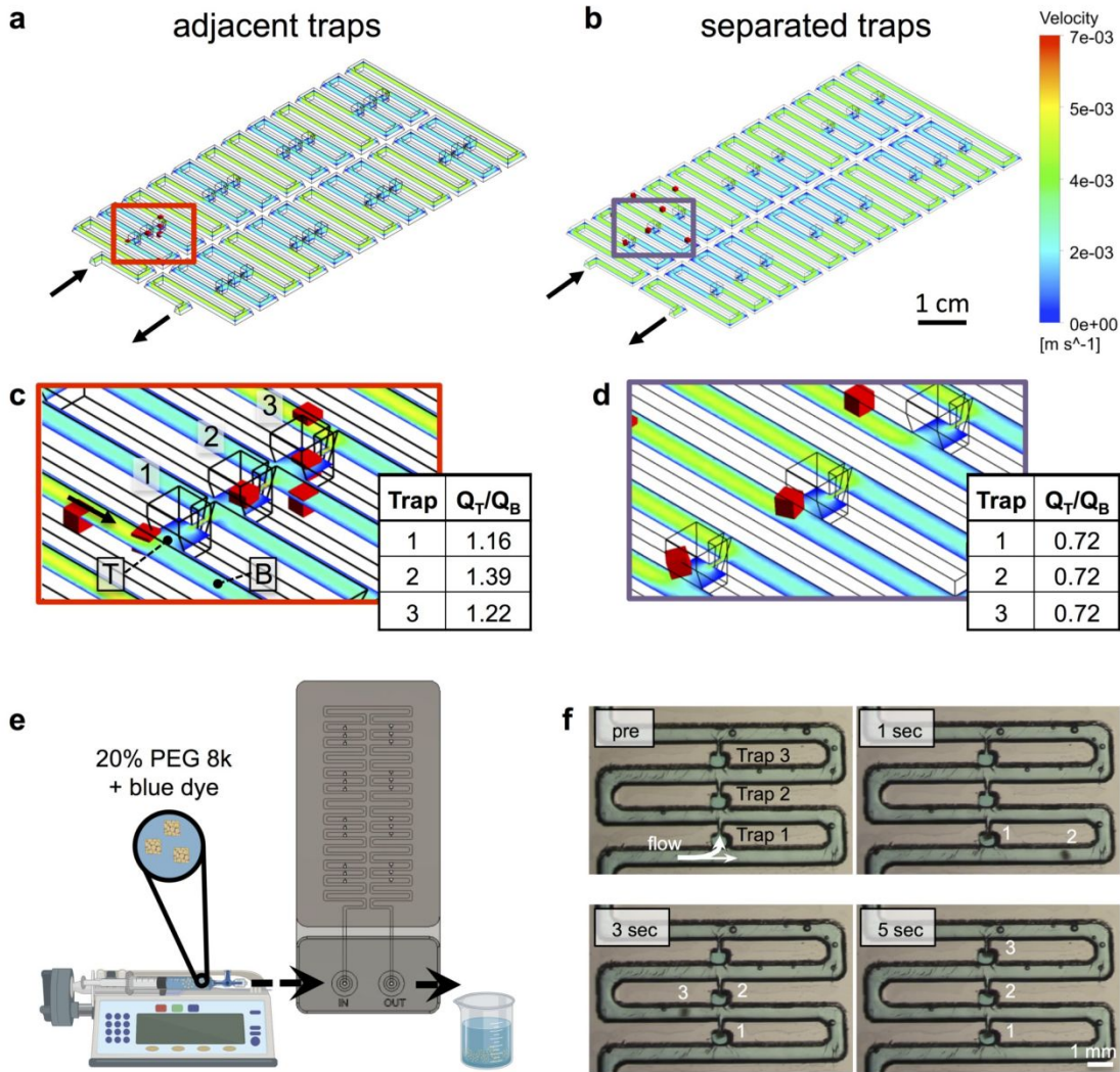
Fig. 6. Finite volume modeling and cuboid loading into the microfluidic device. (a,b) 3D schematics of the microfluidic device with adjacent traps (a) and version with separated traps (b), showing a 2D cross-section of the 3D velocity profile performed with Ansys Fluent (point particles in red). First well (three traps) outlined with a box. (c,d) Close-up views of the first well region with locations at which flow was measured in a plane perpendicular to flow indicated for the trap (T) and for the bypass channel (B). Flow (Q) ratios are given for each trap. (e) Experimental setup. (g) Still images of device loading with fixed U87 cuboids (labeled 1,2,3) in a 20% PEG solution with blue dye. Full movie in Electronic Supplementary Information. The flow rate was 20 mL/h.
