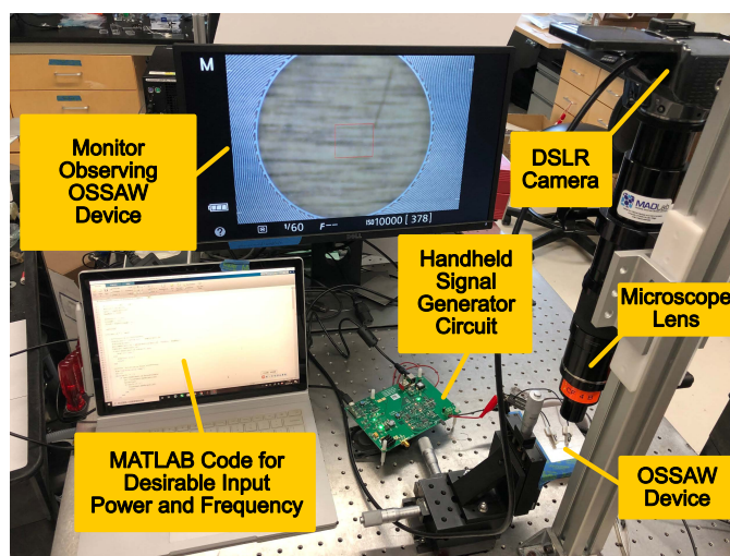
Fig. 7 An example of the SAW board in use for SAW-induced particle separation.
