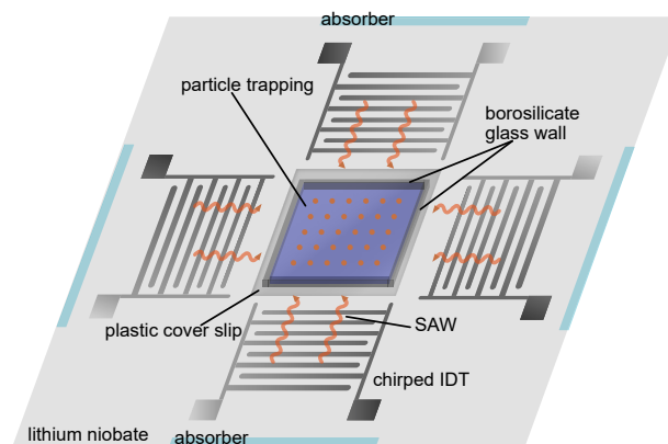
Fig. 12 A schematic of the 2D alignment device. Four-way chirped IDTs create a series of regular pressure nodes where particles are entrapped.
