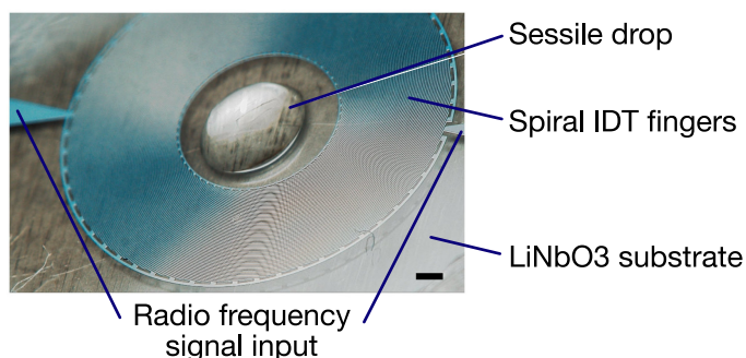
Fig. 10 A 60-MHz OSSAW device with a microliter sessile drop in the inner circular region, showing the fingers and electrode connection to produce a suitable spiral SAW. Scale bar: 0.5 mm.
