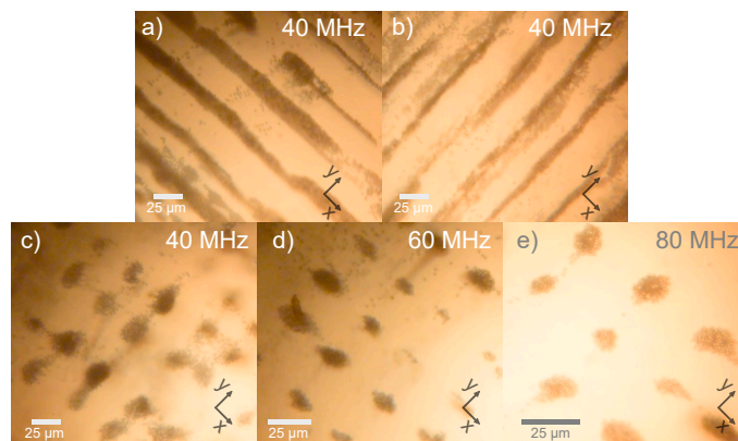
Fig. 13 When only two IDTs are actuated, particles are aligned in lines along (a) the x direction or (b) the y direction depending on which pair of IDTs are actuated (in this case at 40.2 MHz). When 4 IDTs are actuated at the same time, particles are aligned in an array with different separations at corresponding frequencies: (c) 40 MHz, (d) 60 MHz and (e) 80 MHz. Scale bar: 25\ \mu\text{m} .
