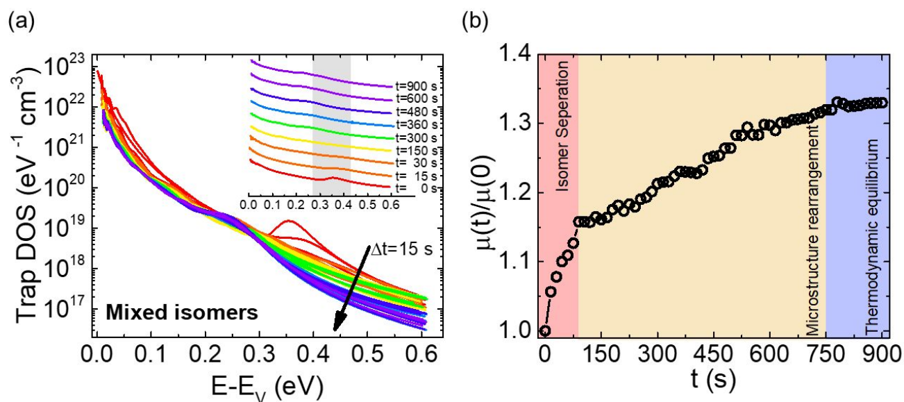
Fig. 3 a) Evolution of the trap DOS spectrum of a device with mixed isomer crystallites. The DOS curves are plotted as a function of energy from the valence band edge and clearly illustrate the annihilation of the peak at 0.36 eV. The DOS was evaluated every 15 s during exposure to ethanol vapor and the time evolution of the spectrum from t = 0 s (red) to t = 900 s (violet) is shown. Inset includes a subset of the trap DOS spectra offset for clarity. b) Time evolution of the charge carrier mobility during the period of solvent exposure. The value is normalized to the initial value obtained before exposure to ethanol.
