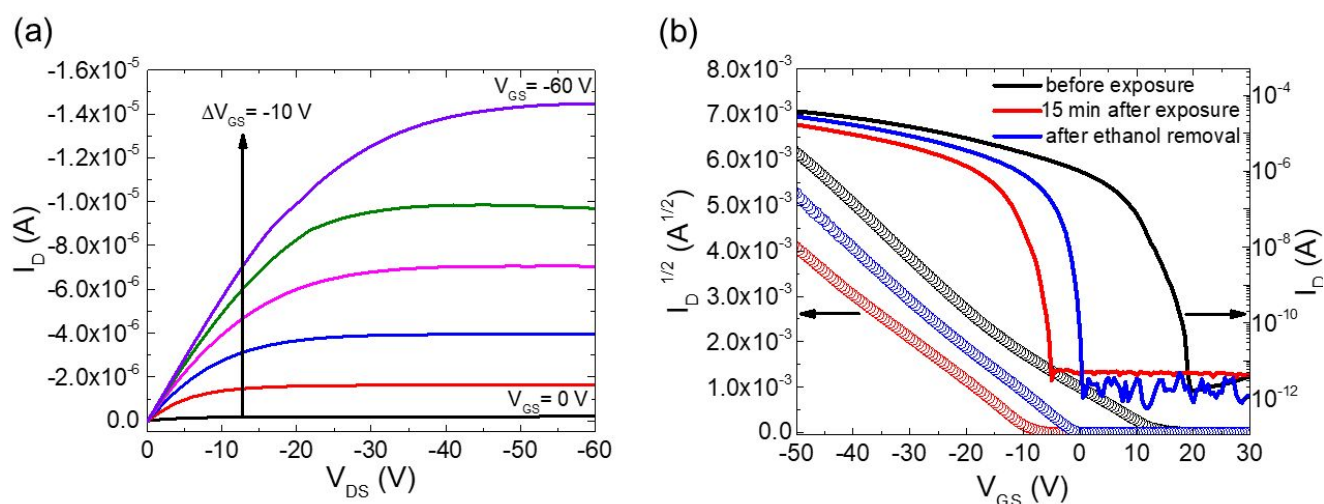
Fig. 2 Current-voltage characteristics of a diF TES ADT OFET device exposed to solvent vapor. a) I_D vs V_{DS} plot at various fixed V_{GS} (0 V to -60 V in -10 V increments) measured before exposure to the ethanol vapor. b) I_D vs V_{GS} plot at V_{DS} = -60 V obtained before exposure to ethanol vapor (black), after 15 min of exposure (red) and after removal of ethanol from the measurement chamber (blue). The left and right axes show the square root and logarithm of the drain current, respectively.
