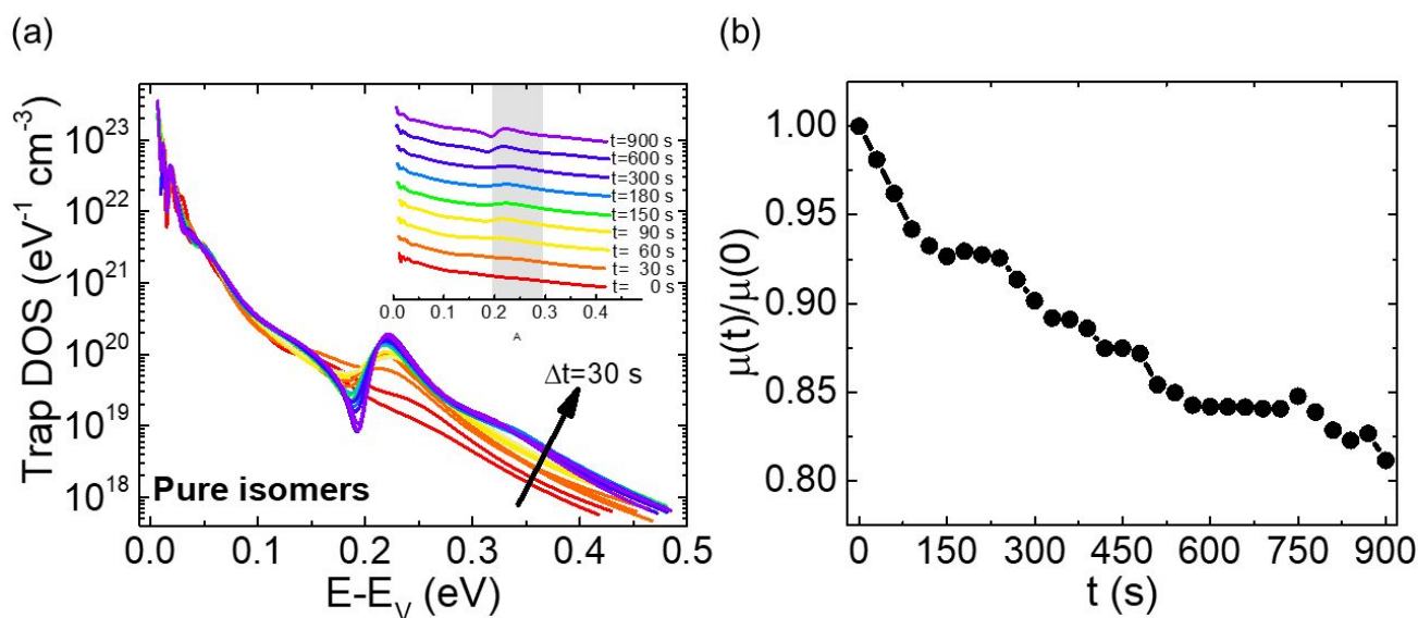
Fig. 5 a) Evolution of the trap DOS spectrum of a device consisting of pure isomers. The DOS curves are plotted as a function of energy from the valence band edge and clearly illustrate the generation of a peak at 0.22 eV. The DOS was evaluated every 30 s during exposure to ethanol vapor and the time evolution of the spectrum from t = 0 s (red) to t = 900 s (violet) is shown. Inset shows a subset of the trap DOS spectra offset for clarity. b) Time evolution of the charge carrier mobility during the period of solvent exposure. The value is normalized to the initial value obtained before exposure to ethanol.
