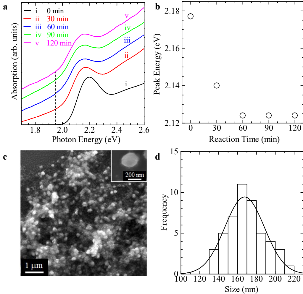
Fig. 5 Observation of quantum resonance in CdTe QD assemblies. (a) Dependence of the absorption (extinction) spectra on the reaction time. Here, 0 min represents the absorption spectrum of the CdTe QD solution and 30–120 min represent the extinction spectra of the CdTe QD assemblies. (b) Dependence of the extinction peak energy on the reaction time. (c) SEM image of the CdTe QD assemblies. The inset shows magnified SEM image. (d) Size histogram of the CdTe QD assemblies. The solid curve represents a gaussian fitting function with an average size of 173 nm and a standard deviation of 22 nm.
