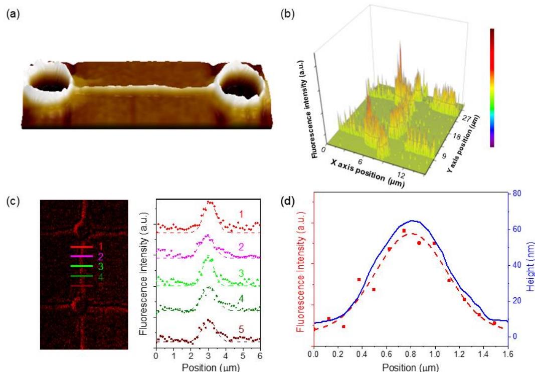
Fig. 3 Utilization of polymer wrinkles as nanofluidic channels. (a) 3D AFM image of wrinkle via analysis. (b) Position-dependent fluorescence intensity map showing the distribution of the fluorescent dye along the linear and circular wrinkles. (c) Fluorescence image and the cross-sectional profiles of the fluorescence intensity at five locations. (d) Overlap of fluorescence intensity (red dots and dashed line) and height profile of the wrinkle (blue line).
