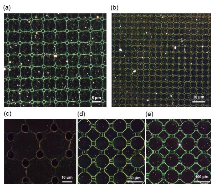
Fig. 2 Dark-field OM images of diverse wrinkle structures. (a–c) Wrinkles with (a, b) square and (c) honeycomb lattice patterns. The D_h /spacing are (a, b) 3/6 \mu\text{m} and (c) 10/10 \mu\text{m} , respectively. (d, e) Multiplets of wrinkles from the square lattice patterns for a D_h of (d) 40 and (e) 80 \mu\text{m} with an identical spacing between neighboring holes of \sim 10 \mu\text{m} .
