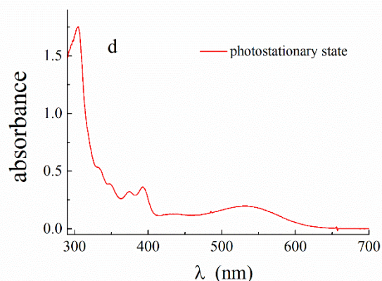
Fig. 8. a) Quantitative absorption spectra of the TTT (peak 1, see text below) forms produced upon irradiation of the CN-Ph-R molecules, along with that of the TT obtained for the unsubstituted CN-Ph-H; the two TTT (peak 1) and CTT (peak 2, see text) coloured isomers produced upon irradiation of CN-Ph-N(pyridyl) 2 (b) and CN-Ph-OMe (c); d) absorption spectrum of the photostationary state mixture obtained upon irradiation of CN-Ph-N(methyl) 2 .
