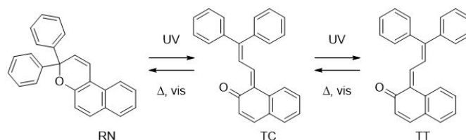
Scheme 1 Mechanism of the photochromic reaction of 3,3-diphenyl-3H-naphtho[2,1-b]pyran.
