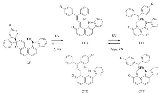
Scheme 6 Mechanism proposed for the photochromic reaction of the CN-Ph-R chromenes, showing the initial closed form (CF), and the main coloured transoid- cis (CTC and TTC) and transoid- trans (CTT and TTT) isomers.
