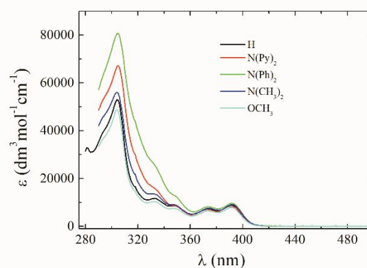
Fig. 3 Quantitative absorption spectra of the five N-phenyl carbazole benzopyrans in toluene.
