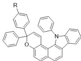
Fig. 1 Molecular structure of the N-phenyl carbazole benzopyrans (CN-Ph-R).
