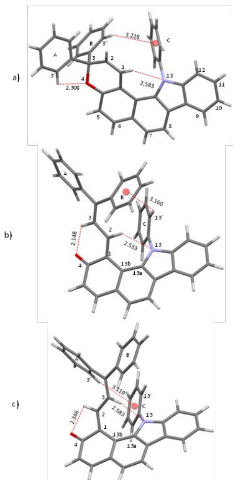
Fig. 2 a) X-ray structure of CN-Ph-H; Optimized structures at CAM-B3LYP of b) TC form and c) TT form.
