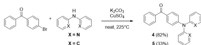
Scheme 3 Preparation of 2,2'-dipyridylamine- and 2,2'-diphenylamine-benzophenones.
