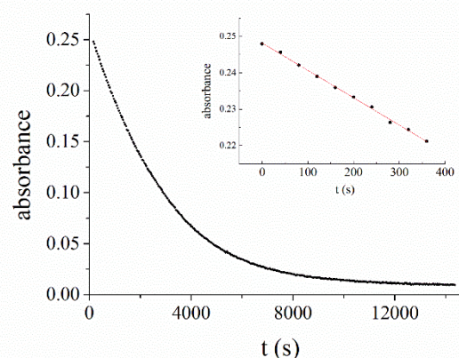
Fig. 6 Kinetics of visible photobleaching ( \lambda_{\text{irr.}} = 435\text{ nm} ) of CN-Ph-H in toluene, monitored at 500 nm. Inset: linear interpolation of the first points of the decay (see below).
