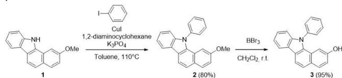
Scheme 2 Preparation of 11-phenyl-11H-benzo[a]carbazol-2-ol.
