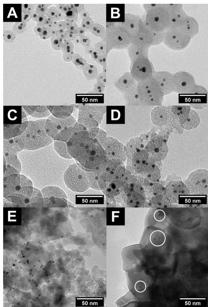
Figure 1. TEM micrographs of Au@SiO 2 CSNPs and control catalysts. (A) CSNPs before the second addition of TEOS and subsequent etching phase. (B) CSNPs pre-calcination. (C) CSNPs post-calcination. (D) CSNPs after two sequential 1-hour benzyl alcohol oxidation reactions with no added base. (E) Silica-supported nanoparticles. (F) Ceria-supported nanoparticles.
