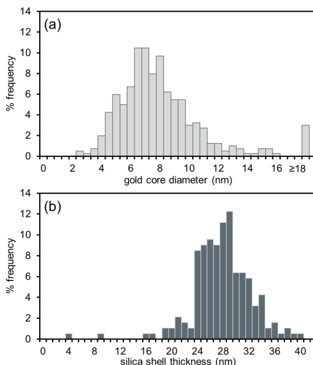
Figure 2. (a) Gold core diameter histogram ( n = 402 ) of post-calcination Au@SiO 2 CSNPs. d = 8.0 \pm 3.9 nm (b) Silica shell thickness histogram ( n = 188 ) of the same sample. T = 27.4 \pm 4.6 nm.
