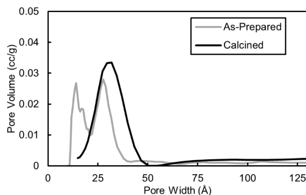
Figure 4. Pore size distribution of as-synthesized and calcined Au@SiO 2 core-shell nanoparticles.
