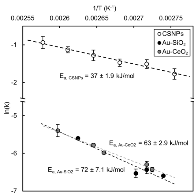
Figure 7. Catalyzed benzyl alcohol oxidation Arrhenius plot for CSNPs and control catalysts, in the absence of a base.
