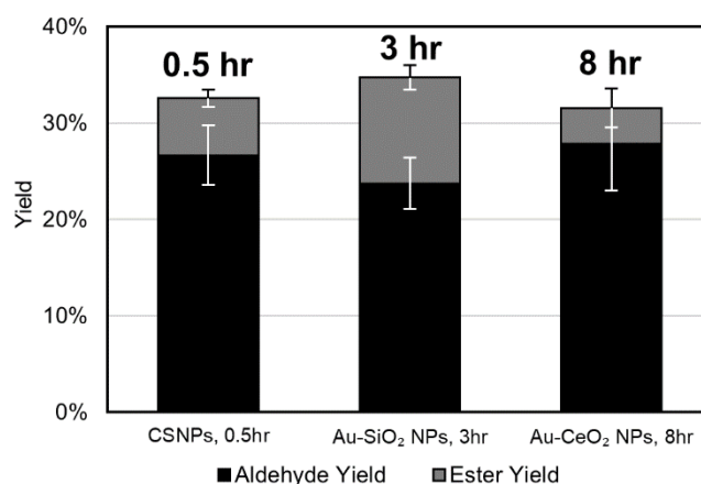
Figure 6. Selectivity of benzyl alcohol oxidation catalyzed by CSNPs and supported Au nanoparticles, in the presence of K 2 CO 3 , reacted for decreasing times to match conversion on Ceria-supported NPs.
