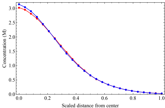
Fig. 4 Ion concentration verses scaled z position for small (red) and large (blue) systems.
