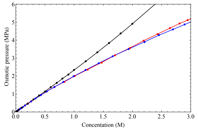
Fig. 5 Experimental data (black) vs simulation data for small (red) and large (blue) systems using default OPLS parameters for \text{Na}^+ and \text{Cl}^- .
