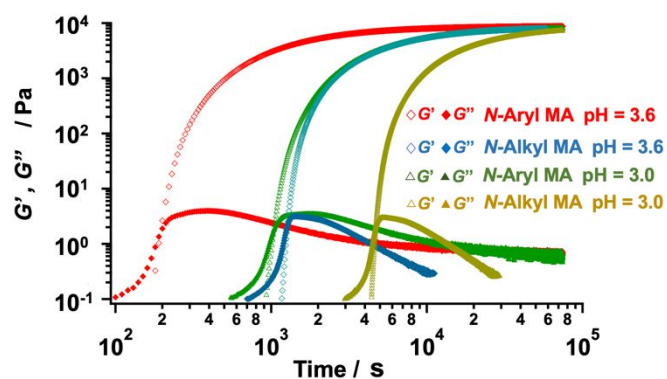
Figure 5. Viscoelastic properties of the gel samples (red and green: N -aryl MA; blue and yellow: N -alkyl MA) during the gelation process (6 wt% in a buffer; pH = 3.0 and pH = 3.6).
