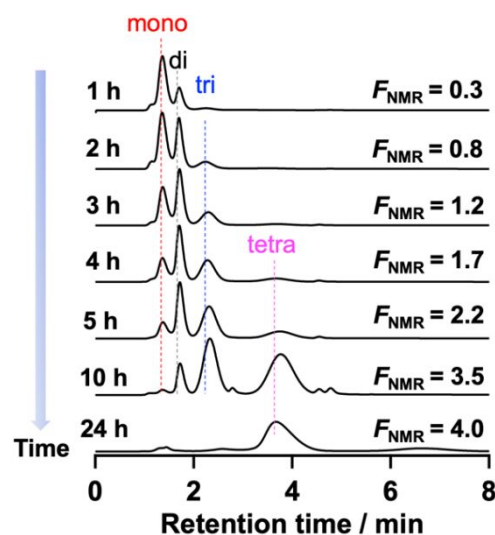
Figure 4. Change in the HPLC profiles during the modification reaction (eluent: acetonitrile/water, 45/55, v/v; flow rate: 1.0 \text{ mL min}^{-1} , UV detector).
