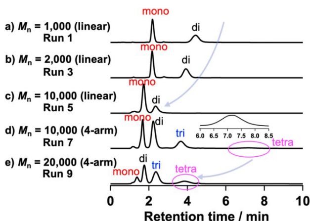
Figure 3. HPLC profiles of modified PEGs with different molar masses and functionalities (eluent: acetonitrile/water, 45/55, v/v; flow rate: 1.0 \text{ mL min}^{-1} on a C18 column at 30^\circ \text{C} using a UV detector).
