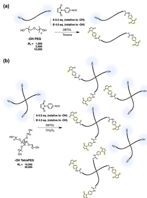
Scheme 1. Synthesis of N -aryl MA PEGs. a) Reaction with hydroxy-terminated PEGs. b) Reaction with hydroxy-terminated TetraPEGs. Table 1 Synthesis conditions and structural parameters of the N -aryl MA PEGs and N -aryl MA TetraPEGs. F_{\text{NMR}} denotes the average functionality estimated using ^1\text{H} NMR.
