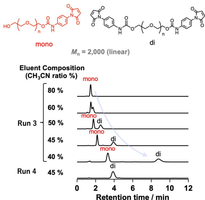
Figure 2. HPLC profiles of modified PEGs ( M_n = 2,000 ) with different numbers of N -aryl MA groups (Runs 3 and 4 in Table 1) using different eluent compositions (values shown are the vol% of acetonitrile in water) at a flow rate of 1.0 \text{ mL min}^{-1} on a C18 column at 30^\circ \text{C} using a UV detector.
