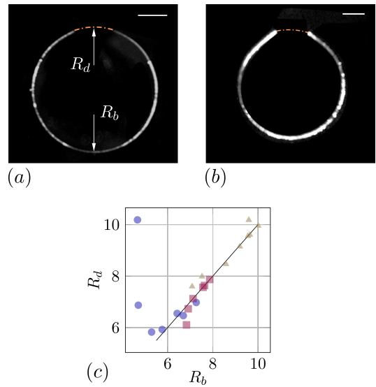
Fig. 6 (a, b) Fluorescence images showing shape of filament encapsulating the droplet for a filament of diameter d = 90 \mu\text{m} , 170 \mu\text{m} and a droplet of size w = 7.5 \text{mm} , 2.3 \text{mm} with droplet-interface shown as dashed-line. The scale bar is 3.7 \text{mm} . (c) Radius of curvature of the buckled zone in the filament, R_b vs the radius of curvature of free interface of the droplet, R_d in mm. Solid line indicates R_b = R_d . We consider three different filament diameters d = 80 \mu\text{m} ( \triangle ), 90 \mu\text{m} ( \square ), 170 \mu\text{m} ( \circ ).
