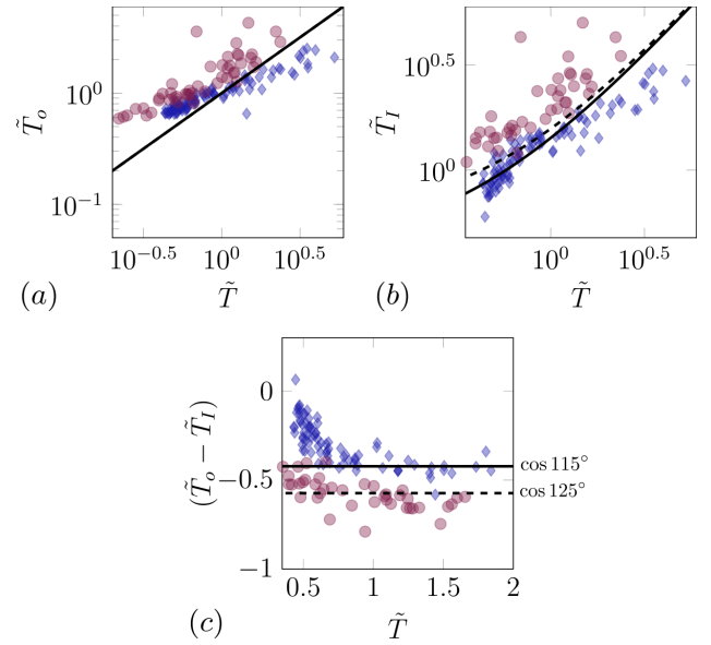
Fig. 4 (a) Non-dimensional applied tension \tilde{T}_o , (b) tension in the portion of the filament wet by the droplet \tilde{T}_I , and (c) the difference between these tension values, (\tilde{T}_o - \tilde{T}_I) evaluated by using angles \vartheta, \phi measured from experiments (using eqn. 5) as functions of the applied tension, \tilde{T} measured using soft-beam displacement. \circ correspond to filament diameter 205\mu\text{m} and \diamond to diameter 77\mu\text{m} for different droplet sizes. The solid and dashed lines respectively indicate theoretical predictions from eqn. 6.
