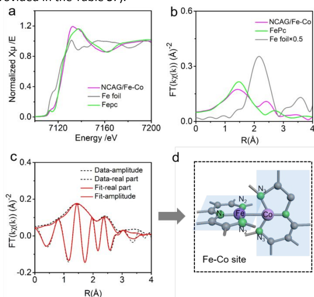
Figure 3. (a) Fe K-edge XANES and (b) EXAFS of NCAG/Fe-Co, Fe foil and FePc. (c) Fe K-edge EXFAS of NCAG/Fe-Co and the fitting curve. (d) Schematic illustration of the structure of the Fe-Co dual metal sites in NCAG/Fe-Co.
