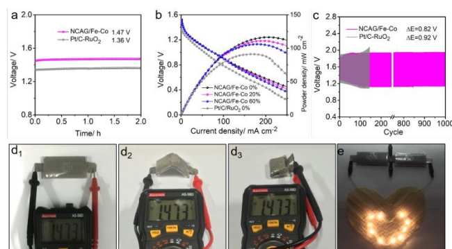
Figure 5. (a) Open circuit voltage of a solid Zn-air battery with NCAG/Fe-Co as the oxygen electrode catalysts, in comparison to that
