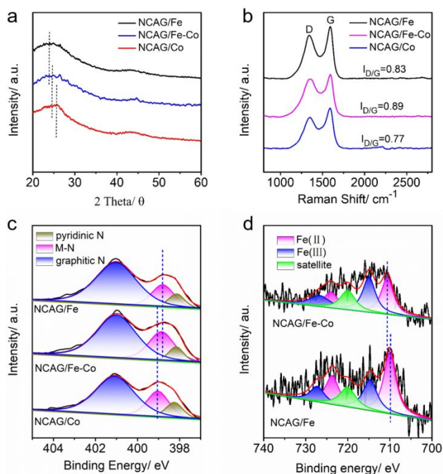
Figure 2. (a) XRD patterns of NCAG/Fe-Co, NCAG/Fe, NCAG/Co. (b) Raman spectra of NCAG/Fe-Co, NCAG/Fe, NCAG/Co. (c) XPS spectra of the N 1s electrons in NCAG/Fe-Co, NCAG/Fe, NCAG/Co. (d) High-resolution XPS scan of the Fe 2P electrons of NCAG/Fe-Co, NCAG/Fe.
