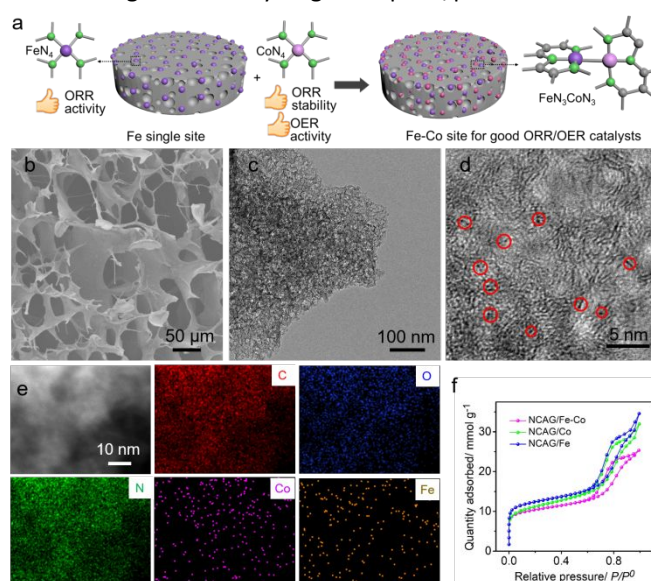
Figure 1. (a) Schematic illustration of the combination of Fe and Co single atom catalysts into Fe-Co dual metal-doped carbon aerogel. (b) SEM image of the freeze-dried G Si-Zn /Fe@CoPM hydrogel. (c) TEM image of the NCAG/Fe-Co aerogel. (d) HRTEM image of the NCAG/Fe-Co aerogel. The red circles indicate metal clusters. (e) HAADF-STEM image and elemental maps of NCAG/Fe-Co. (f) Nitrogen adsorption-desorption isotherms of NCAG/Fe-Co, NCAG/Fe, NCAG/Co.
