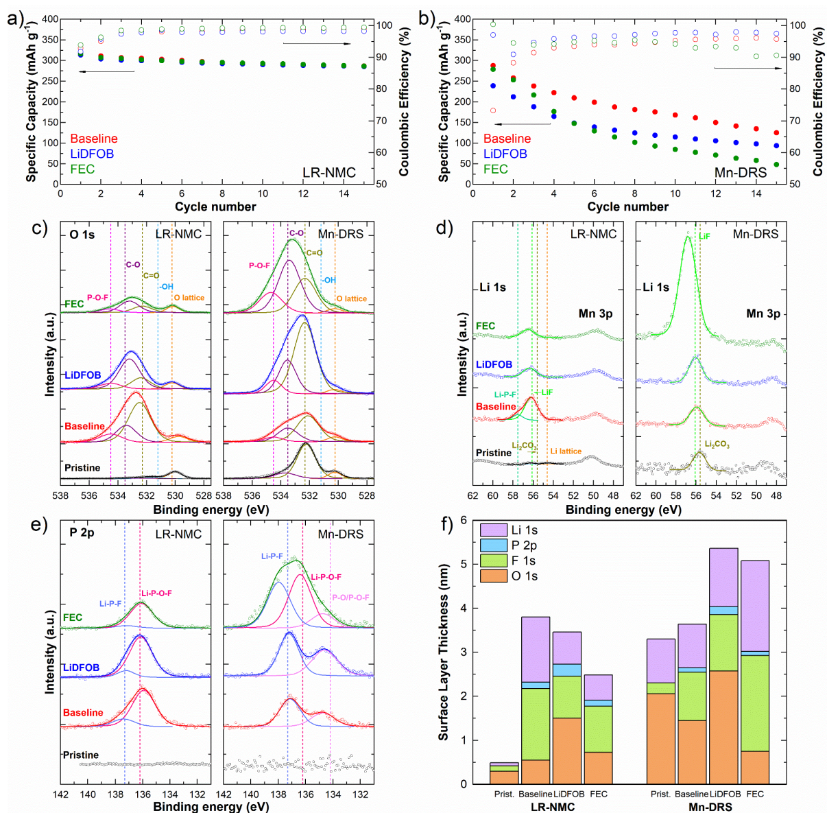
Figure 6. Cycling stability of a) \text{Li}[\text{Li}_{0.144}\text{Ni}_{0.136}\text{Co}_{0.136}\text{Mn}_{0.544}]\text{O}_2 (LR-NMC) and b) \text{Li}_{1.3}\text{Mn}_{0.4}\text{Nb}_{0.3}\text{O}_2 (Mn-DRS) with the 3 different electrolytes studied. XPS spectra of the c) O 1s, d) Li 1s – Mn 3p, and e) P 2p region of LR-NMC and Mn-DRS in the pristine state and after first discharge for the 3 electrolytes tested. f) Surface layer thickness calculated from the XPS spectra with elemental contribution.
