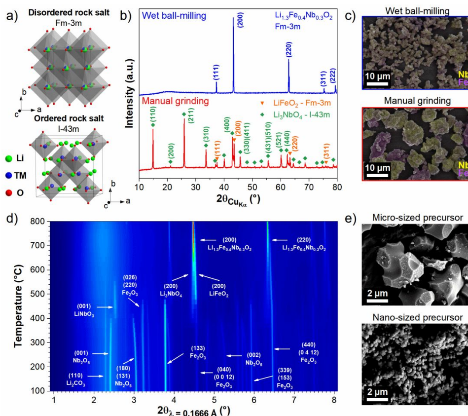
Figure 1. a) Crystal structures of disordered and ordered rock salt. Key parameters influencing the morphology and phase obtained during the solid-state synthesis of \text{Li}_{1.3}\text{Fe}_{0.4}\text{Nb}_{0.3}\text{O}_2 : b, c) Precursor mixing process, d) synthesis temperature, and e) morphology of the precursors.
