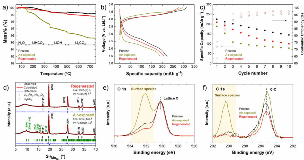
Figure 5. Study of the effect of surface contamination on the morphology-controlled sample of \text{Li}_{1.3}\text{Fe}_{0.4}\text{Nb}_{0.3}\text{O}_2 in pristine state, after 4 weeks of air exposure, and after regeneration by heat treatment: a) Thermogravimetric analysis, b) First voltage profiles, c) Cycling stability, d) Profile matching refinement of the XRD patterns, and XPS measurements of the e) O 1s and f) C 1s core regions.
