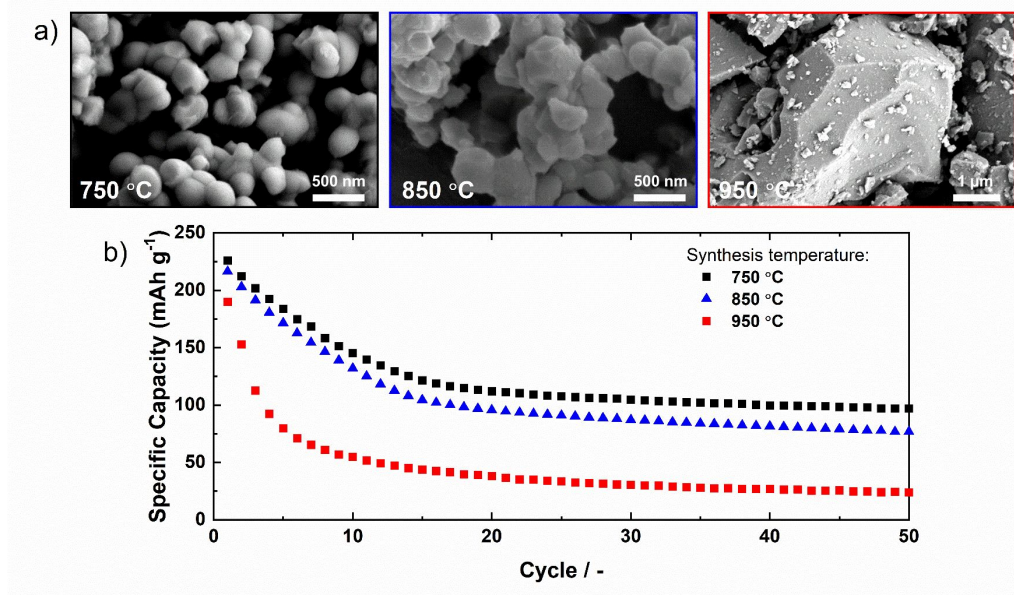
Figure 4. a) SEM images and b) cycling stability of \text{Li}_{1.3}\text{Fe}_{0.4}\text{Nb}_{0.3}\text{O}_2 synthesized at a temperature of 750 °C (black), 850 °C (blue), and 950 °C (red).
