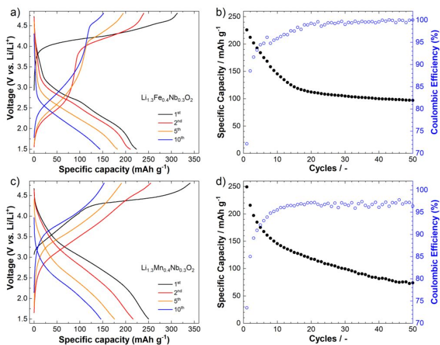
Figure 3. Voltage profile and cycling stability of morphology-controlled samples of a, b) \text{Li}_{1.3}\text{Fe}_{0.4}\text{Nb}_{0.3}\text{O}_2 and c, d) \text{Li}_{1.3}\text{Mn}_{0.4}\text{Nb}_{0.3}\text{O}_2 in the voltage range of 1.5 - 4.8 V vs. \text{Li}/\text{Li}^+ at room temperature.
