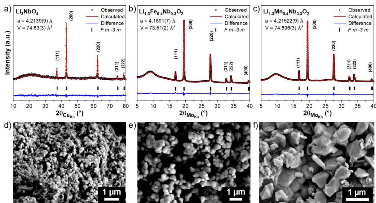
Figure 2. Rietveld refinements of the XRD patterns and associated SEM images of a, d) \text{Li}_3\text{NbO}_4 ; b, e) \text{Li}_{1.3}\text{Fe}_{0.4}\text{Nb}_{0.3}\text{O}_2 ; and c, f) \text{Li}_{1.3}\text{Mn}_{0.4}\text{Nb}_{0.3}\text{O}_2 obtained by using nano-sized precursors
