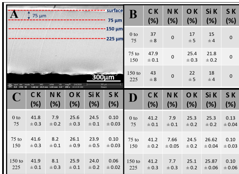
Fig. 6. PDMS-control coating with PDMS-SB-UU (A) cross-section image for analysis, (B) atomic % of non-coated, (C) atomic % of dip-coating using 2% (wt/vol) in HFIP, and (D) atomic % of dip-coating using 2% (wt/vol) in HFIP/DCM (1/1). Data are expressed as mean ± SD
