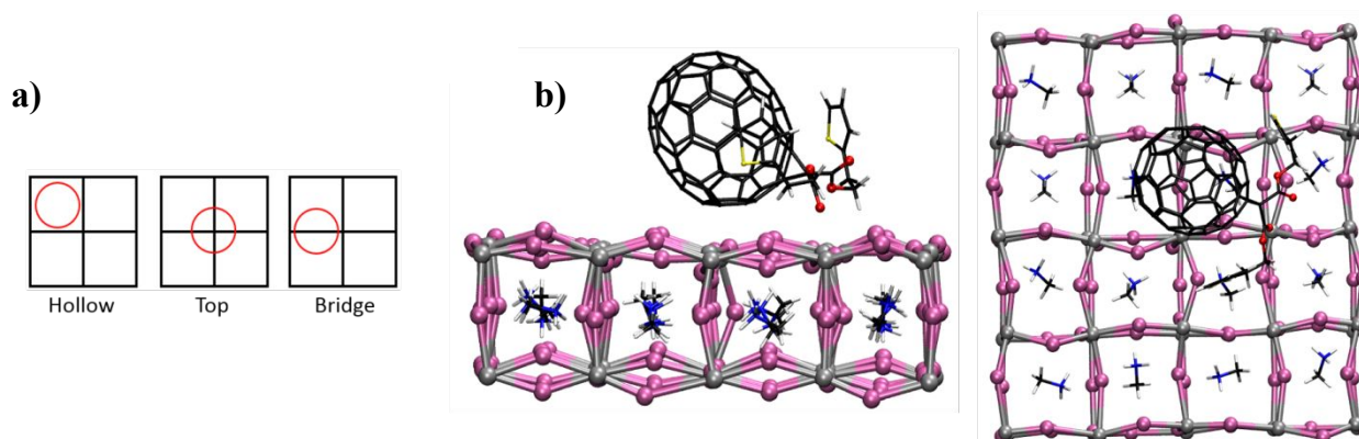
Figure 6. a) Schematic representation of three types of adsorption sites of the fullerene on the perovskite surface and b) two views of the lowest energy structures (bridge isomer) for \alpha -DTC 70 .
