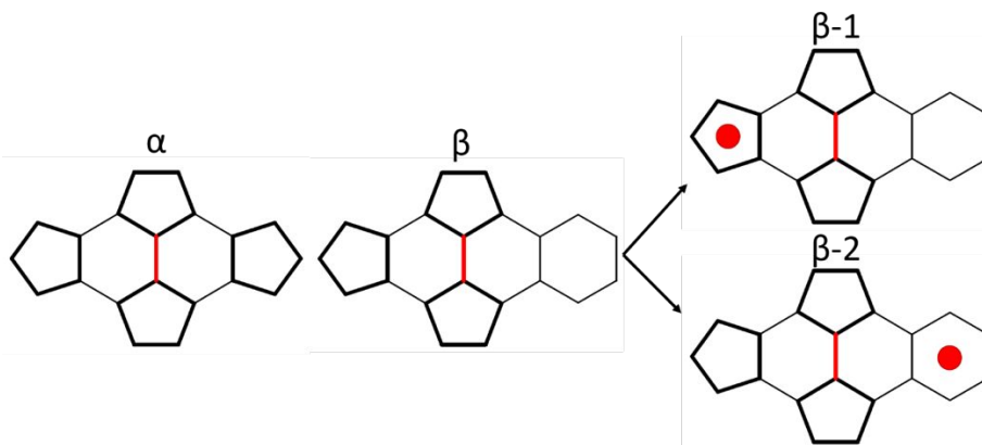
Figure 5. \alpha and \beta motifs for the [6,6] Bingel adducts of C 70 . The red line represents the addend carbon-carbon bond position on the fullerene. For a representation of \beta_1 and \beta_2 isomers see Figure S15.
