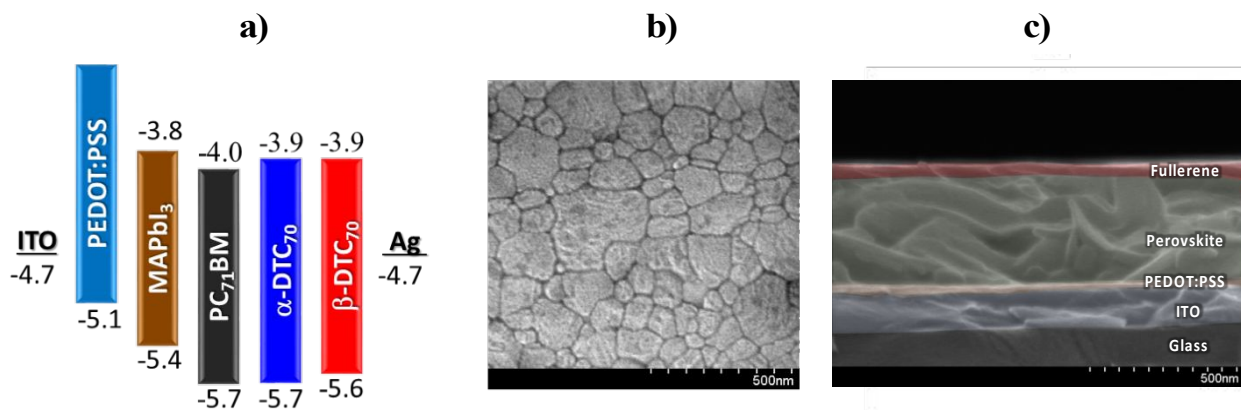
Figure 1 a) Energy level diagram, PC 71 BM values were taken from the literature, 21 b) surface SEM image of the perovskite layer and c) cross section SEM of the perovskite device.
