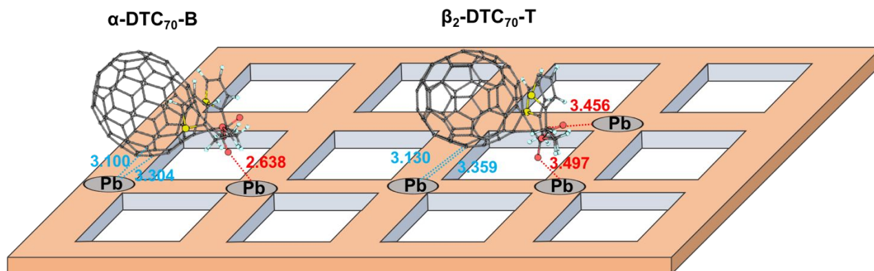
Figure 7. Schematic representation for the lowest energy \alpha -DTC 70 and \beta -DTC 70 adducts adsorbed on the MAPbI 3 surface. The values in red and cyan correspond to the shortest lead-fullerene and lead addend distances (in Å), respectively. A 3D view of the metal adduct contacts can be found in Figure S17.
