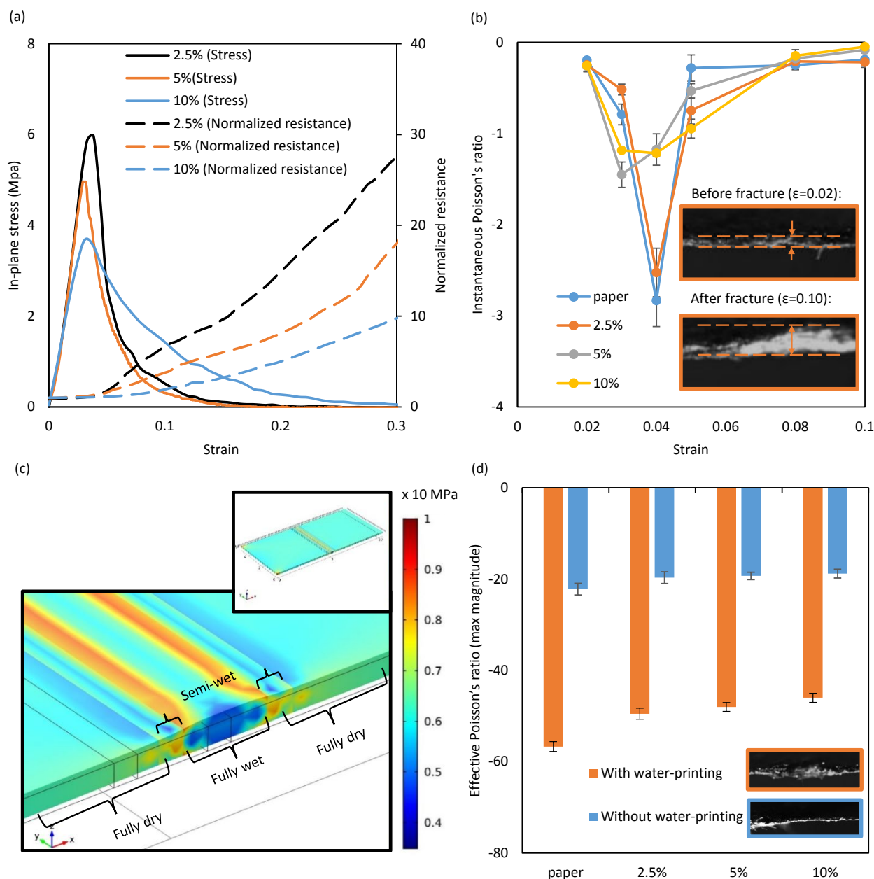
Fig. 2 (a) Stress-strain relationship coupled with normalized resistance change. (b) Instantaneous Poisson's ratios of pure paper and CPC with CNT wt% of 2.5, 5 and 10 during stretching. Inset: optical images of CPC profiles with 2.5 CNT wt % before and after fracture ( \epsilon = 0.02 and 0.10 ). The original CPC thickness is 100\ \mu\text{m} . (c) Simulation result of stress distribution for water-printed CPC under tension. (d) Maximum effective Poisson's ratios for water-printed and non-water-printed pure paper and CPC with CNT wt % of 2.5, 5, and 10. Inset: optical microscope images of fractured profiles of CPC with 10 CNT wt % with and without water-printing.
