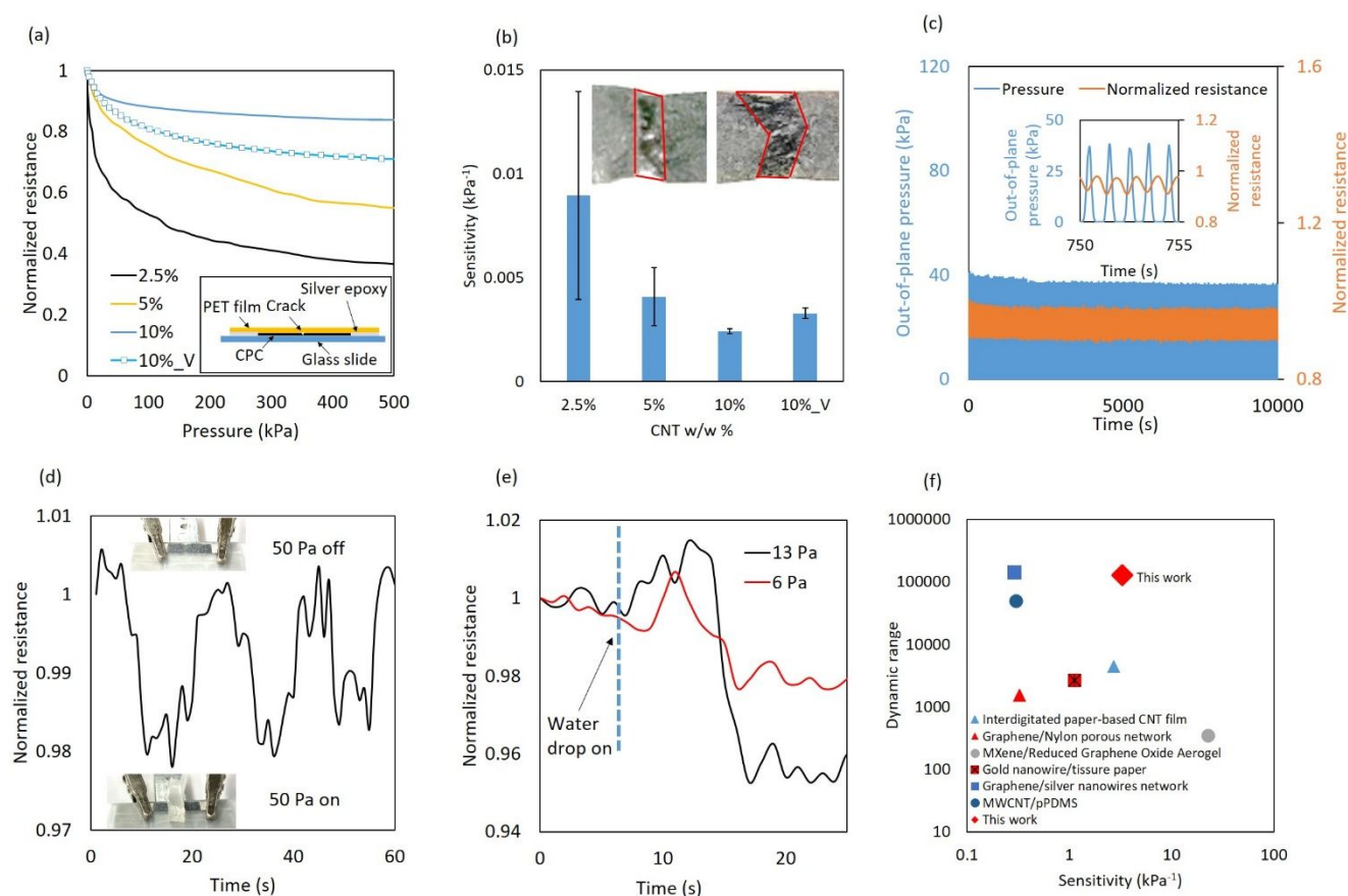
Fig. 4 Characterization of sensing performance of CPC piezoresistive sensor. (a) Normalized resistance response of CPC sensors with CNT wt % of 2.5, 5, 10, and 10 with V-shaped pattern under applied pressure from 0 ~ 500 kPa. Inset: packaging of the pressure sensor. (b) Average sensitivity of CPC sensors with CNT wt % of 2.5, 5, 10, and 10 with V-shaped pattern under applied pressure from 0 ~ 50 kPa. Inset: fractured shape induced by straight line and V-shaped water-printing. (c) Normalized resistance response of CNT-cellulose piezoresistive pressure sensor (thickness: 100 \mu\text{m} ) to cyclic loads of 0 ~ 40 kPa. Inset: closeup of normalized resistance response for 750 ~ 755 s. The CPC sensor is sealed with a polyethylene terephthalate (PET) film to avoid damaging the sensing element. (d) Cyclic detection of small pressure of 50 Pa. Inset: images of sensor surface with and without the weight block. (e) Resistance changes of the CPC sensor when detecting a small drop of water with applied pressure of 6 Pa and 13 Pa, respectively. (f) Comparison of piezoresistive sensors for their sensitivity and dynamic range. 43-48
