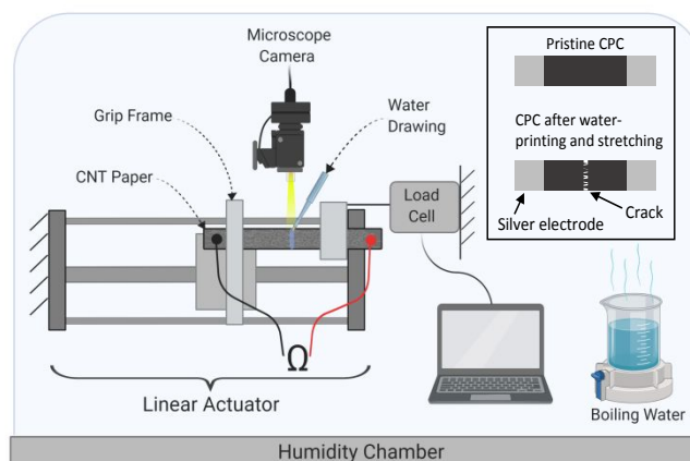
Fig. 1 Schematic describing the production of auxetic CPC by water-printing under uniaxial tension. The inset shows the CPC before and after the water-printing and stretching process.
