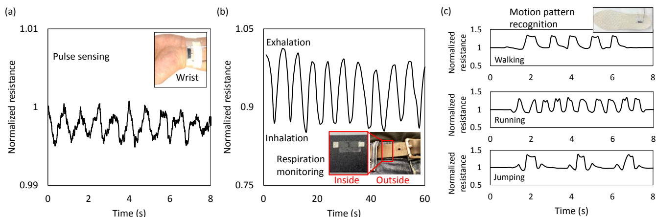
Fig. 5 Wearable sensor applications with CPC piezoresistive sensors. (a) Resistance variance of CPC pulse sensor when detecting wearer's pulse. Inset: images of the CPC pulse sensor attached to the wearer's wrist. (b) Normalized resistance of the smart belt during normal respiration. (c) Resistance changes of a foot pressure sensor at three modes of motions: walking, running, and jumping. The CPC sensor is sealed with a polyethylene terephthalate (PET) film to avoid damaging the sensing element.
